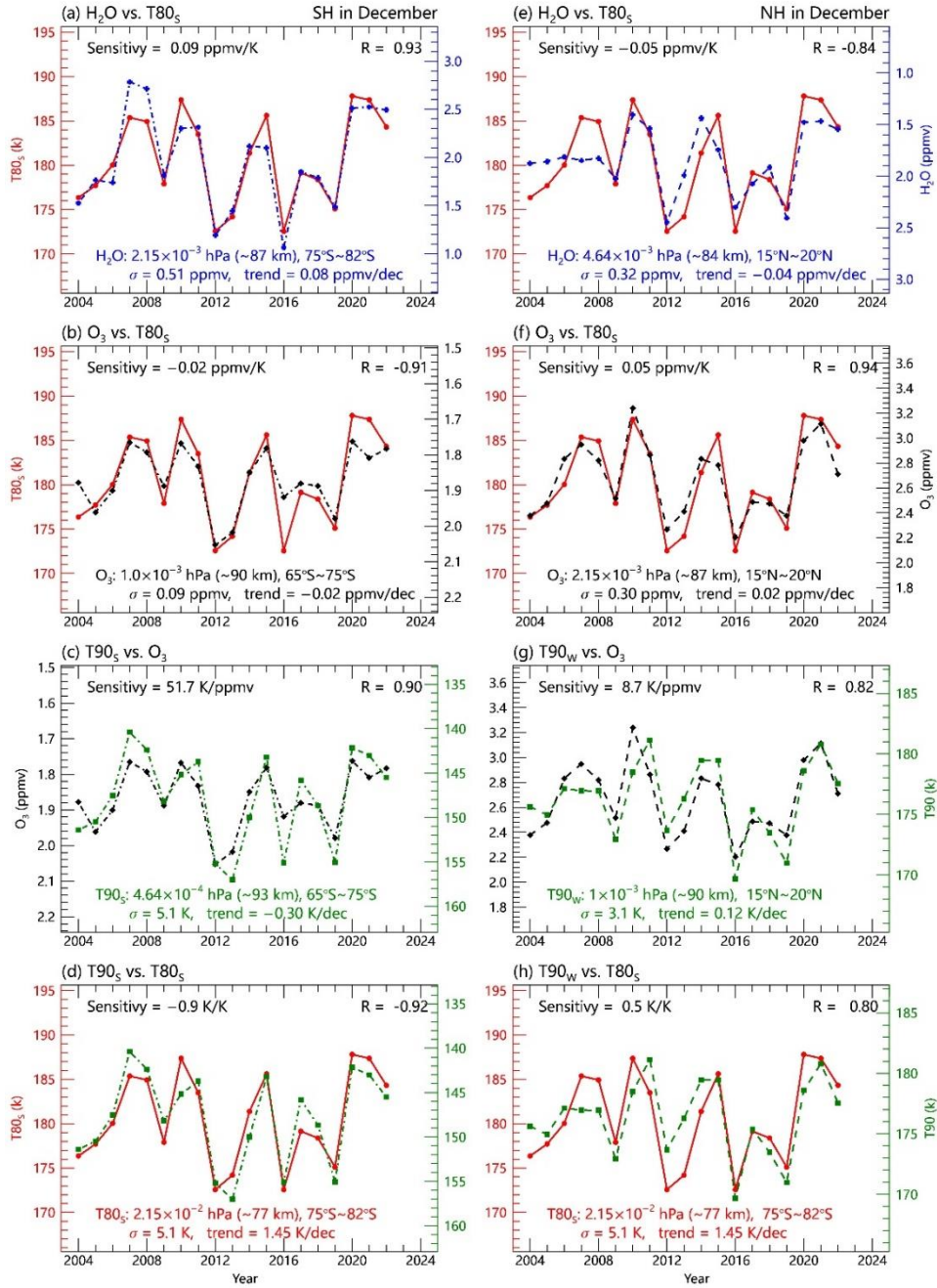
Figure 3. Hemispheric responses of mesospheric (a, e) \text{H}_2\text{O} , (b, f) \text{O}_3 , and (d, h) T90 to upwelling variability (indicated by \text{T80}_s ) during December, showing anti-phase behavior between (left) summer and (right) winter hemispheres. Panels (c, g) show \text{O}_3 -T90 correlations. All plots display monthly and zonal means from MLS/Aura observations during 2004-2022, with correlation coefficients ( R ), sensitivities, standard deviations ( \sigma ), and trends derived from linear regression analysis. The opposing \text{H}_2\text{O} responses reflect hydration (winter hemisphere, negative correlation) and dehydration (summer hemisphere, positive correlation), while \text{O}_3 and T90 variations demonstrate the consequent chemical and thermal feedbacks.
