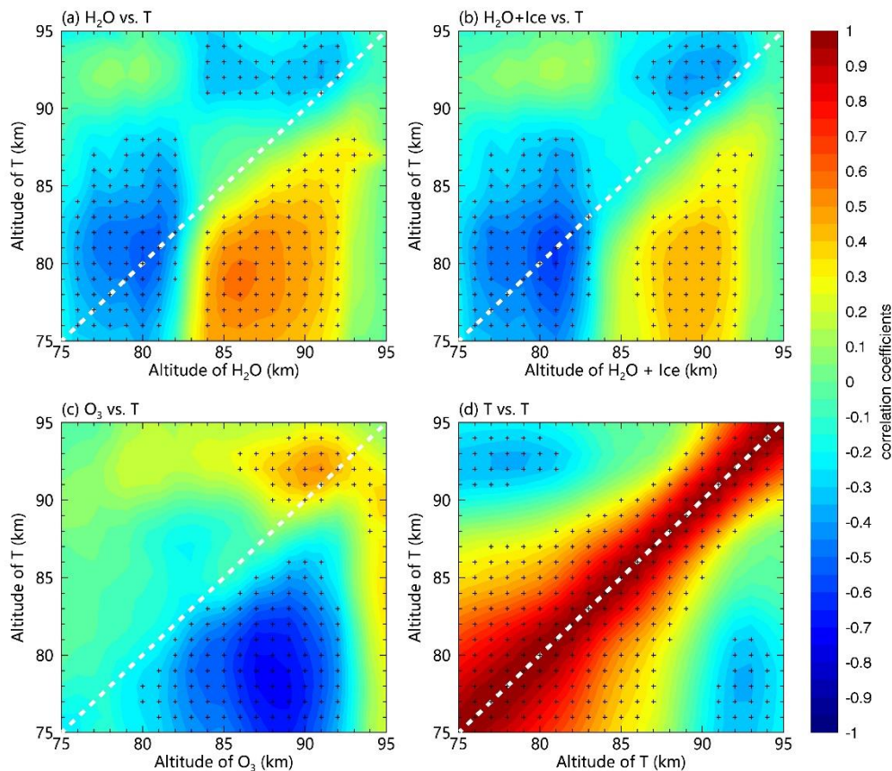
220 Figure 7. Daily-scale bottom-up control processes observed by SOFIE at \sim 70^\circ\text{S} for the SH PMC seasons during 2007-2013. (a) \text{H}_2\text{O} above and below 83 km are both subject to the control of \text{T80}_\text{s} rather than local temperatures. (b) Combined \text{H}_2\text{O} and ice content demonstrate similar \text{T80}_\text{s} dependence. (c) Anti-correlation between \text{O}_3 and \text{T80}_\text{s} , accompanied by positive \text{O}_3 - \text{T90} relationship. (d) Negative correlation between \text{T90}_\text{s} and \text{T80}_\text{s} . Correlation coefficients are calculated for -10 to 50 days relative to solstice (35-day running mean removed), with the 0.95 significance level marked by dots.
