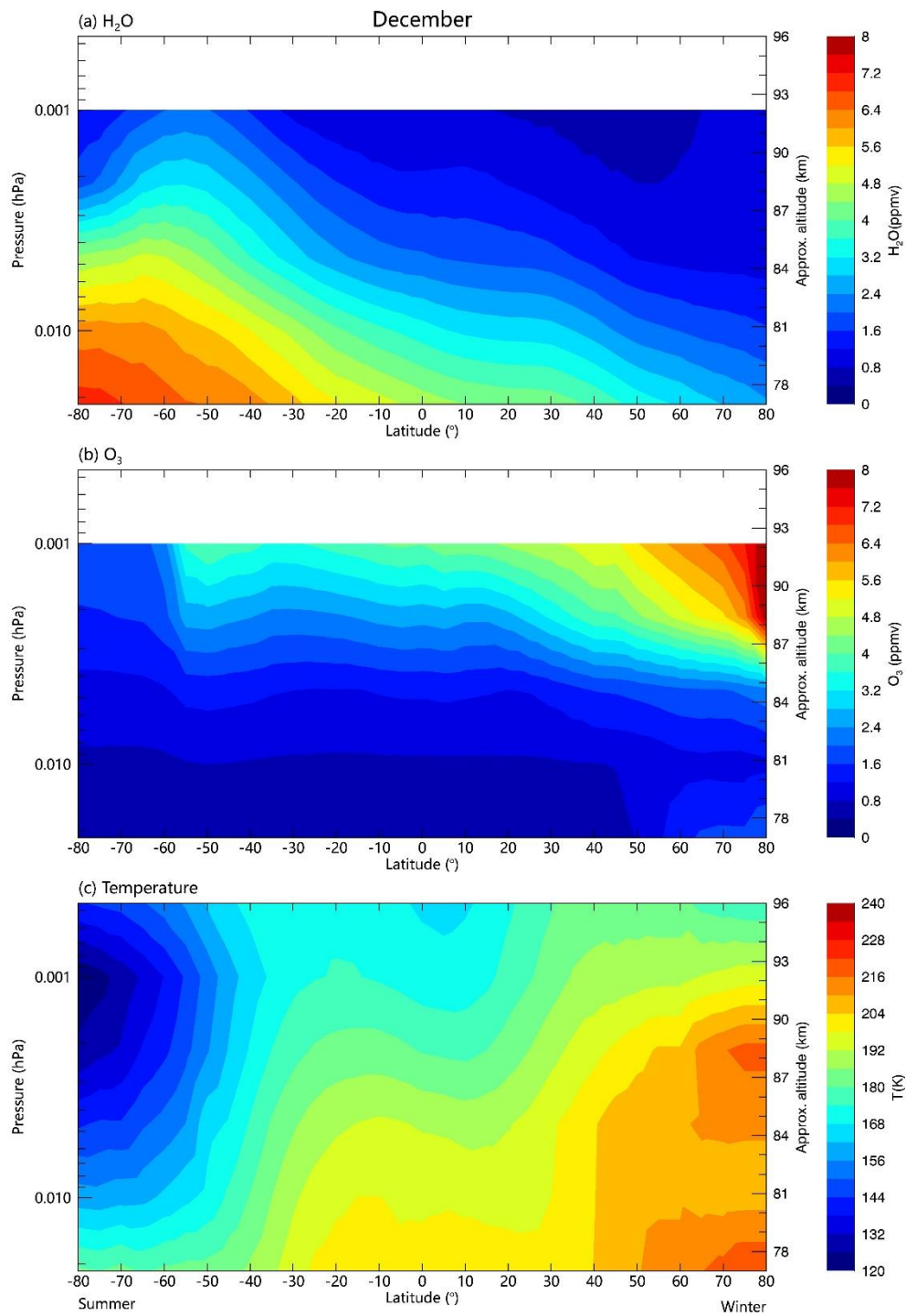
Figure 1. December climatology of (a) water vapor mixing ratio, (b) ozone mixing ration, and (c) temperature in the upper mesosphere. Data represent monthly means from MLS/Aura observations during 2004-2022.
