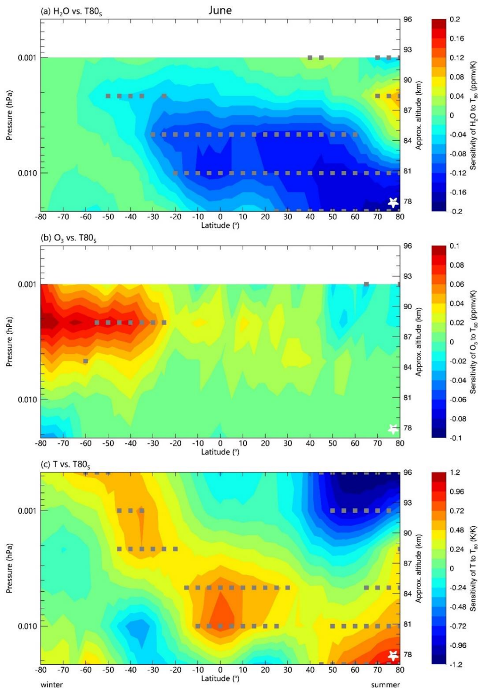
240 Figure 10. Spatial patterns of bottom-up control processes during June showing (a) \text{H}_2\text{O} , (b) \text{O}_3 , and (c) temperature responses to upwelling (indicated by \text{T80}_s , white stars), analogous to but weaker than December patterns (Fig. 4). Sensitivities derived from linear regression of MLS/Aura data (2004-2022) show reduced but still significant anti-phase relationships between hemispheres compared to December. Gray dots mark the 0.95 significance level. Note the responses of variables in winter hemisphere extend to \sim 50^\circ\text{S} in June.
