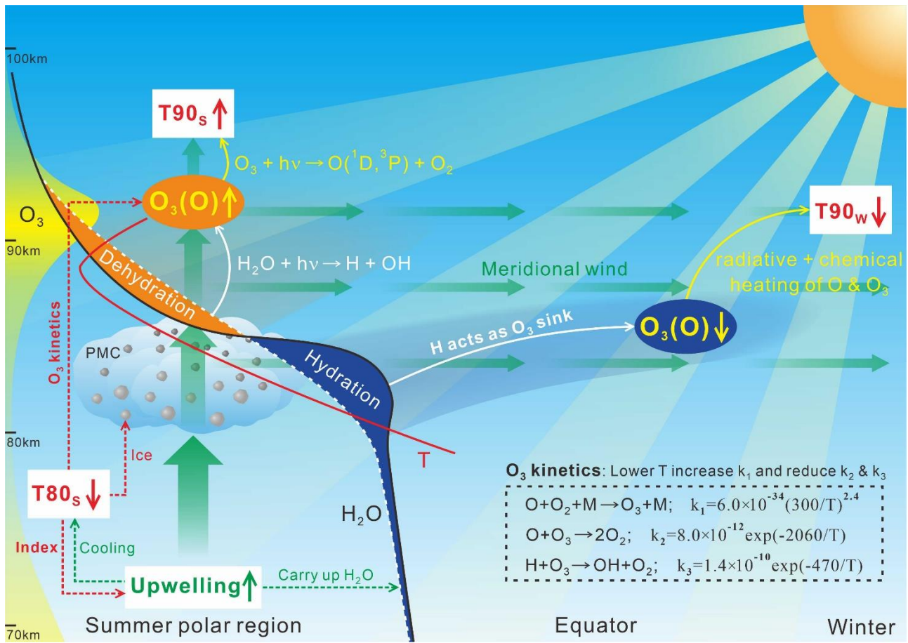
140 Figure 2. Schematic diagram of the bottom-up control mechanism in solstice months, showing how summer polar upwelling controls interhemispheric climate variability through coupled dynamical and chemical processes. Key pathways include: (1) winter-hemisphere hydration is induced by summer polar upwelling in combination with meridional transport, and summer-hemisphere dehydration is governed by the cold-trap effect; (2) subsequent modulation of O 3 through H-driven ozone loss and temperature-dependent ozone kinetics, with O varying in pace with O 3 due to the ozone photochemical equilibrium assumption; and (3) resulting temperature (T 90 ) variations via radiative and chemical heating of O 3 /O. 145
