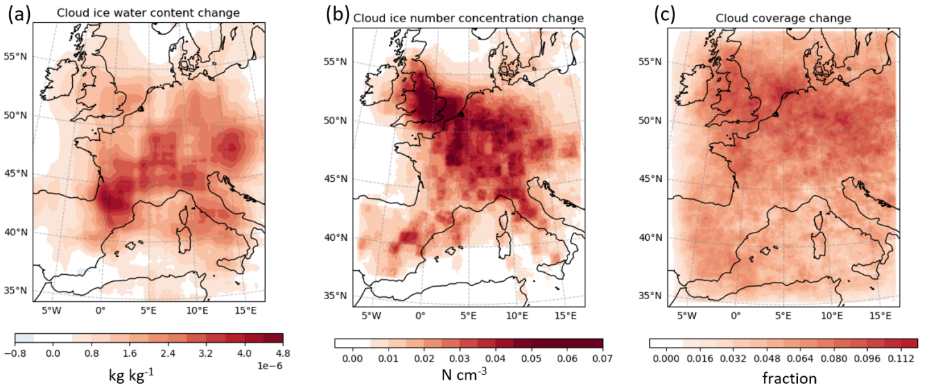
Figure 6: Spatial distribution of annual mean (averaged over the 10 days in all twelve months) changes in cloud (a) ice water content in \text{kg kg}^{-1} , (b) ice number concentration in \text{cm}^{-3} , and (c) ice cloud coverage.
