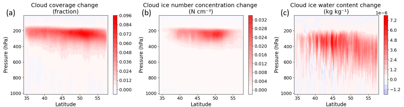
335 Figure 7: Vertical cross section of annual mean changes in cloud (a) coverage, (b) ice crystal number concentration ( \text{cm}^{-3} ), and (c) cloud ice mass ( \text{kg kg}^{-1} ).
