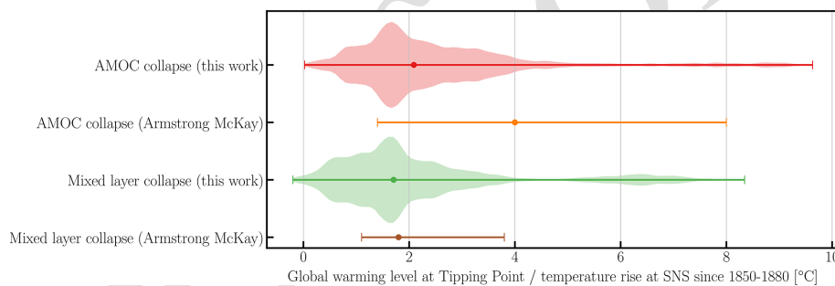
Figure 18. Comparison of global warming levels thresholds for tipping points (Armstrong McKay et al., 2022) and the occurrence of maximal change of SNS (this work), where we compare the full CDF of Fig. 17 illustrated with violin plots, to the Min, Estimate, and Max global warming level thresholds described in Armstrong McKay et al. (2022). On top of the violin plots, we indicated the 0th-, 50th- (i.e. median), and 100th-percentiles of the CDFs with error bars. We compare our result AMOC collapse (Category D) to the Atlantic M.O. Circulation collapse, and our result NH Mixed-layer collapse to the Labrador-Irminger Seas/SPG Convection collapse. As discussed in the text, the metrics from Armstrong McKay et al. (2022) and this work are inherently different, and this comparison is therefore not one to one.
