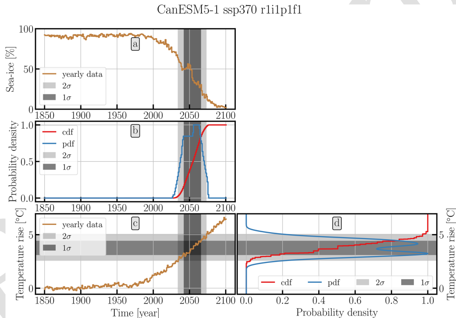
Figure A3. Method of obtaining the global temperature rise at shift for an SNS. We analyze the yearly data of panel (a) (see text for details) to determine when the change is maximal. The resulting CDF and PDF are shown in panel (b). Based on the CDF in panel (b), we draw the vertical 1\sigma and 2\sigma probability intervals. In panel (c), we add the global temperature rise relative to the 1850–1880 average. By weighing the temperature rise values with the PDF of panel (b) we can calculate panel (d), where we show the CDF and the PDF of the shift to occur at a certain temperature rise. The PDF in panel (d) is smoothed by a Gaussian with a standard deviation of 0.2^\circ\text{C} for illustration purposes. The horizontal 1\sigma and 2\sigma probability intervals are based on the CDF of panel (d).
