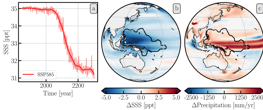
Figure 9. The time series (panel a ) of category “E” in IPSL-CM6A-LR (r1i1p1f1) is shown together with the change in SSS (panel b ) and precipitation (panel c ). The change for SSS and precipitation is calculated between the averages for the 1850–1880 and 2270–2300 periods. See the caption of Fig. 7 for further details.
