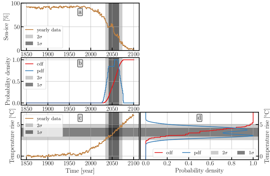
Figure A3. Method of obtaining the global temperature rise at shift for an SNS. We analyze the yearly data of panel a (see text for details) to determine when the change is maximal. The resulting CDF and PDF are shown in panel b. Based on the CDF in panel b, we draw the vertical 1\sigma and 2\sigma probability intervals. In panel c, we add the global temperature rise relative to the 1850-1880 average. By weighing the temperature rise values with the PDF of panel B we can calculate panel d, where we show the CDF and the PDF of the shift to occur at a certain temperature rise. The PDF in panel d is smoothed by a Gaussian with a standard deviation of 0.2^\circ\text{C} for illustration purposes. The horizontal 1\sigma and 2\sigma probability intervals are based on the CDF of panel d.
