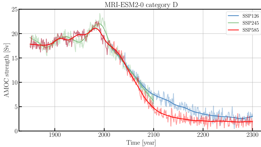
Figure 8. Category “D” for the MRI-ESM2-0 model (SSP126: r1i1p1f1, SSP245: r4i1p1f1, SSP585: r1i1p1f1). The yearly data is illustrated by the shaded lines while the solid lines depict the smoothed time series, where the smoothing is the same as in Figure 2.
