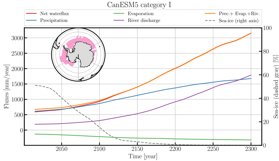
Figure 13. Case “I” for the CanESM5 model (r11p1f1) as found in the net water flux, split by precipitation, evaporation and river discharge (purple). By summing (Prec. + Evap. + Riv.) the contributions of precipitation, evaporation, and river discharge we are able to close the water budget in this region. The right axis additionally shows the sea-ice cover in this region. The inset shows the region of the category I case in the CanESM5 model, where the region of the SNS is illustrated as the pink shaded region.
