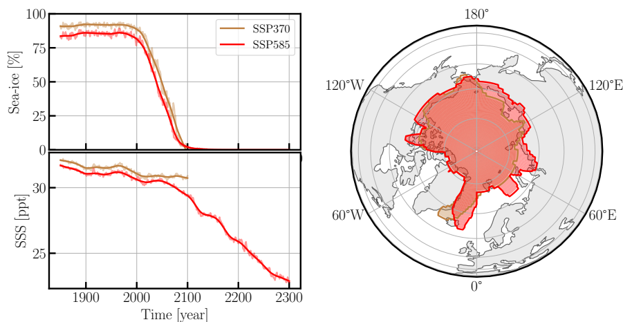
Figure 4. Category “A” for the CanESM5 model (r11p1f1), where the SSP370 model run was evaluated until the year 2100 and SSP585 was extended to 2300. The sea surface salinity (SSS) is expressed in parts per thousand (ppt). The region (right) corresponds to the region wherein the sea-ice SNS is found, and, for consistency, the left panels correspond to these regions. For SSP585, an SNS was also found in a (smaller) sub-region for SSS. See caption of Figure 3 for details.
