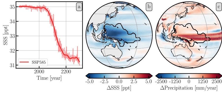
Figure 9. The time series (panel a) of category “E” in IPSL-CM6A-LR (r1i1p1f1) is shown together with the change in SSS (panel b) and precipitation (panel c). The change for SSS and precipitation is calculated between the averages for the 1850 – 1880 and 2270 – 2300 periods. See the caption of Figure 7 for further details.
