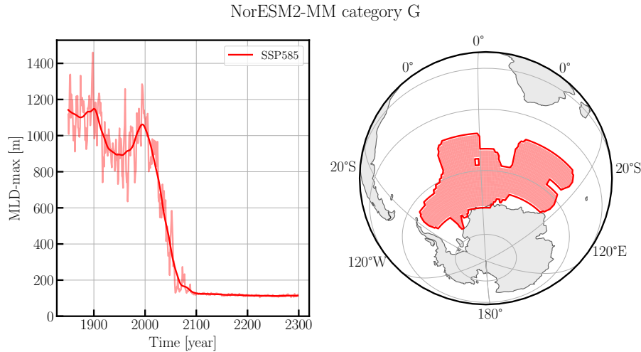
Figure 11. Category “G” for the NorESM2-MM model (r1i1p1f1). See caption of Figure 3 for details.
