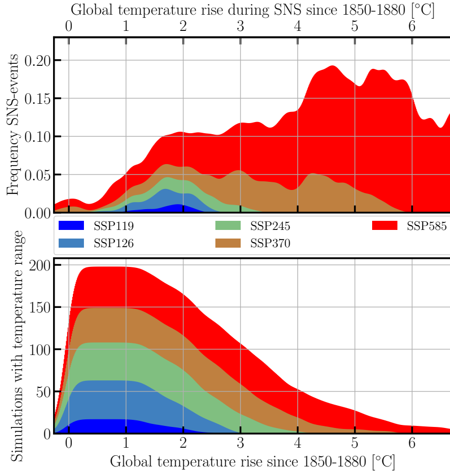
Figure 14. Frequency of SNS (top) as a fraction of the number of available simulations that reach such a temperature range (bottom). The frequency of a shift is calculated by dividing the summed fractional probability of an SNS to occur in a temperature interval, divided by the number of available simulations that cover that interval (see text for details). The data is smoothed using a Gaussian convolution with a standard deviation of 0.1^{\circ}\text{C} . The temperature scale (x-axis) is limited to -0.3 - 6.7^{\circ}\text{C} , where at least five simulations are available (bottom panel).
