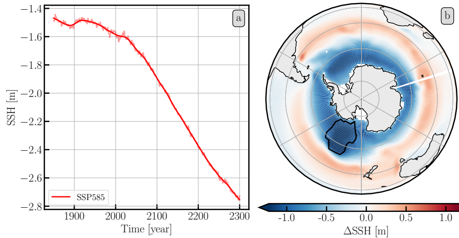
Figure 12. Time series (panel a) of category “H” in IPSL-CM6A-LR (r1i1p1f1) together with the change in SSH (panel b). The change of SSH is calculated between the averages for the 1850 – 1880 and 2270 – 2300 periods. See the caption of Figure 7 for further details.
