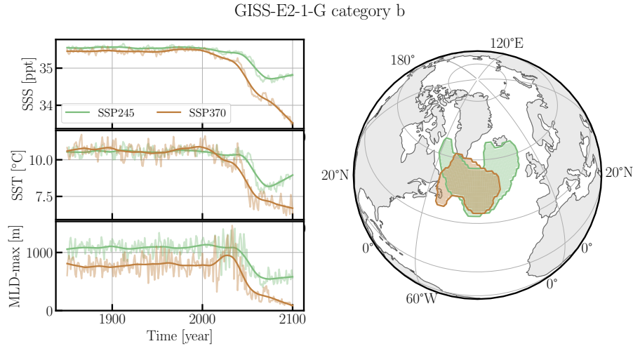
Figure 5. Category “b” for the GISS-E2-1-G model (SSP245: r2i1p5f1, SSP370: r4i1p5f1). The region-SSP245 region belongs to the SNS detected in SSS, while the SNS for the SSP370 region is detected in SST. See caption of Figure 3 for details.
