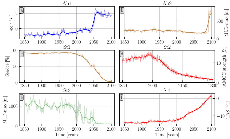
Figure 2. Examples of the six formal classification criteria (Ab1-St4), see text for further details. Panels Ab1a , Ab2b , St1c , St2d , St3e and St4f refer to SNS 61, 60, 6, 50, 66, and 18 respectively in Table A3. The solid lines indicate the smoothed yearly time series (which are illustrated as shaded lines). The data is smoothed using a Lowess filter with a window of 40 years.
