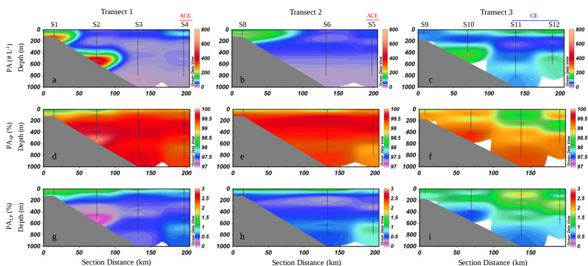
Fig. 4 Vertical distribution of particles abundance (PA, # L^{-1} ) and the relative proportion of small particles ( PA_{SP} , ESD < 500 \mu m ) and large particles ( PA_{LP} , ESD \geq 500 \mu m ) within the total particle abundance. PA: a-c; PA_{SP}\% : d-f; PA_{LP}\% : g-i. SP: small particles; LP: large particles. ACE represents stations influenced by anticyclonic eddies, while CE represents stations influenced by cyclonic eddies.
