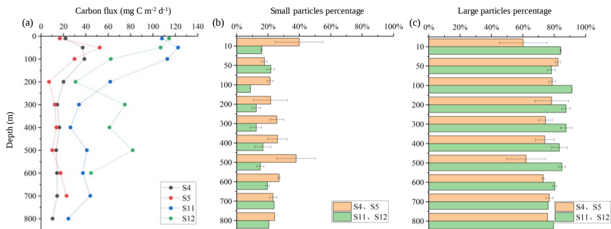
Fig. 8 POC flux derived from UVP data in different water layers and contributions of small and large particles in the anticyclonic eddy region (S4, S5) and cyclonic eddy region (S11, S12). a: Carbon flux (mg C m -2 d -1 ); b: Small particles percentage; c: Large particles percentage. b, c: mean values and standard deviations of those two stations.
