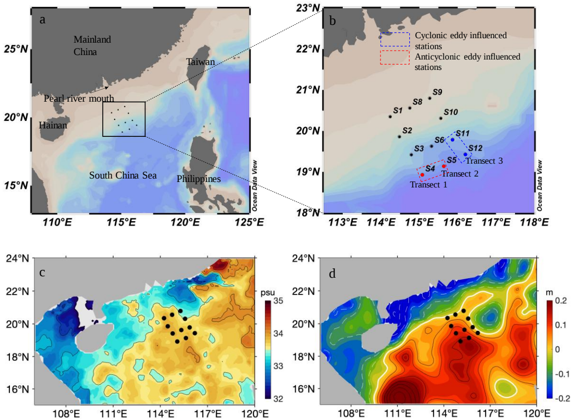
Fig. 1 Study area and survey stations in the SCS continental slope. a: the study region; b: the enlarge view; c: sea
