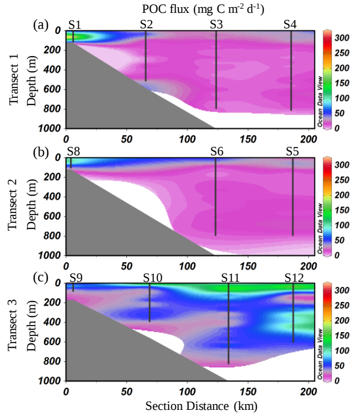
Fig. 7 Vertical distribution of POC flux across the three transects ( \text{mg C m}^{-2} \text{d}^{-1} ) in the study area. a: Transect 1; b: Transect 2; c: Transect 3
