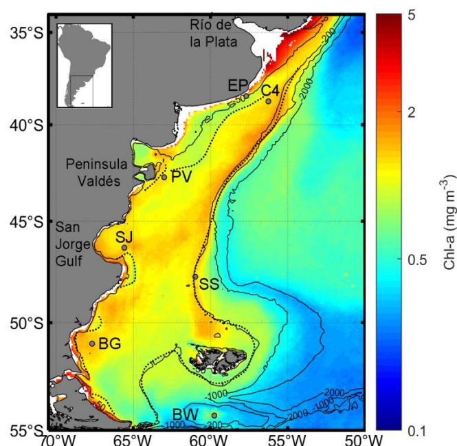
169 Figure 1 Selected sites overlaid on the mean surface Chl-a concentration distribution from CCI-OC v6.0 (1998–2020). Black 170 solid lines indicate the 50 m, 200 m, 1,000 m, and 2,000 m isobaths. Schematic frontal zones in the Southwest Atlantic Ocean 171 (SWAO) are shown as black dotted lines, based on Acha et al. (2018). Site abbreviations correspond to those listed in Table 1.
