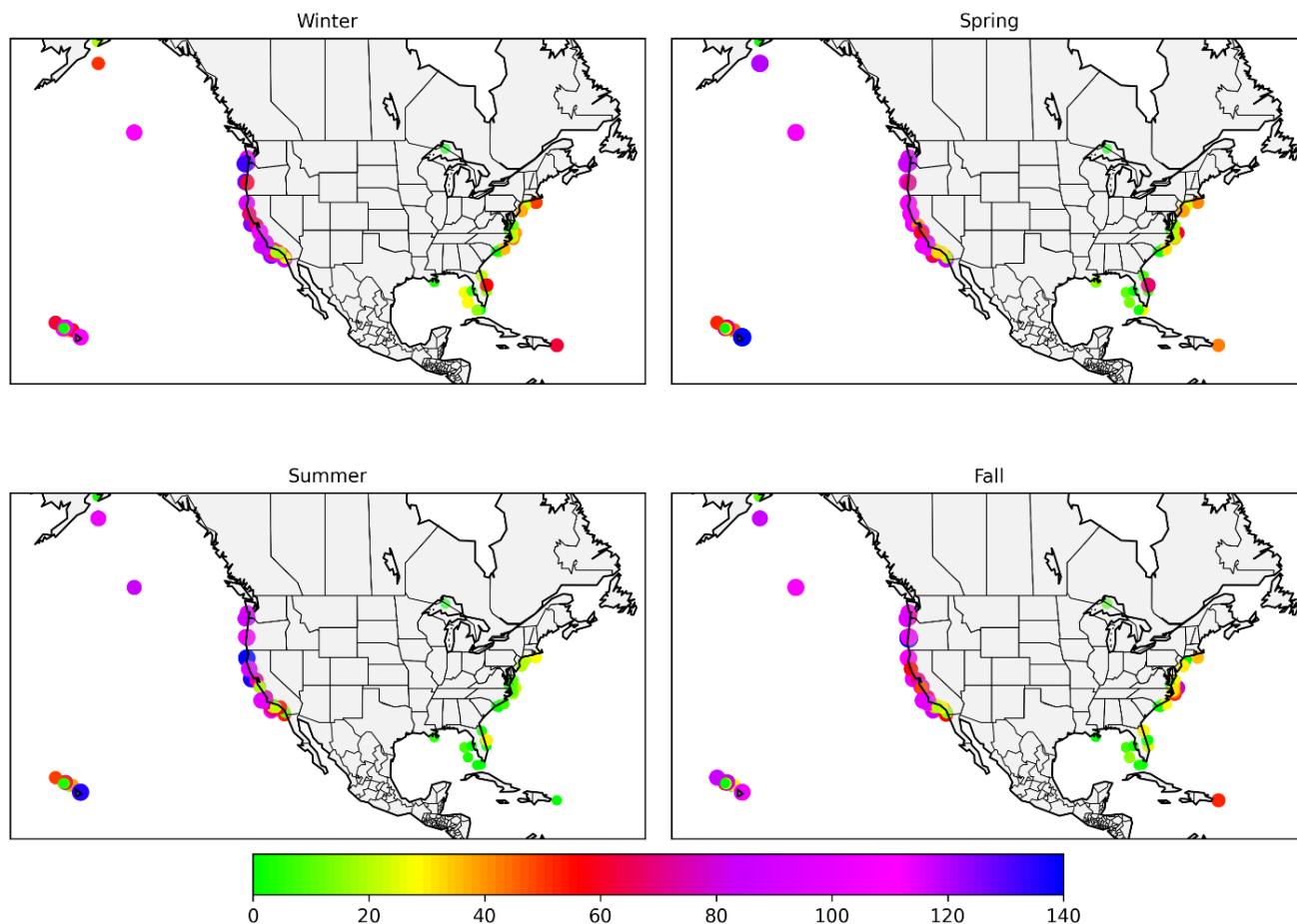
Fig.1 – Average number of rogue waves per season based on CDIP buoy data from the FOWD dataset from 2015 to 2021. Color gradients represent the average number of rogue waves detected per season at each buoy location. Seasons are defined as: Winter from December to February, Spring from March to May, Summer from June to August and Fall from September to November.
