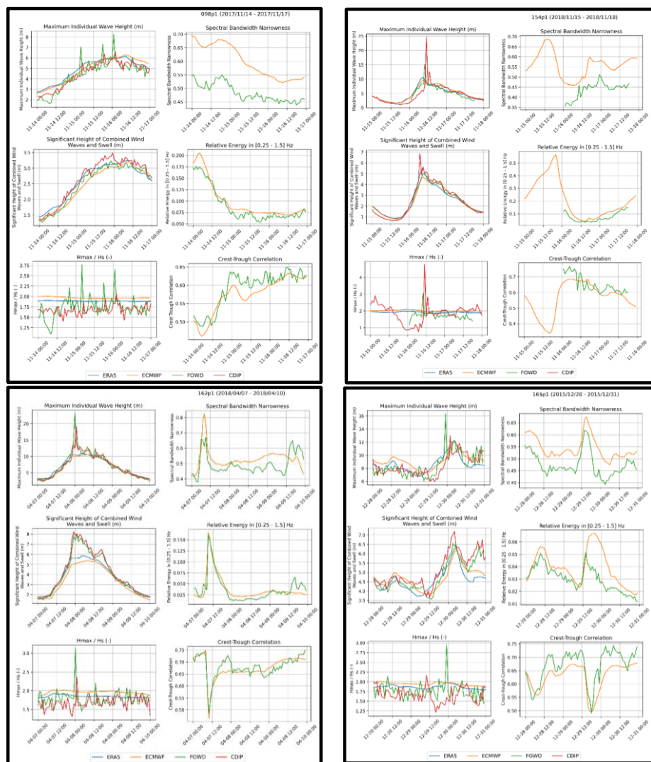
550 Fig. 5 – Specific rogue wave event analysis at four different buoy stations (098, 154, 162, and 166) during a period of 72 hours. ERA5 data is depicted in blue, ECMWF CY47R1 data depicted in orange, FOWD data depicted in green and raw CDIP data depicted in red. Buoy Hmax from zero-crossings; model (Hmax) is envelope-based.
