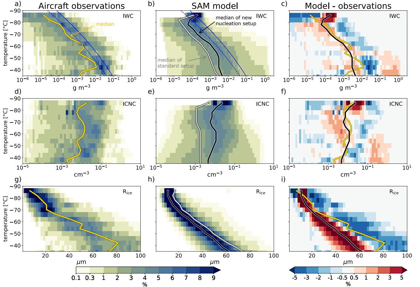
Figure 3. Cirrus cloud properties from tropical aircraft measurements (first column) and SAM model simulations with improved micro-physics at 1 km horizontal grid spacing (second column). Thick solid lines represent median values. Gray lines in the middle column represent median values of the standard model setup. The third column displays the difference between improved SAM and aircraft data; lines are repeated from the first and second columns for reference. Blue lines in panels a) and b) show the theoretical maximum IWC formed locally by vapor deposition under ice-supersaturated conditions, based on RH_{ice} required to trigger homogeneous nucleation (Koop et al., 2000) (solid) and RH_{ice} of 120%, more typical for heterogeneous ice nucleation (dashed). All data is sorted into 4^\circ C temperature bins, with values normalized to add up to 100% within each temperature bin.
