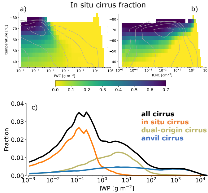
Figure 6. Fraction of in situ cirrus represented in the (a) temperature-IWC and (b) temperature-ICNC space for the cirrus classification criterion from Fig. 5. The gray lines in the contour indicate the joint distribution of cloud occurrence in each two-dimensional phase space. Panel c) shows the fraction of cirrus binned by IWP.
