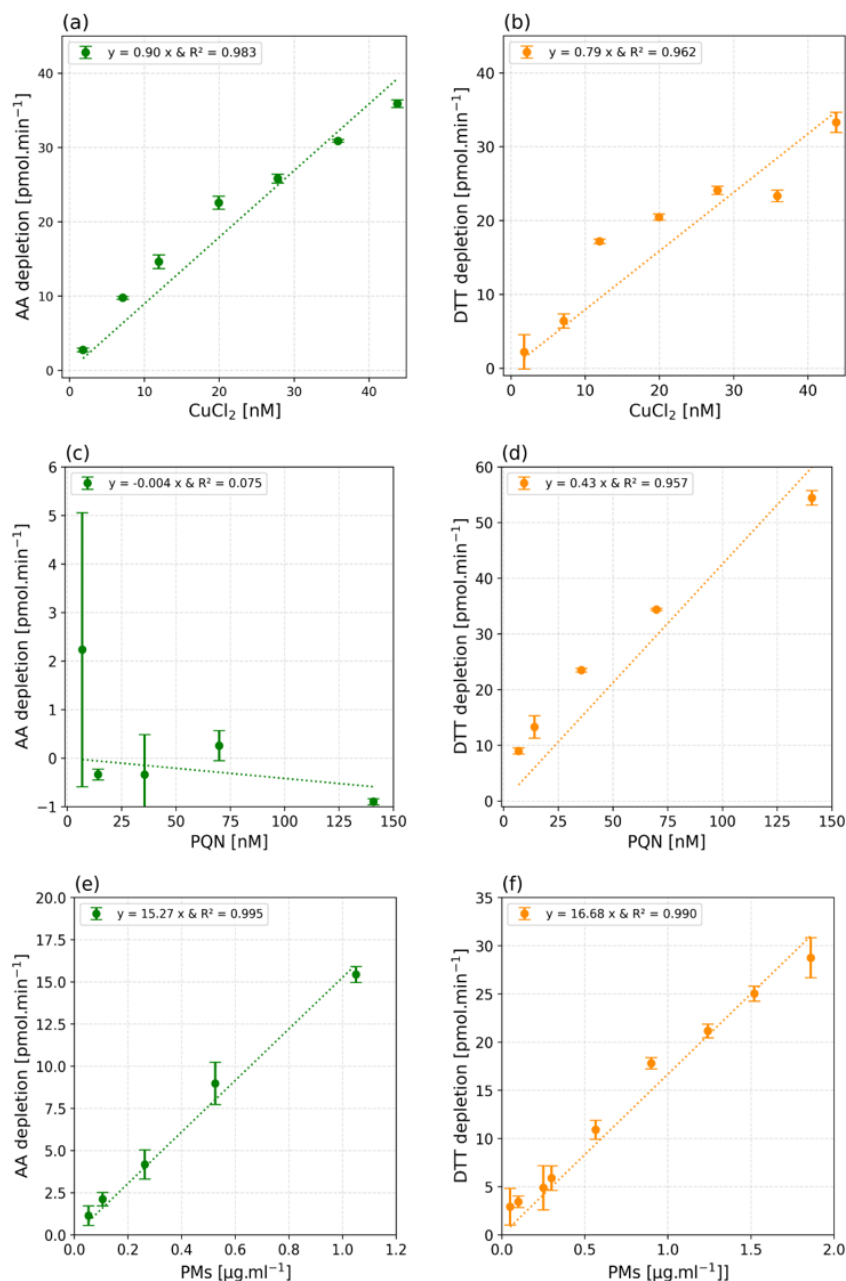
Figure 5. Green dots represent the ascorbic acid consumption rate, i.e., depletion, in [\text{pmol}\cdot\text{min}^{-1}] as a function of \text{CuCl}_2 (a) and PQN (c) concentration in [nM]. The orange dots represent the dithiothreitol depletion in [\text{pmol}\cdot\text{min}^{-1}] as a function of \text{CuCl}_2 (b) and PQN (d) concentration in [nM]. (e) Green dots represent the ascorbic acid depletion, in [\text{pmol}\cdot\text{min}^{-1}] as a function of PMs samples [ \mu\text{g}\cdot\text{ml}^{-1} ] taken from a traffic site filter (Bern), and (f) orange dots represent the dithiothreitol depletion in [\text{pmol}\cdot\text{min}^{-1}] as a function of PMs samples [ \mu\text{g}\cdot\text{ml}^{-1} ] taken from an urban background winter filter (Grenoble). Dashed lines represent the modelled linear regressions. Each sample was analysed in triplicate, and the figures present average (dots), with the error bars representing \pm 1\sigma .
