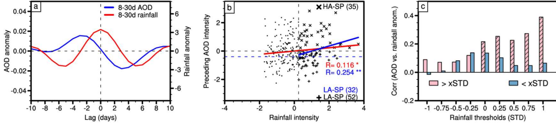
Figure 2. (a) Evolution of 8–30-day precipitation (red curve, \text{mm d}^{-1} ) and 8–30-day AOD (blue curve, unitless) associated with quasi-biweekly precipitation events, defined as periods with positive 8–30-day rainfall anomalies over South China. These results are based on CPC rainfall data and MERRA-2 AOD data. Day 0 denotes the peak of rainfall events, while negative and positive values on the x -axis indicate days before and after the peak, respectively. (b) Scatterplot of rainfall intensity (i.e., 8–30-day-filtered rainfall anomalies at Day 0; x -axis, \text{mm d}^{-1} ) versus preceding AOD intensity (represented by the peak value of 8–30-day-filtered AOD anomalies during Days -6 to -1 ; y -axis, unitless), with both variables normalized by their climatology. The red line represents the linear regression fitted to all cases, while the blue line corresponds to events where rainfall intensity exceeds 0.25\sigma . The correlation coefficients between the two variables are shown in the bottom right corner, with single and double asterisks indicating significance at the 90% and 95% confidence levels, respectively. Enhanced 8–30-day rainfall events ( >0.25\sigma ) are classified into High AOD–Strong Precipitation (HA–SP; cross sign) and Low AOD–Strong Precipitation (LA–SP; plus sign) categories, with case counts displayed in each quadrant. To maintain nearly equal sample sizes for these two groups, the LA–SP classification is determined using an AOD anomaly threshold of -0.4\sigma (blue dashed line and blue text). (c) Correlation coefficients between preceding AOD intensity and rainfall intensity at Day 0 for different rainfall amplitude thresholds (bins with 0.25\sigma intervals). Pink bars represent correlations when 8–30-day rainfall exceeds a given threshold, while blue bars show correlation coefficients for the remaining events. Hatching indicates correlations significant at the 90% confidence level.
