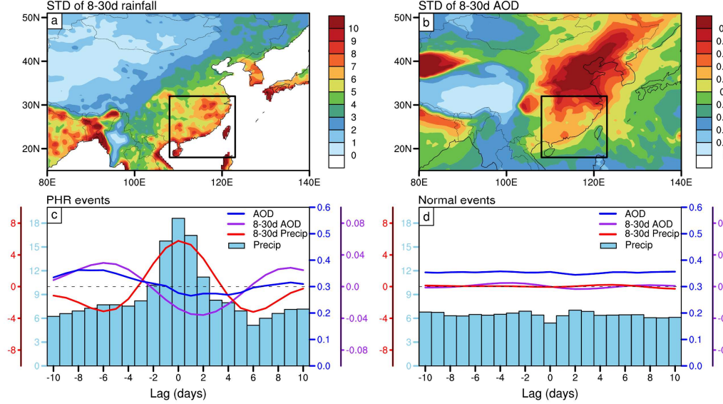
Figure 1. Spatial distributions of the standard deviation of (a) 8–30-day-filtered precipitation anomalies ( \text{mm d}^{-1} ) and (b) 8–30-day-filtered aerosol optical depth anomalies (AOD; unitless) during MJJAS from 2000 to 2021, based on CPC rainfall data and MERRA-2 AOD data, respectively. The black boxes indicate the study domain of southern China ( 18^{\circ} – 32^{\circ}\text{N} , 108^{\circ} – 123^{\circ}\text{E} ). (c) Composites of daily precipitation (light blue bars, left y-axis in light blue, \text{mm d}^{-1} ), 8–30-day-filtered precipitation (red curve, left y-axis in red, \text{mm d}^{-1} ), AOD (blue curve, right y-axis in blue, unitless), and 8–30-day-filtered AOD (purple curve, right y-axis in purple, unitless) associated with persistent heavy rainfall events over South China. The x-axis is centered at “0”, representing the median timing of individual rainfall events, with negative and positive values indicating periods before and after the event. (d) As in (c) but for the composites of normal-intensity rainfall events.
