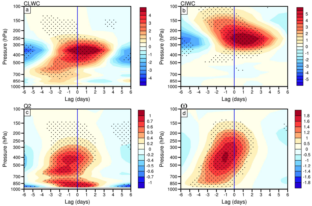
Figure 5. Height–time evolution of 8–30-day anomalies in (a) liquid cloud water content (CLWC; 10^{-6} \text{ kg kg}^{-1} ), (b) ice cloud water content (CIWC; 10^{-6} \text{ kg kg}^{-1} ), (c) latent heat heating ( \text{K d}^{-1} ), and (d) vertical velocity anomalies ( -10^{-2} \text{ Pa s}^{-1} ) between the HA–SP and LA–SP events, based on the MERRA-2 data. Stippling denotes differences statistically significant at the 90% confidence level. Vertical blue lines denote the peak timing of heavy rainfall event (Day 0).
