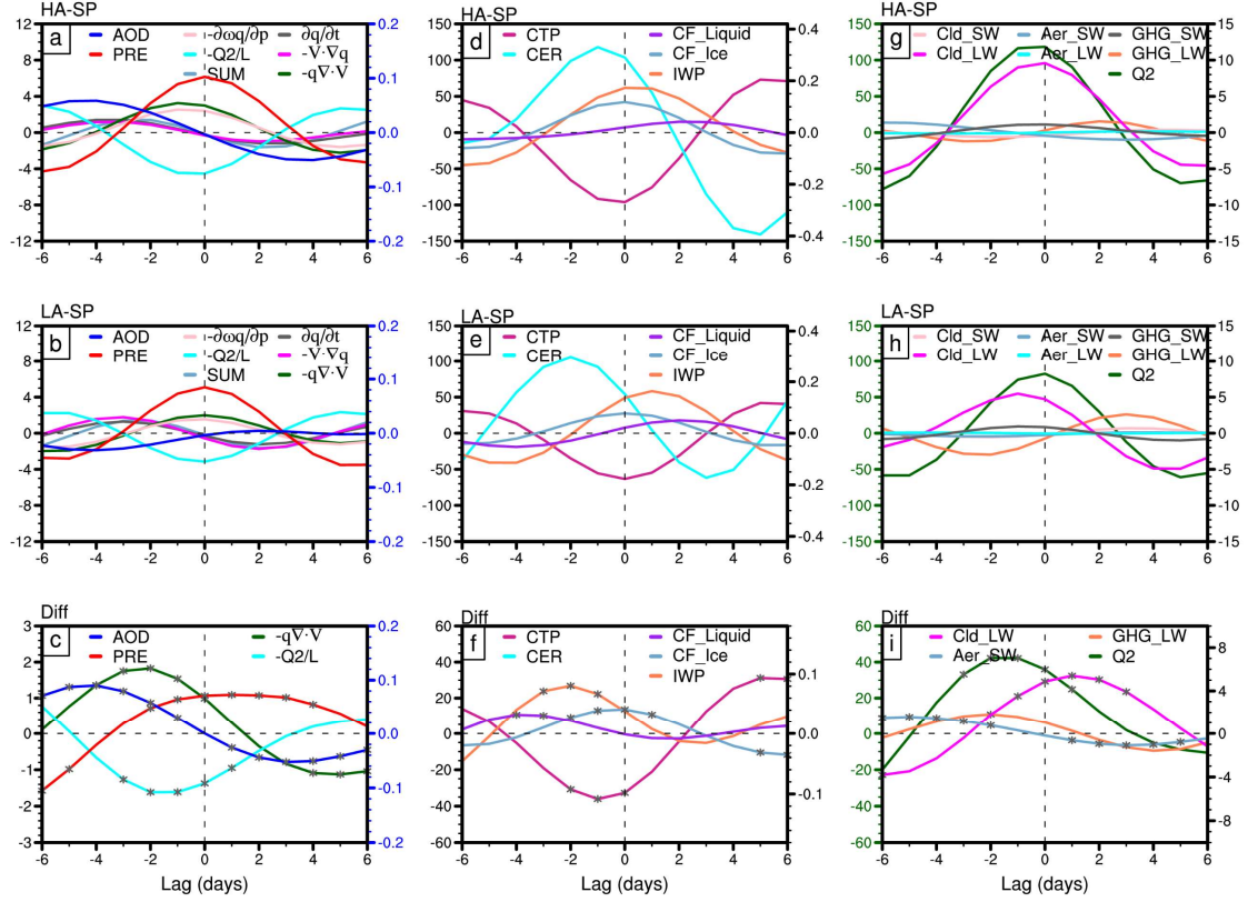
Figure 4. As in Fig. 2a, but for the composite evolution of 8–30-day (a) precipitation (red curve; left y-axis, \text{mm d}^{-1} ), AOD (blue curve; right y-axis in blue, unitless), and individual moisture budget terms (various colored curves representing each budget term in Eq. (1); left y-axis, \text{mm d}^{-1} ) associated with HA–SP events. (d, g) As in (a), except that (d) shows the 8–30-day evolution of cloud top pressure (CTP; magenta curve; left y-axis, hPa), ice water path (IWP; orange curve; left y-axis, \text{g m}^{-2} ), cloud droplet effective radius (CER; orange curve; right y-axis, \mu\text{m} ), liquid cloud fraction (CF_Liquid; purple curve; right y-axis, unitless), and ice cloud fraction (CF_Ice; light blue curve; right y-axis). Panel (g) presents 8–30-day column-integrated latent heat heating ( Q_2 ; green curve; left y-axis in green, \text{W m}^{-2} ) and 8–30-day radiative budget terms calculated from Eq. (2) (right y-axis, \text{W m}^{-2} ), including longwave/shortwave cloud radiative effects (Cld_LW/Cld_SW; magenta curve/pink curve), longwave/shortwave aerosol direct radiative effects (Aer_LW/Aer_SW; cyan curve/light blue curve), and longwave/shortwave greenhouse gas radiative effects (GHG_LW/GHG_SW; orange curve/gray curve). (b, e, h) and (c, f, i) are similar to (a, d, g), but represent the composite results for LA–SP events and the differences between HA–SP and LA–SP events, respectively. In panels (c) and (i), only
