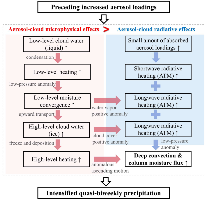
Figure 10. Schematic diagram illustrating the mechanisms of aerosol effects on heavy rainfall events at the 8–30-day timescale. The symbol “↑” denotes the enhancement of the corresponding processes, “ATM” refers to the whole atmosphere, and “>” indicates stronger contributions of the process to heavy precipitation events.
