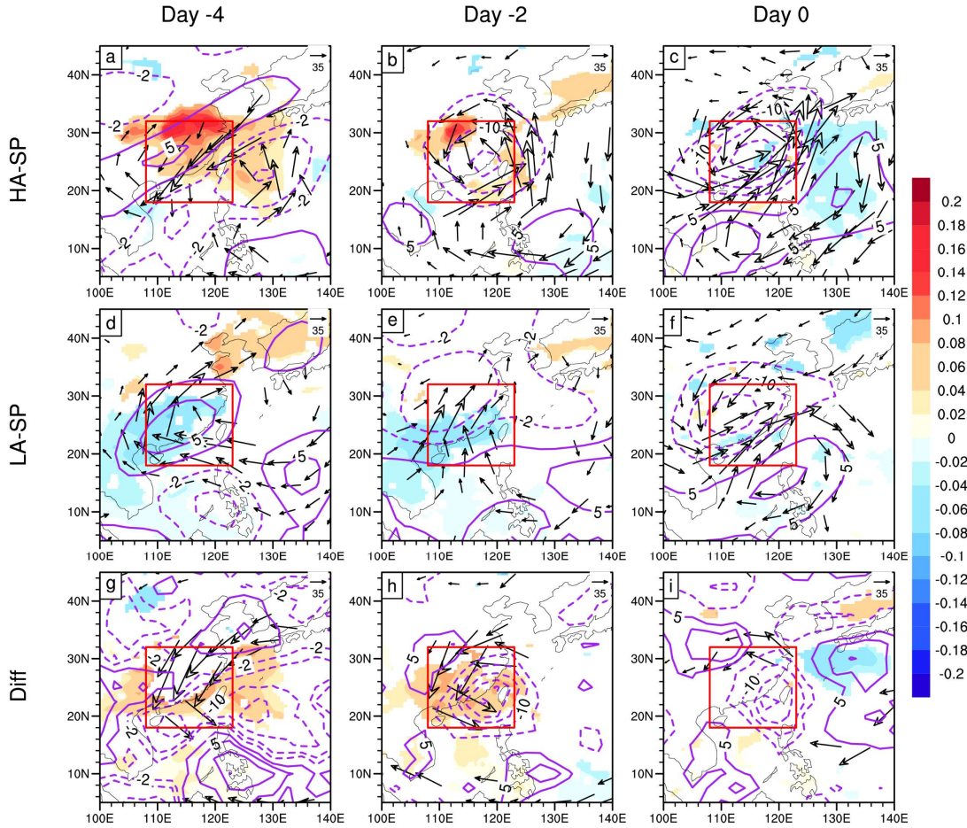
Figure 3. (a)–(c) Composite evolution of 8–30-day outgoing longwave radiation (OLR; purple contours, \text{W m}^{-2} ), AOD (shading, unitless), and column-integrated moisture flux (vectors, \text{kg m}^{-1} \text{s}^{-1} ) at 4, 2, and 0 days before the occurrence of HA–SP events, respectively. The results are based on NOAA OLR data, MERRA-2 AOD and meteorological data. (d)–(f) and (g)–(i) Similar to (a)–(c), but for the composite results of LA–SP events and the differences between HA–SP
