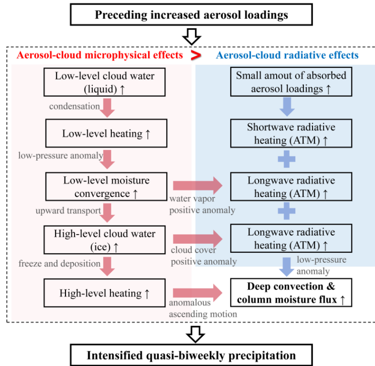
613 Figure 10. Schematic diagram illustrating the mechanisms of aerosol effects on heavy rainfall events at the 8–30-day 614 timescale. The symbol “↑” denotes the enhancement of the corresponding processes, “ATM” refers to the whole 615 atmosphere, and “>” indicates stronger contributions of the process to heavy precipitation events.
