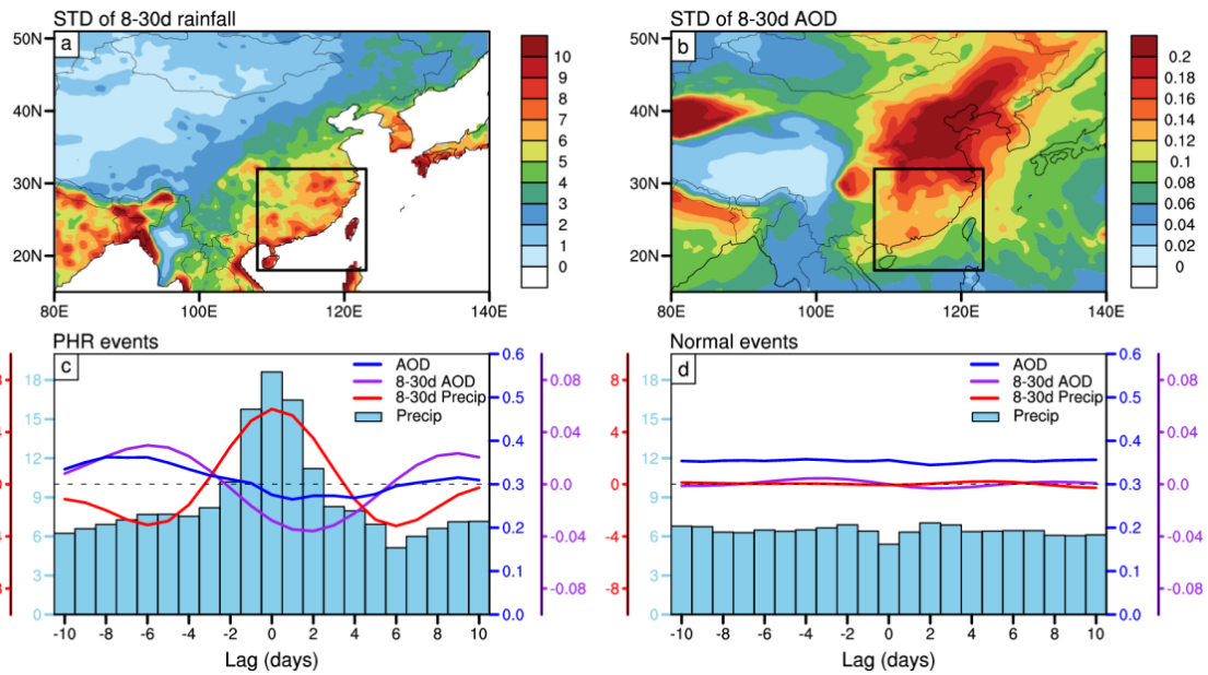
235 236 Figure 1. Spatial distributions of the standard deviation of (a) 8–30-day-filtered precipitation anomalies (mm d -1 ) and (b) 237 8–30-day-filtered aerosol optical depth anomalies (AOD; unitless) during MJJAS from 2000 to 2021, based on CPC 238 rainfall data and MERRA-2 AOD data, respectively. The black boxes indicate the study domain of southern China (18°– 239 32°N, 108°–123°E). (c) Composites of daily precipitation (light blue bars, left y-axis in light blue, mm d -1 ), 8–30-day-
