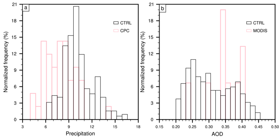
Figure 6. Normalized occurrence frequency Probability density functions (PDFs) of (a) daily precipitation ( \text{mm d}^{-1} ) and (b) AOD (unitless) from observations (pink curves, CPC rainfall and MODIS AOD data) and the CTRL experiment (black curves) during the model integration period over the key region of interest ( 21^{\circ} – 24^{\circ}\text{N} , 111^{\circ} – 116^{\circ}\text{E} ) in South China.
