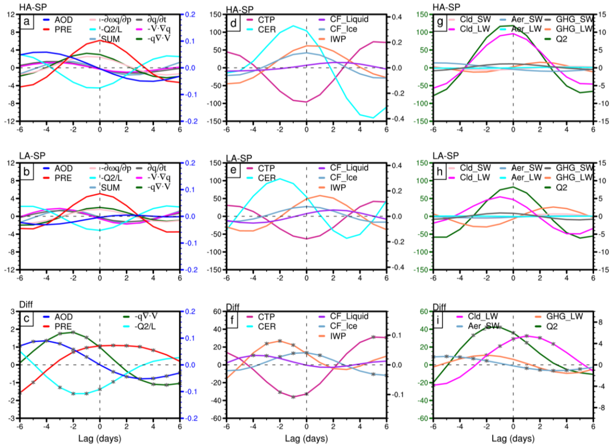
409 Figure 4. As in Fig. 2a, but for the composite evolution of 8–30-day (a) precipitation (red curve; left y-axis, mm d -1 ), 410 AOD (blue curve; right y-axis in blue, unitless), and individual moisture budget terms (various colored curves 411 representing each budget term in Eq. (1); left y-axis, mm d -1 ) associated with HA–SP events. (d, g) As in (a), except that 412 (d) shows the 8–30-day evolution of cloud top pressure (CTP; magenta curve; left y-axis, hPa), ice water path (IWP; 413 orange curve; left y-axis, g m -2 ), cloud droplet effective radius (CER; orange curve; right y-axis, μm), liquid cloud 414 fraction (CF_Liquid; purple curve; right y-axis, unitless), and ice cloud fraction (CF_Ice; light blue curve; right y-axis). 415 Panel (g) presents 8–30-day column-integrated latent heat heating ( Q_2 ; green curve; left y-axis in green, W m -2 ) and 8– 416 30-day radiative budget terms calculated from Eq. (2) (right y-axis, W m -2 ), including longwave/shortwave cloud 417 radiative effects (Cld_LW/Cld_SW; magenta curve/pink curve), longwave/shortwave aerosol direct radiative effects 418 (Aer_LW/Aer_SW; cyan curve/light blue curve), and longwave/shortwave greenhouse gas radiative effects 419 (GHG_LW/GHG_SW; orange curve/gray curve). (b, e, h) and (c, f, i) are similar to (a, d, g), but represent the composite 420 results for LA–SP events and the differences between HA–SP and LA–SP events, respectively. In panels (c) and (i), only 421 terms with statistically significant differences at the 90% confidence level are shown, with significant periods marked 422 by gray asterisks. These results are based on MERRA-2 budget variables and MODIS cloud parameters.
