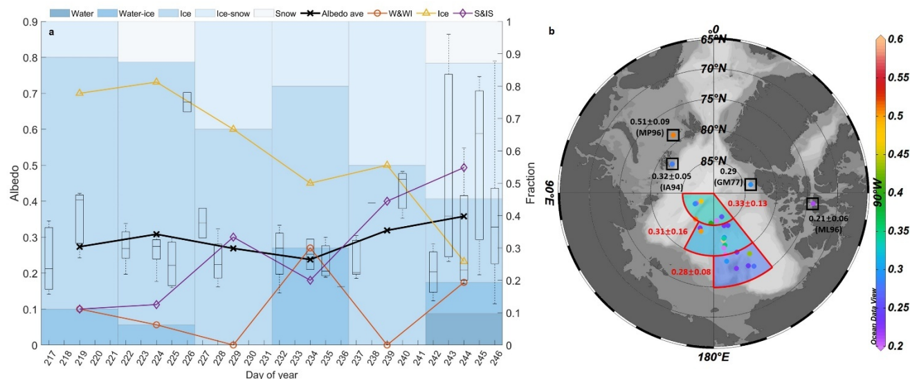
Figure 6: The temporal (a) and spatial (b) distribution of total albedo of melt ponds. In subplot (a), the boxplot represents the albedo of melt ponds observed in certain DOY (day of year), bars represent 5-day average proportions (axis at the right side) of each type of pond, the black solid line is the 5-day average of albedo, dashed lines represent 5-day average of proportions (axis at the right side) of water & water-ice (red) pond, ice (yellow) pond, ice-snow & snow (purple) pond, respectively.
