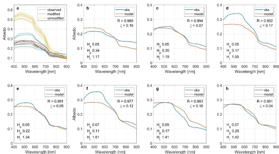
Figure 11: The observed and simulated values of spectral albedo for melt ponds, where (a) shows the observed albedo, and the result of model with and without modification of all ponds. Panels (b)–(h) present the result of each pond separately, where R represents correlation coefficient, \zeta represents relative error, H_s is the ice lid thickness, H_p is the melt pond depth and H_i is the substrate ice thickness.
