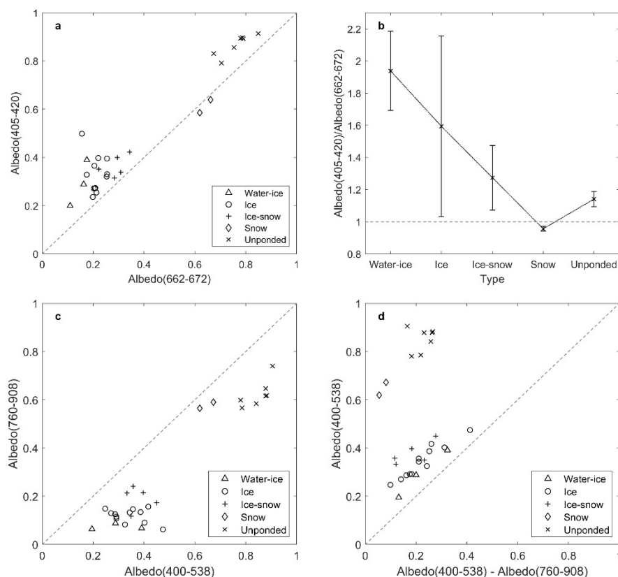
Figure 13: The ratio of spectral albedo between 405–420 nm and 662–672 nm for (a) all ponds and (b) different types, and scatterplots for albedo ratio between different bands following (c) PCA and (d) LinearPolar Algorithm, where numbers in the brackets represent the limits of the integral albedo.
