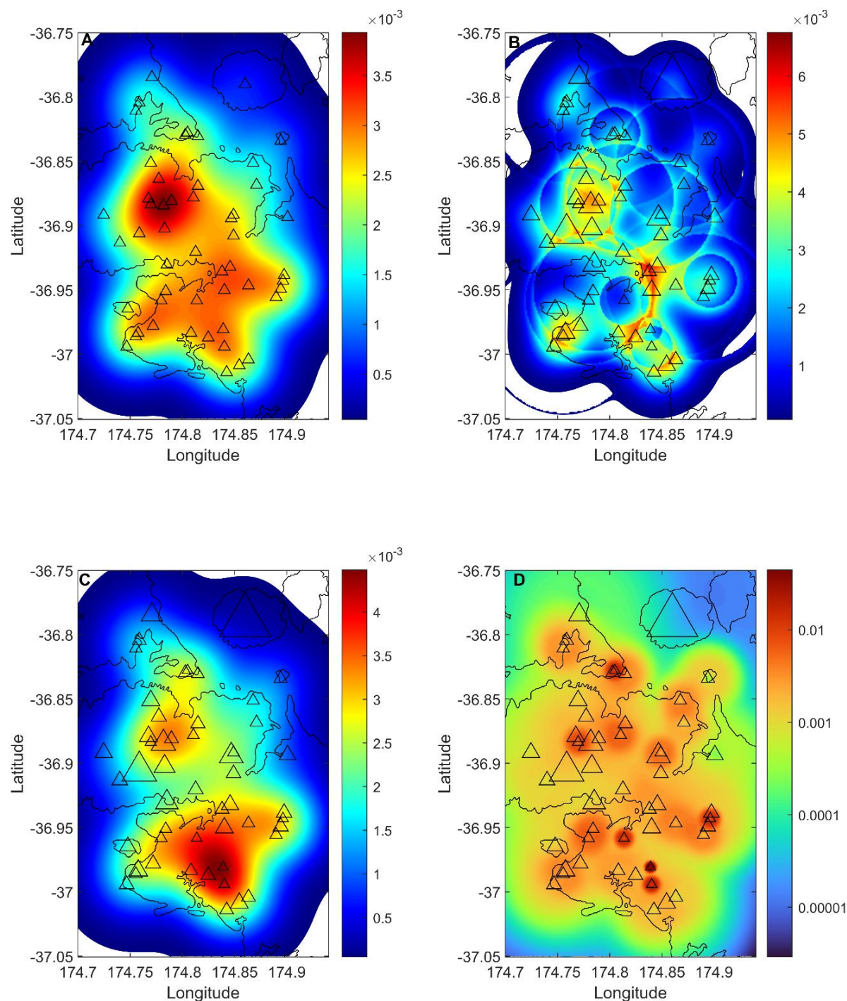
125 Figure 2 Fitted spatial densities to the Auckland Volcanic Field, Aotearoa-New Zealand. A) Isotropic Gaussian (Eq. 2), B) Disk-based depletion (Eq. 6), C) Inverse-volume weighted (Eq. 8), D) Distance-multiplied (Eq. 10). Vent location symbols (triangles) scale with square root of volume (except in A as volume is not considered in the model).
