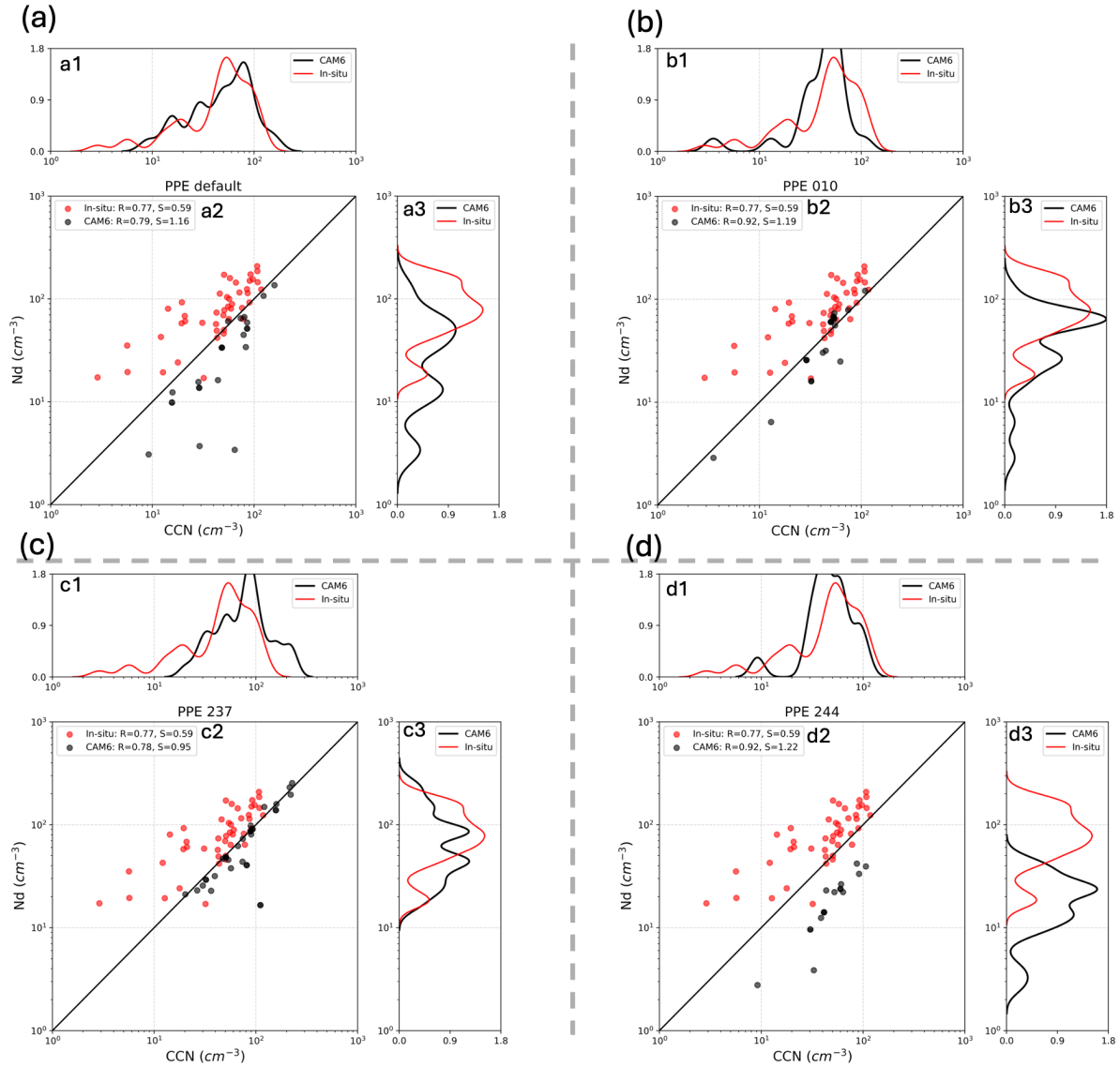
Figure 2. Relationships between SOCRATES CCN and cloud droplet number concentration ( N_d ) from in-situ measurements (red) and CAM6 members (black) from individual flight tracks. Observations are binned into 50 m (altitude) by 2 min (time) bins for each flight. Bin medians are taken for comparison with CAM6 models following McCoy et al. (2021). CAM6 in-cloud N_d is computed as N_d divided by liquid cloud fraction (when cloud fraction \leq 1\% , we set N_d = 0 ). CAM6 PPE CCN and N_d are collocated to observations (50 m \times 2 min bins) by linear interpolation for individual PPE members. PDFs of number concentrations of CCN (top) and cloud droplets (right) for matched binned values occurring for CAM6 (black) and observations (red) are shown. (a) Default CAM6 configuration (i.e., PPE simulation for ensemble member 000), (b) PPE simulation for ensemble member 010, (c) PPE 237, (d) PPE 244.
