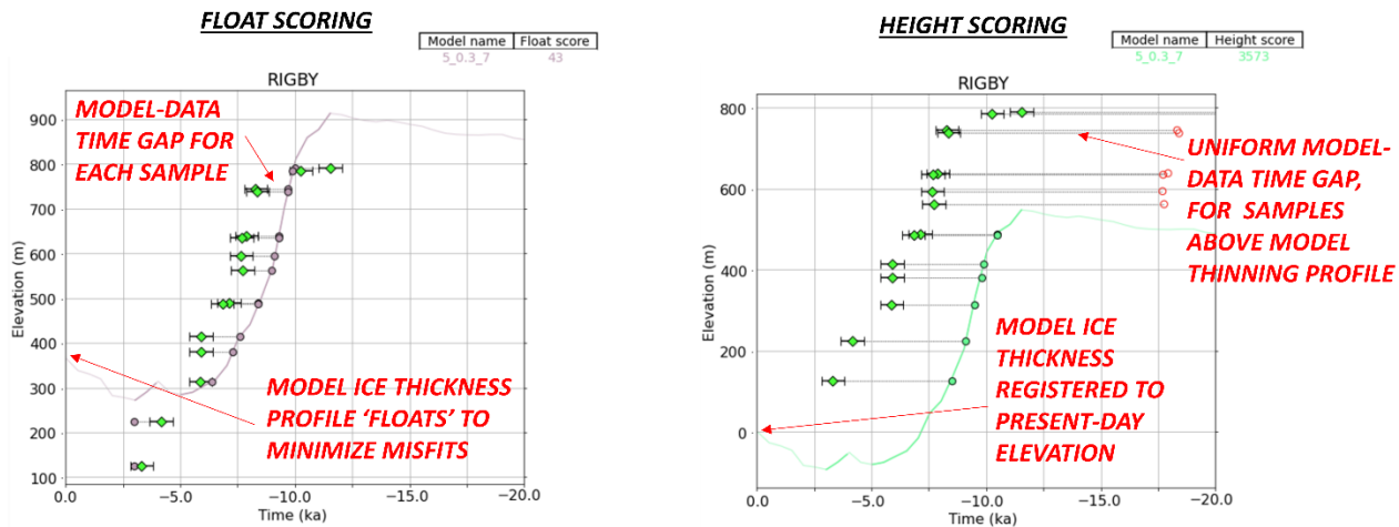
1085 Figure A3: The model-data time gap which is used to calculate sample misfit (Section 4.2.1) is plotted as a horizontal bar for a float scoring (left) or height scoring (right) approach. Samples that fall above the model thinning curve are assigned a uniform time gap \Delta t_u of 10 kyr.
