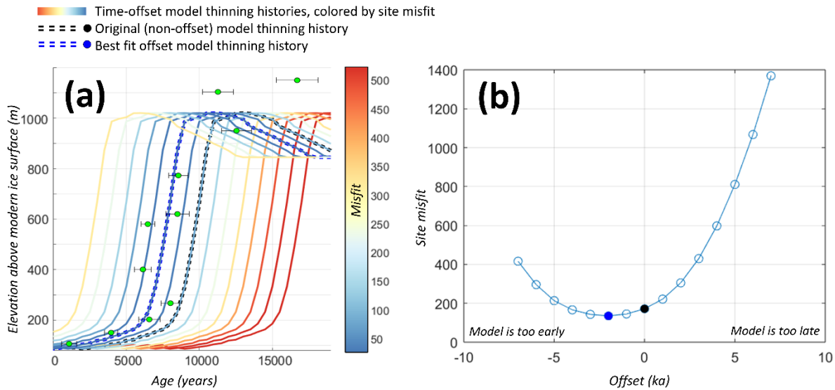
580 Figure 7: Calculating a best-time-offset value at a site. (a) Exposure age samples and model ice thickness profile (dashed black line) from Fig. 6. The model thickness profile is systematically shifted earlier and later via an imposed ‘time offset’; time-offset model thickness profiles are colored by the resulting site misfit. The model thinning curve with the best-time-offset value (-2 kyr) is shown with a dashed red line. This -2 kyr time-offset model thinning curve results in the minimum site misfit (the ‘site best-time-offset misfit’). This process is demonstrated graphically in (b), where the original model thickness profile (offset=0) is shown as a black dot, and the best-time-offset model profile is a red dot.
