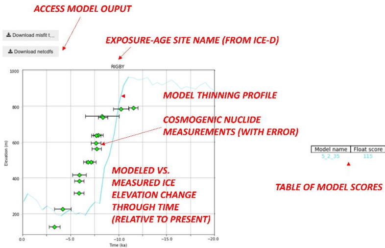
Figure A1: Model thinning at a selected site RIGBY (original data from Spector et al., 2017), compared to the profile of youngest-age-elevation samples at that site. Error bar width denotes the 1\sigma standard deviation of the Monte Carlo youngest age/elevation space. Model-data misfit at each sample is calculated and the sum is tabulated.
