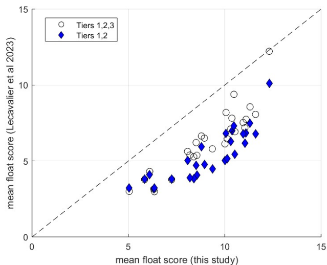
Figure 11: Float misfit model scores for each model -simulation using either the Lecavalier et al. (2023) curated dataset (y-axis) or the ICE-D all-inclusive dataset (x-axis; this study). Blue diamonds indicate model scores calculated using the Lecavalier et al. dataset with both Tier 1 and Tier 2 constraints, following their methodology (30 sites). We also show the impact of scoring models with all three tiers (38 sites).
