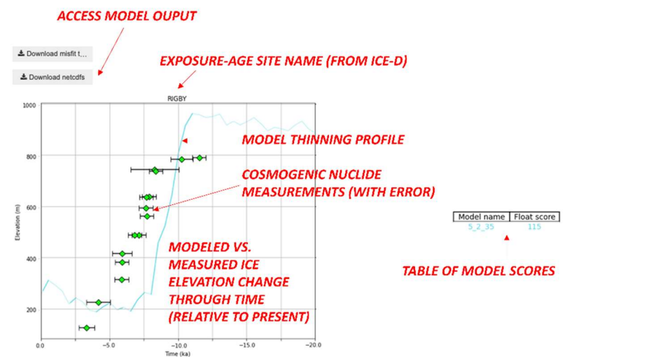
Figure A1: Model thinning at a selected site RIGBY (original data from Spector et al., 2017) , compared to the profile of youngest-age-elevation samples at that site. Error bar width denotes the 1\sigma standard deviation of the Monte Carlo youngest age/elevation space. Model-data misfit at each sample is calculated and the sum is tabulated.
