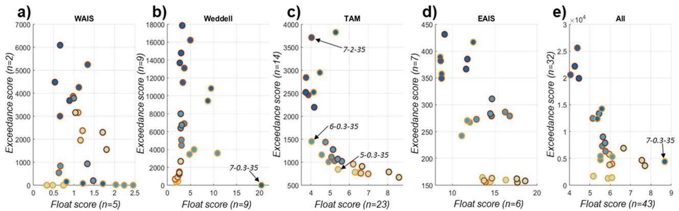
1065 Figure 14: Float misfit scores and exceedance misfit scores by region (WAIS: West Antarctic Ice Sheet; Weddell: Weddell Sea region; TAM: Transantarctic Mountains; EAIS: East Antarctic Ice Sheet margin; regions shown in Fig. 1a). Axis labels indicate the number of sites in each region for both float misfit score and exceedance score metrics. When all regions are considered (e), scores are identical to the results with 2km nested domains shown in Fig. 12. Model simulations referred to in the text are labeled here. Circle color and outline color correspond to parameter value, as in Fig. 12.
