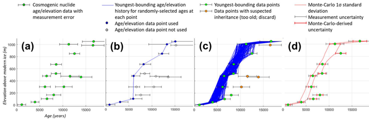
430 Figure 2: (a) Sample illustrative dataset of cosmogenic nuclide measurements collected along an elevation transect, with error bars denoting measurement error. (b) One iteration of our youngest-sample identification scheme (identifying the youngest age/elevation bounding range given randomly varied age/elevation data points within measurement uncertainty). (c) 10,000 Monte Carlo (MC) iterations produce a range of youngest-boundary age/elevation trajectories, and identify all possible youngest data points (green) to
