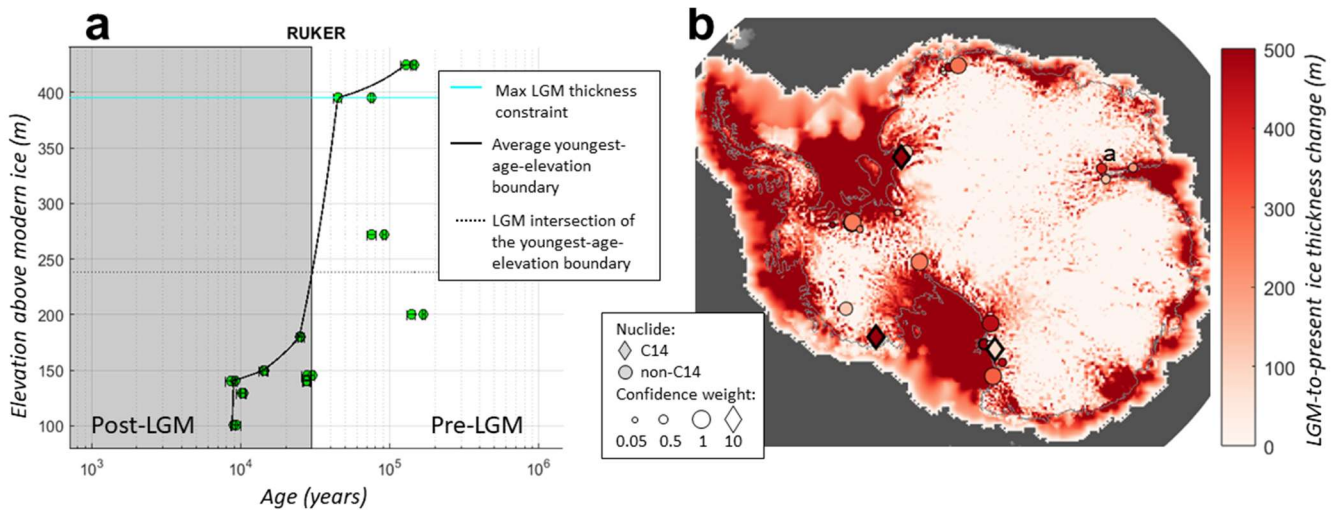
Figure 10: (a) Identifying an LGM maximum ice-thickness-above-present constraint (395 m; cyan line) from a gap between pre- and post-LGM ages at RUKER ( Prince Charles Mountains, Mt. Ruker; original data from White et al., 2011 ). The confidence weighting, based on the total number of samples at the site, is 0.4. (b) Maximum ice thickness constraint data are compared to a model prediction of the same quantity (ice thickness change since the Last Glacial Maximum; shown here from model member 5-0.3-7). Maximum ice thickness constraints are differentiated between ^{14}\text{C} data (diamonds; 3 samples) and non- ^{14}\text{C} nuclides (circles; 29 samples). The size of the circle indicates the confidence weighting, described below, from 0-1. Grey contour denotes the modern grounding line.
