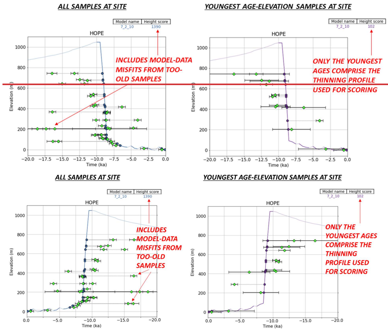
Figure A4: Model scores are calculated by summing the model-data misfit statistic for each sample; therefore, using every measured sample at a selected site (left) produces a worse and less representative model score than selecting and proceeding with model-data comparison using just the youngest-age-elevation-bounding samples (right). Original data from HOPE are also from Spector et al. (2017).
