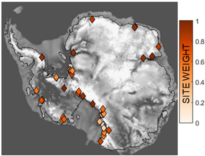
Figure 9: Spatial weights at each exposure age site used for scoring (i.e., with more than 3 samples that span more than 100m of elevation change). Sites are inversely weighted based on the number of nearby sites.
