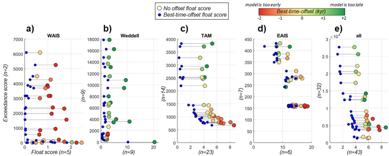
1115 Figure 15: Float misfit scores with no time offset (same as in Fig. 14), compared to the best-time-offset float misfit scores (the minimum possible float misfit score achieved by shifting the model thinning curves by the best-time-offset value). Each regional float misfit score is colored with respect to the best-time-offset value (kyr; averaged across all sites in the region) that produces the minimized best-time-offset float misfit score plotted in blue.
