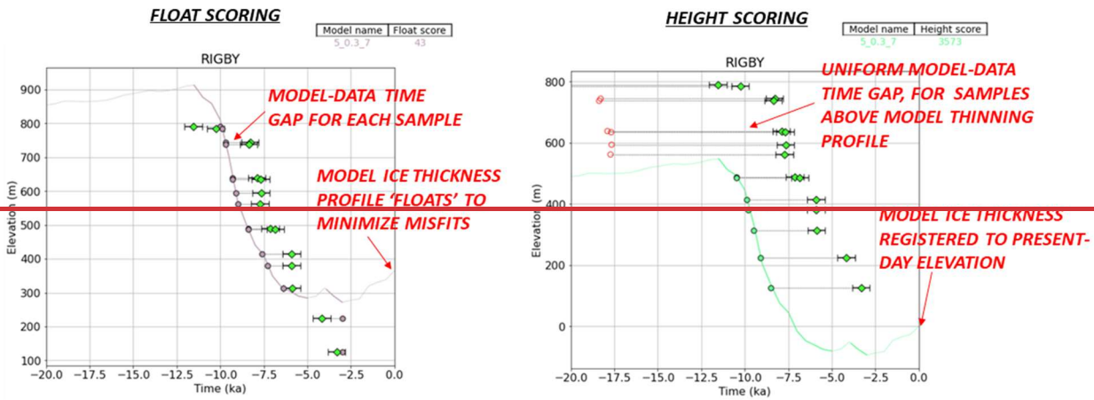
Figure A3: The model-data time gap which is used to calculate site-sample misfit (see Section 43.2.3-1) is plotted as a horizontal bar for a float scoring (left) or height scoring (right) approach. Samples that fall above the model thinning curve are assigned a uniform time gap \Delta t_0 of 10 kyr.
