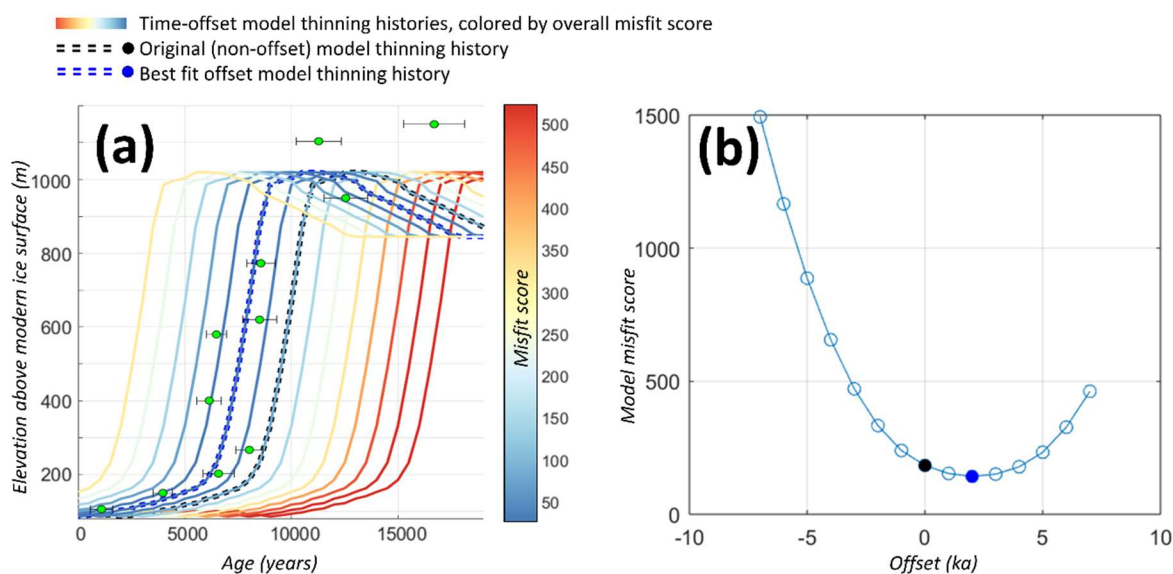
690 Figure 7: Calculating a best-time-offset value at a site. (a) Exposure age samples and model ice thickness profile (dashed black line) from Fig. 6. The model thickness profile is systematically shifted earlier and later via an imposed ‘time offset’; time-offset model thickness profiles are colored by the resulting model/data misfit score. The model thinning curve with the best-time-offset value (-2 kyr) is shown with a dashed red line. This -2 kyr time-offset model thinning curve results in the minimum misfit score (the best- time-offset misfit score). This process is demonstrated graphically in (b), where the original model thickness profile (offset=0) is 695 shown as a black dot, and the best-time-offset model profile is a red dot.
