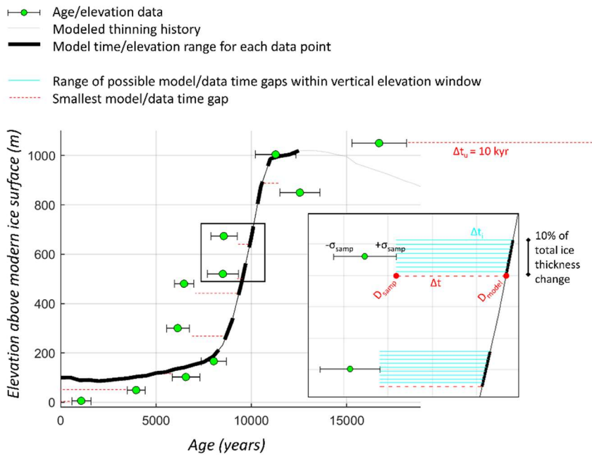
625 Figure 57: Graphical illustration of model/data misfit components (exposure age samples and compared to a ‘floating’ ice thickness history from Fig. 5 ). The thicker lines denote the model vertical window (elevation range for assessing model thickness history against each data sample). The model vertical window is defined as 10% of LGM-to-present ice thickness change; in this case, \pm 47\text{m} . \Delta t_u , the smallest time gap for each sample, is identified with a red dashed line.
