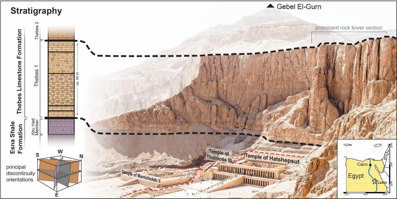
100 Figure 1: Topographic and geological setting of the Mortuary Temple of Hatshepsut within Deir el-Bahari (view towards west). In 105 terms of geo-mechanics, the brittle Thebes Limestone on thinly layered Esna Shales (Dupuis et al., 2011) represent a typical “brittle on weak” structure.
