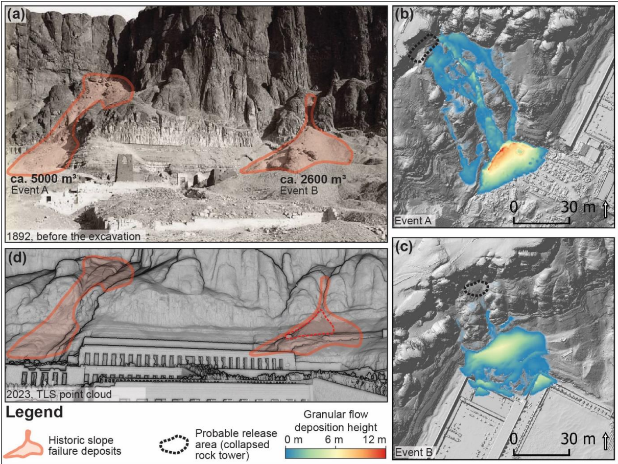
Figure 5: a) Earliest historic photograph of the Temple of Hatshepsut before the first major excavation (Neville, 1894) shows two distinct deposits that indicate previous rock slope failure. b), c) Results of the dry flow simulations for historic rock tower collapses
