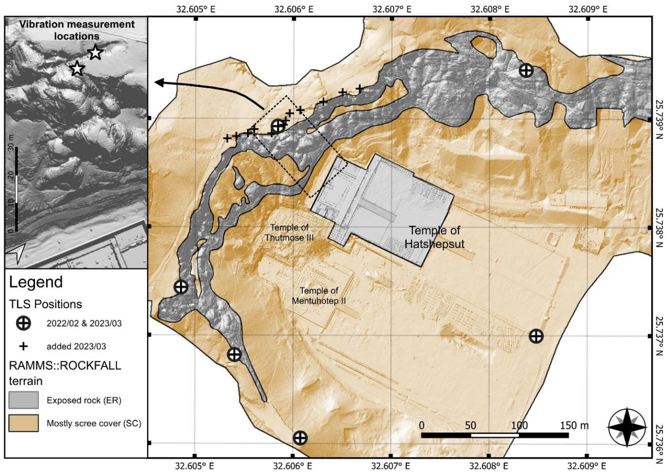
Figure 2: Map of the Deir EL-Bahari with the Mortuary Temple of Hatshepsut mortuary temple including repeated TLS Scan Positions, vibration measurements, and spatial extent of terrain for rockfall simulations.
