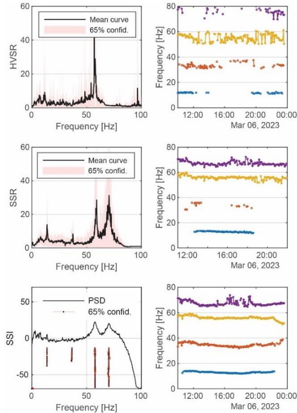
415 Figure 6: Extracted ambient seismic vibration frequencies of the rock towers above the temple of Hatshepsut based on HVSR, SSR, and SSI techniques.
