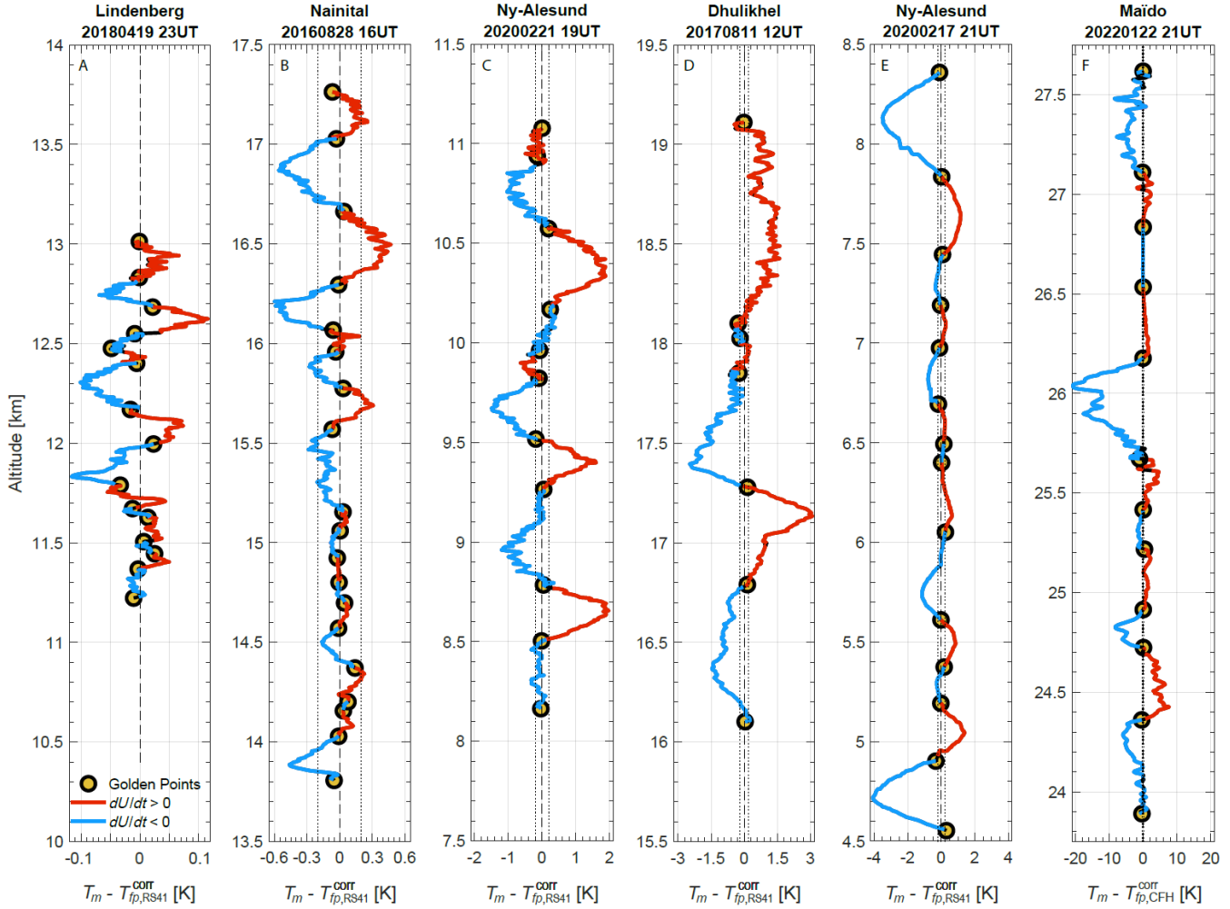
847 Figure 7: Four-kilometer slabs of various soundings with CFH, sorted according to nonequilibrium error. Slabs start after the 848 second cycle (at T_{fp} = -53^{\circ}\text{C} ) and end at the hygropause. We use the higher reliability of RS41 below the hygropause to correct 849 CFH in panels A-E. An exception is panel F, which shows the CFH measurement in the core of the Hunga Tonga-Hunga 850 Ha'apai plume, for which CFH was corrected assuming a background mixing ratio of 5 ppmv. Panels A and F will be discussed 851 in detail in the following subsections.
