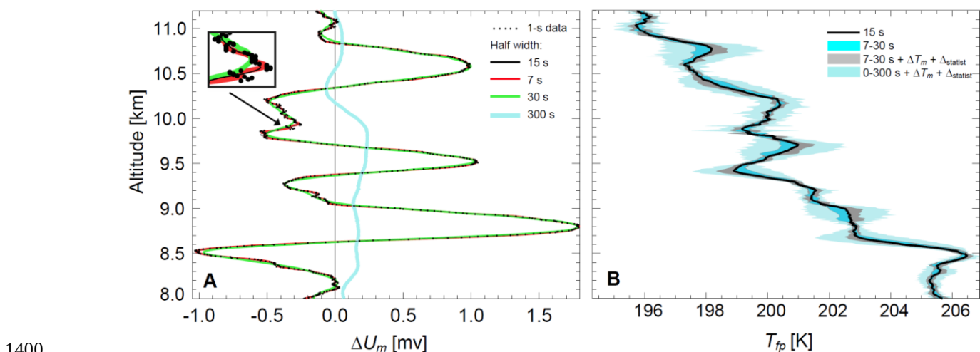
1401 Figure D2: Sensitivity of non-equilibrium correction using different smoothing widths for a sounding in Ny-Ålesund on 21 1402 Feb. 2020 (same as Fig. 6). (A) Reflectance smoothed by using a Savitzky-Golay filter with different widths ranging from 7 1403 s to 300 s. (B) The uncertainty of the non-equilibrium corrected CFH frost points. Black line: 15-s filtering. Dark blue shading: 1404 range of smoothing of reflectance with 7 s, 15 s and 30 s Savitzky-Golay filter; grey shading: range of smoothing of reflectance 1405 with 7-15-30 s Savitzky-Golay plus mirror temperature uncertainty and statistical uncertainty (similarly to NDACC, see also 1406 Figure 6 and Eq. 9); light blue shading: 0-7-15-30-300 s Savitzky-Golay plus mirror temperature and statistical uncertainties.
