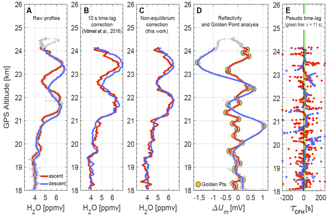
Figure 5. Water vapor mixing ratios during ascent and descent measured by CFH on 20 May 2014 22UT over Lindenberg (serial 2L3407 with FW 6.40 on LI133). (A) Raw signal of H 2 O mixing ratio ascent with smoothed mirror temperature (using a second-order, 15 s half-width, Savitzky-Golay filter) versus GPS altitude (air temperature and air pressure from iMet1-RSB radiosonde, serial 14246; telemetry software (Strato 9.54) applied an offset of 2.9 hPa to the pressure measurement). (B) Time-lag corrected mixing ratio profiles, using an e-folding time constant of 10 s, as in Vömel et al. (2016). (C) Nonequilibrium corrected mixing ratio profiles, using an effective sensitivity A = 800 V/s for ascent and A = 2300 V/s for descent. (D) Raw signal of mirror reflectance profiles (smoothed with a second-order, here in the stratosphere with a Savitzky-Golay filter with 21 s half width instead the standard 15 s) and associated Golden Points. (E) Ascent and descent profiles of the pseudo time lag constant \tau_{\text{noneq}} , i.e. the mathematical time constant that would be required to reproduce the atmospheric frost point profile after applying the nonequilibrium correction. The median of all \tau_{\text{noneq}} is 11 s (green line), i.e. close to the e-folding time constant of 10 s used for the time-lag treatment in panel (B).
