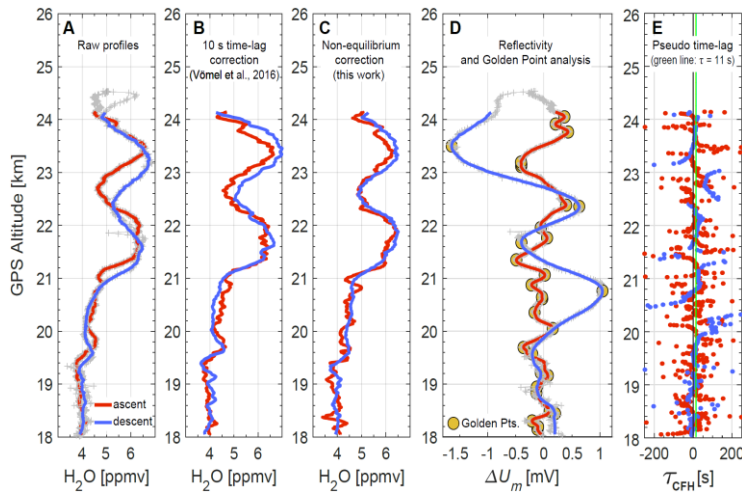
731 Figure 5. Water vapor mixing ratios during ascent and descent measured by CFH on 20 May 2014 22UT over Lindenberg 732 (serial 2L3407 with FW 6.40 on LI133). (A) Raw signal of \text{H}_2\text{O} mixing ratio ascent with smoothed mirror temperature (using 733 a second-order, 15 s half-width, Savitzky-Golay filter) versus GPS altitude (air temperature and air pressure from iMet1-RSB 734 radiosonde, serial 14246; telemetry software (Strato 9.54) applied an offset of 2.9 hPa to the pressure measurement). (B) 735 Time-lag corrected mixing ratio profiles, using an e-folding time constant of 10 s, as in Vömel et al. (2016). (C) 736 Nonequilibrium corrected mixing ratio profiles, using an effective sensitivity A = 800 V/s for ascent and A = 2300 V/s for 737 descent. (D) Raw signal of mirror reflectance profiles (smoothed with a second-order, here in the stratosphere with a Savitzky- 738 Golay filter with 21 s half width instead of the standard 15 s) and associated Golden Points. (E) Ascent and descent profiles of 739 the pseudo time lag constant \tau_{\text{noneq}} , i.e. the mathematical time constant that would be required to reproduce the atmospheric 740 frost point profile after applying the nonequilibrium correction. The median of all \tau_{\text{noneq}} is 11 s (green line), i.e. close to the e- 741 folding time constant of 10 s used for the time-lag treatment in panel (B).
