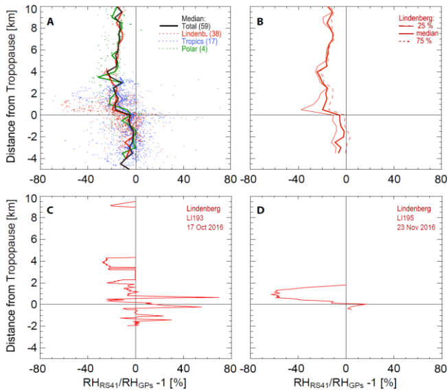
Figure B1: Comparison of (RH_{RS41} - RH_{GP})/RH_{GP} of the RS41 manufacturer product with 3042 Golden Points (GP) of CFH. The GP have an uncertainty of 0.2 K in the frost point corresponding to an uncertainty of less than 3.5% in the value of RH. (A) Scatter plot of (RH_{RS41} - RH_{GP})/RH_{GP} for 3042 GP during 59 RS41-CFH tandem soundings after the second cleaning cycle (i.e., second ice film). These are the soundings listed in Table A1, excluding flights with apparent contamination problems. Launch sites are color coded. Lines show median values in 500-m steps. (B) 25%, 50%, and 75% percentiles for the 38 soundings from Lindenberg, showing the reduced RS41 data quality with a pronounced dry bias directly above the tropopause and larger sonde-to-sonde variability. (C+D) Two examples of Lindenberg soundings illustrating the RS41 sonde-to-sonde-variability.
