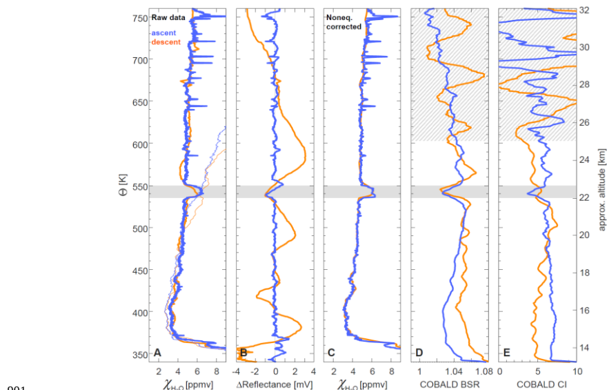
Figure 8: Balloon sounding on 19 April 2018 in Lindenberg (52.21°N, 14.12°E) showing remarkable \text{H}_2\text{O} and particle backscatter anomalies (gray shading) in measurements by CFH and the backscatter sonde COBALD during ascent (blue lines) and descent (orange lines). (A) \text{H}_2\text{O} mixing ratios retrieved from CFH raw data. Thin lines show the RS41 data (Vaisala product). In this sounding, RS41 lost sensitivity above potential temperature level 500 K ( \approx 20.5 km altitude). (B) CFH reflectance signal. (C) Nonequilibrium correction of the CFH mixing ratio, making the blue ascent and the orange descent lines almost coincide. (D) COBALD backscatter ratio ( \text{BSR}_{455\text{nm}} ) at 455 nm, with 10 K (potential temperature) moving average. (E) COBALD Color Index \text{CI} = (\text{BSR}_{940\text{nm}} - 1) / (\text{BSR}_{455\text{nm}} - 1) , also with 10 K moving average. Hatched area: above 600 K the backscatter signal is too noisy during descent, possibly due to excessive swinging of the dangling payload.
