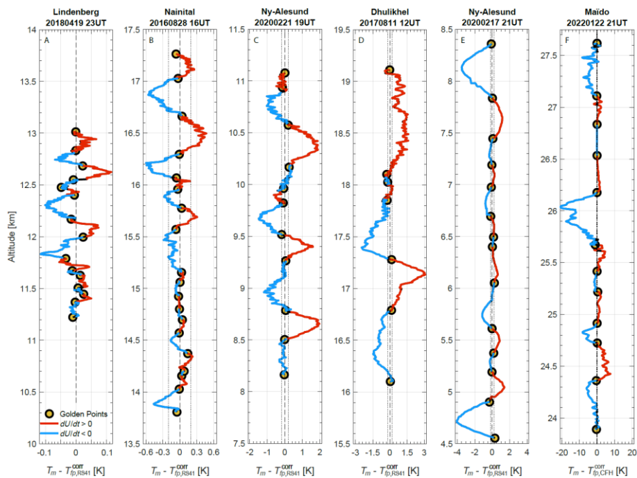
888 Figure 7: Four-kilometer slabs of various soundings with CFH, sorted according to nonequilibrium error. Slabs start after the 889 second cycle (at T_{fp} = -53^{\circ}\text{C} ) and end at the hygropause. We use the higher reliability of RS41 below the hygropause to correct 890 CFH in panels A-E. An exception is panel F, which shows the CFH measurement in the core of the Hunga Tonga-Hunga 891 Ha'apai plume, for which CFH was corrected assuming a background mixing ratio of 5 ppmv. Panels A and F will be discussed 892 in detail in the following subsections.
