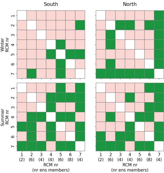
355 Figure 8 Matrix of significant differences in temperature (tas) between RCM-based sub-ensembles within RCM17, for southern Sweden (South, region C in Fig. 1) and northern Sweden (North, region D in Fig. 1.). Green colours indicate significant differences. Numbers indicate sub-ensemble numbers, with the number of members in parenthesis.
