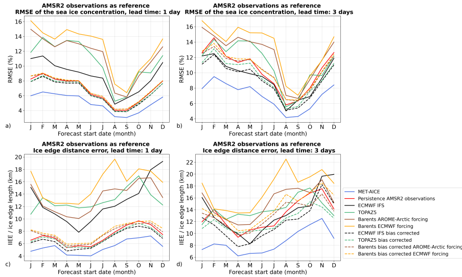
Figure 7. Seasonal variability of the performances of MET-AICE, ECMWF IFS, TOPAZ5, and Barents-2.5 for 1-day and 3-day lead times using AMSR2 observations as reference during the period April 2024 - March 2025. a, b) Root mean square error (RMSE) of the sea ice concentration. c, d) Evaluation of the ice edge position (defined by the 10 % sea ice concentration contour). The forecasts are evaluated over the shared domain between MET-AICE and Barents-2.5.
