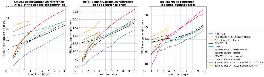
Figure 5. Performances of MET-AICE, ECMWF IFS, TOPAZ5 and Barents-2.5 during the period April 2024 - March 2025 over the shared domain between MET-AICE and Barents-2.5. a) Root mean square error (RMSE) of the sea ice concentration using AMSR2 observations as reference. b) Evaluation of the ice edge position (defined by the 10 % sea ice concentration contour) using AMSR2 observations as reference. c) Evaluation of the ice edge position using the ice charts as reference.
