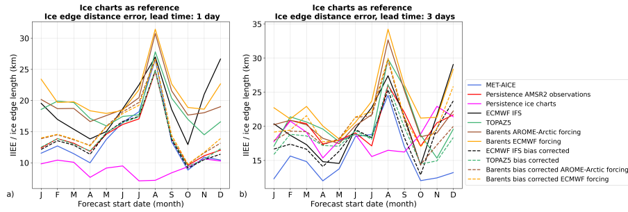
Figure 8. Seasonal variability of the performances of MET-AICE, ECMWF IFS, TOPAZ5, and Barents-2.5 for 1-day (a) and 3-day (b) lead times using the ice charts as reference during the period April 2024 - March 2025. The forecasts are evaluated over the shared domain between MET-AICE and Barents-2.5.
