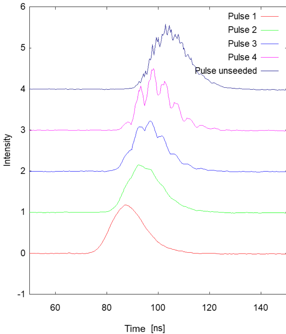
Laser impulse shape
