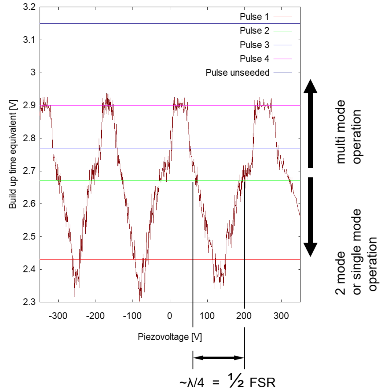
Length dependence of the pulse build up time
