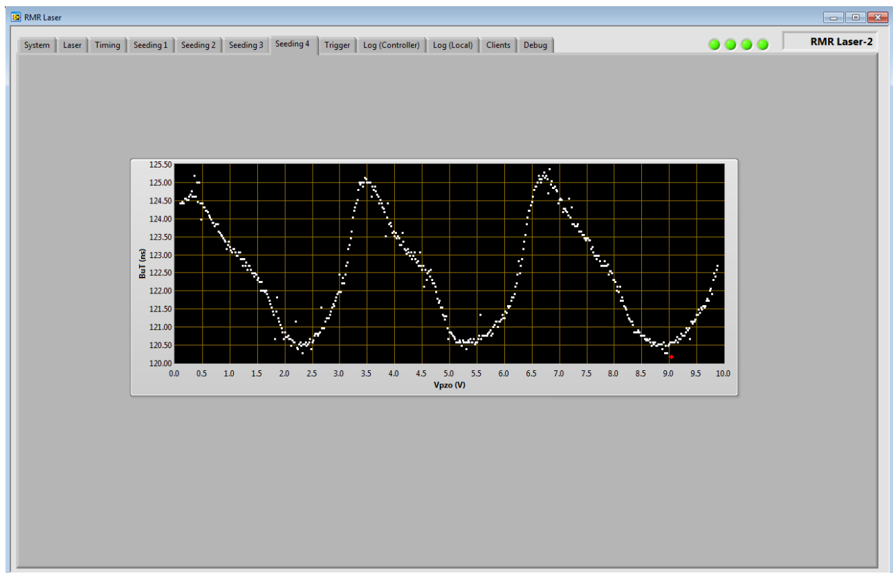
Fig. 2: Scan of the piezo over several resonance conditions of the power laser cavity (pulse build-up time as function of piezo position in terms of control voltage).
