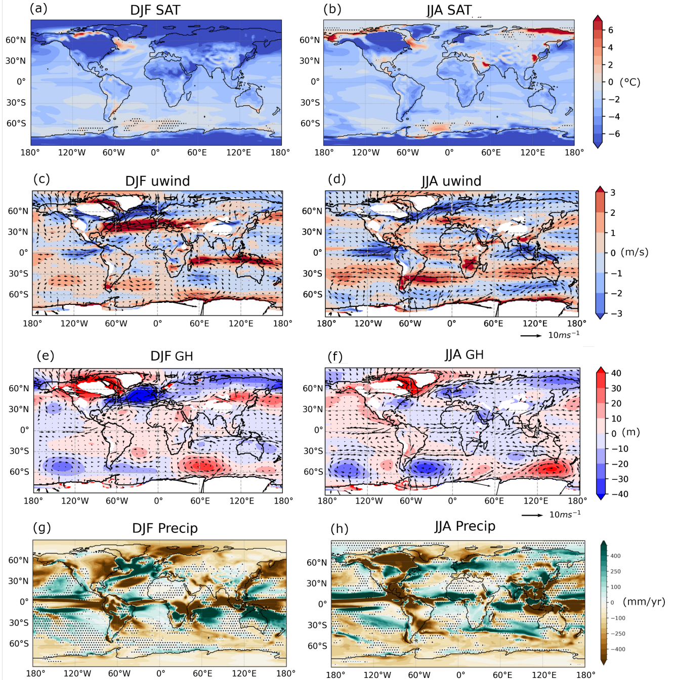
Figure 3. Anomalies between 49ka-full and PI for (a,b) SAT ( ^{\circ}\text{C} ), (c,d) zonal winds at 850 hPa (m/s) overlaid with 850 hPa wind vector anomalies (m/s), (e,f) geopotential height at 850 hPa (m) with zonal mean removed and overlaid with 850 hPa wind vector anomalies (m/s), and (g,h) precipitation (mm/yr) during (left) DJF and (right) JJA. Stippling in subpanels (a,b) and (g,h) indicates non-significant changes based on a Student's t-test at the 95% confidence level. The white space in subpanels c–f indicates the ice mask at the 850 hPa level.
