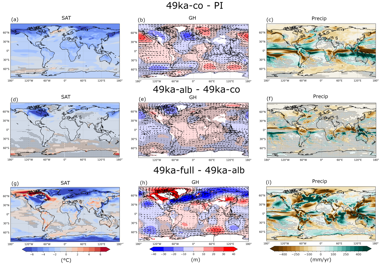
Figure 6. DJF (a,d,g) SAT (°C), (b,e,h) geopotential height (m) overlaid with wind vector anomalies at 850 hPa and precipitation (mm/yr) anomalies for (a-c) 49ka-co minus PI, (d-f) 49ka-alb minus 49ka-co, (g-i) and 49ka-full minus 49ka-alb. Stippling indicates non-significant changes based on a Student's t-test at the 95% confidence level. The white space in subpanels (b,e,h) indicates the ice mask at the 850 hPa level.
