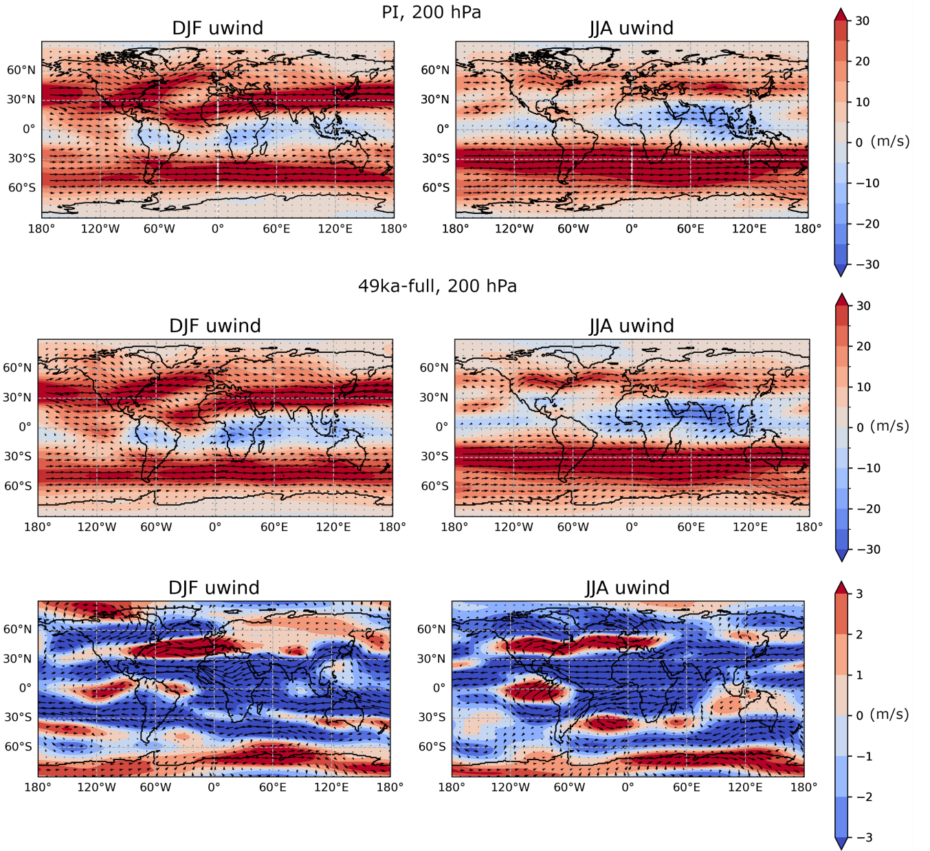
Figure A4. Zonal winds at 200 hPa (m/s) overlaid with 200 hPa wind vectors (m/s) in (left) DJF and (right) JJA for (top) PI and (middle) 49ka-full, and (bottom) 49ka-full minus PI ( overlaid with 200 hPa wind vectors anomalies (m/s) ).
