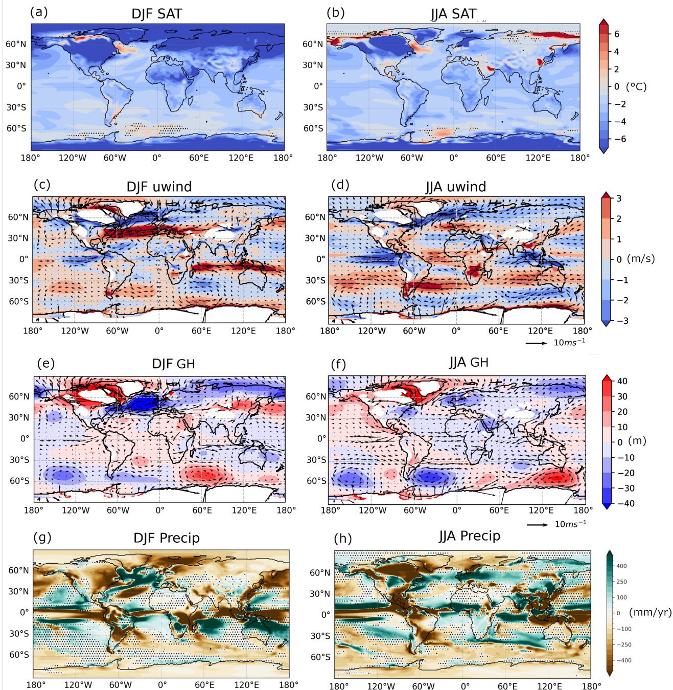
Figure 3. Anomalies between 49ka-full and PI for (a,b) SAT (°C), (c,d) zonal winds at 850 hPa (m/s) overlaid with 850 hPa wind vectors (m/s), (e,f) geopotential height at 850 hPa (m) with zonal mean removed and overlaid with 850 hPa wind vectors (m/s), and (g,h) precipitation (mm/yr) during (left) DJF and (right) JJA. Stippling in subpanels (g,a,b) and (g,h) indicates non-significant changes based on a Student's t-test at the 95% confidence level. The white space in subpanels c-f indicates the ice mask at the 850 hPa level.
