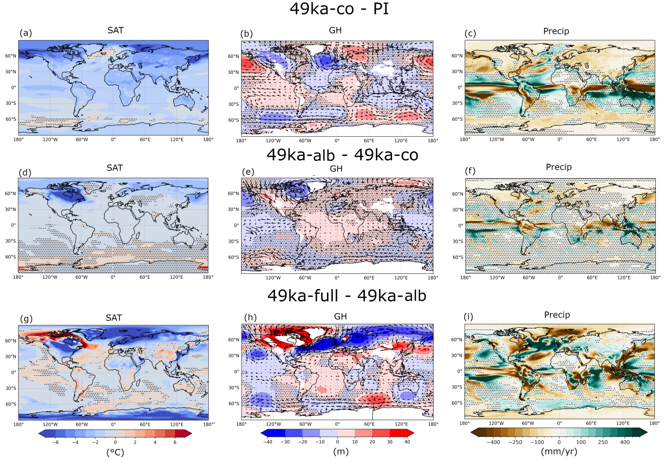
Figure 6. DJF (a,d,g) SAT (°C), (b,e,h) geopotential height (m) overlaid with winds-wind vector anomalies at 850 hPa and precipitation (mm/yr) anomalies for (a-c) 49ka-co minus PI, (d-f) 49ka-alb minus 49ka-co, (g-i) and 49ka-full minus 49ka-alb. Stippling indicates non-significant changes based on a Student's t-test at the 95% confidence level . The white space in subpanels (b,e,h) indicates the ice mask at the 850 hPa level .
