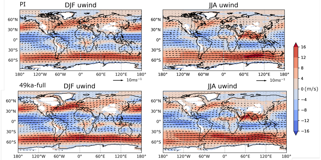
Figure 5. Zonal winds at 850 hPa (m/s) overlaid with 850 hPa wind vectors (m/s) in (left) DJF and (right) JJA for (top) PI and (bottom) 49ka-full. The white space the ice mask at the 850 hPa level.
