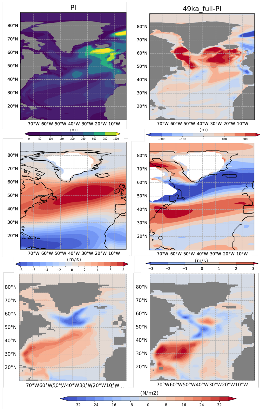
Figure A3. (top) Winter mixed layer depth (m), (middle) Zonal winds (m/s) at 850 hPa, and (bottom) North Atlantic gyre strength ( calculated from the barotropic streamfunction , N/m 2 ) for (left) PI and (right) 49ka-full compared to PI. The white areas in the middle panel mark grid cells with continental ice, and for the 49ka-full simulation, continental outlines are shown based on the adjusted land-sea mask.
