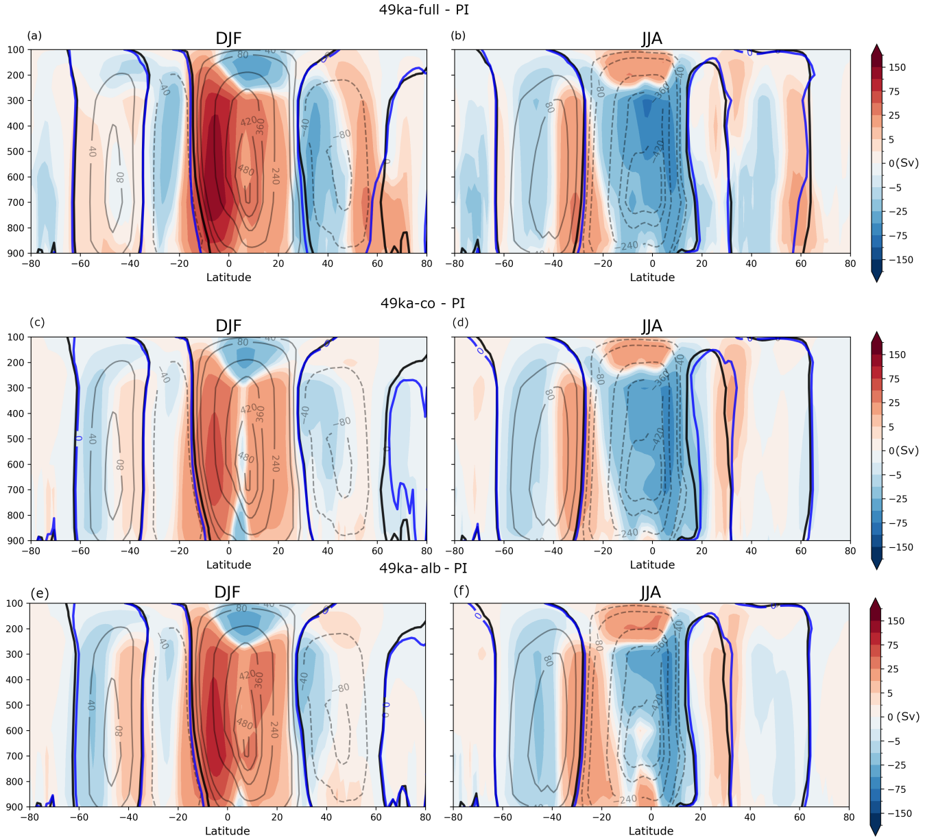
Figure 8. Atmospheric mass streamfunction (Sv) anomalies (shading) between (a,b) 49ka-full and PI, (c,d) 49ka-ic 49ka-co and PI, and (e,f) 49ka-ice 49ka-alb and PI, for (left) DJF and (right) JJA. Contours (solid=positive; dashed=negative) are PI (black) absolute streamfunction values. The thick black and blue lines represent the zero contour for PI and 49ka experiments, respectively.
