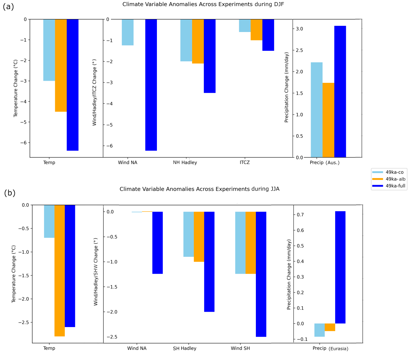
Figure 9. Summary of key atmospheric responses across experiments. (Top) DJF anomalies: (left) NH SAT (°C); (middle) latitudinal shifts (°) in westerlies averaged over the North Atlantic (80°W:0°E, 30°N:90°N), NH Hadley cell's southern edge, and globally averaged ITCZ position; and (right) northern Australian precipitation (116°E:152°E, 25°S:12°S, mm/day). (Bottom) JJA anomalies: (left) NH SAT (°C); (middle) latitudinal shifts (°) in westerlies averaged over the North Atlantic, SH Hadley cell's southern edge (°), westerlies averaged over the SH; and (right) precipitation changes over Eurasia (60°W:80°E, 48°N:60°N). Results are shown for the 49ka-co (cyan), 49ka-ice (orange), and 49ka-full (blue) experiments, with all values presented as anomalies relative to PI. Negative values in latitudinal shifts indicate an equatorward shift.
