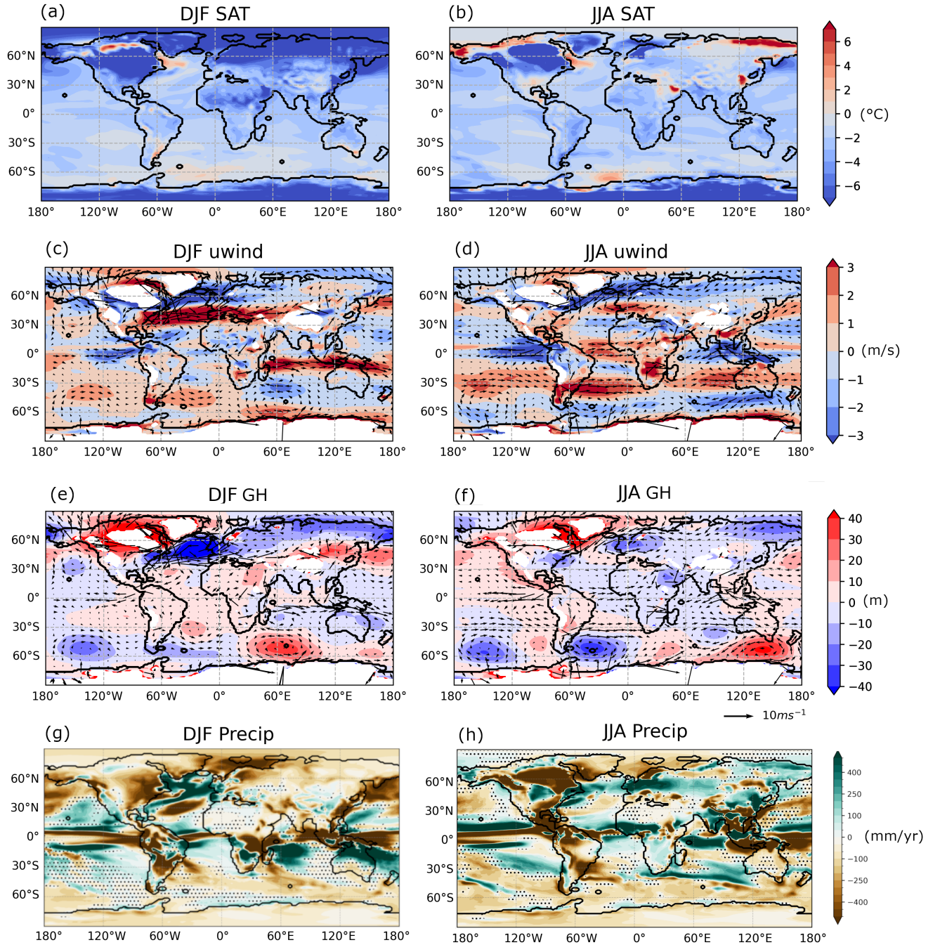
Figure 3. Anomalies between 49ka-full and PI for (a,b) SAT (°C), (c,d) zonal winds at 850 hPa (m/s) overlaid with wind vectors ( m/s ), (e,f) geopotential height at 850 hPa (m) with zonal mean removed and overlaid with wind vectors (m/s) , and (g,h) precipitation (mm/yr) anomalies between 49ka-full and PI during (left) DJF and (right) JJA. Stippling in subpanels (g) and (h) indicates significant-non-significant changes based on a Student's t-test at 95% significance-confidence level.
