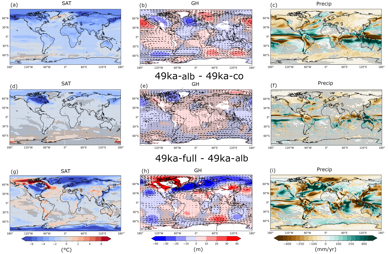
Figure 6. DJF (a,d,g) SAT (°C), (b,e,h) geopotential height (m) overlaid with winds at 850 hPa and precipitation (mm/yr) anomalies between for (a-c) 49ka-co minus PI, (d-f) 49ka-ice-49ka-alb minus 49ka-co, (g-i) and 49ka-full minus 49ka-ice-49ka-alb . Stippling indicates significant non-significant changes based on a Student's t-test at 95% significance-confidence level.
