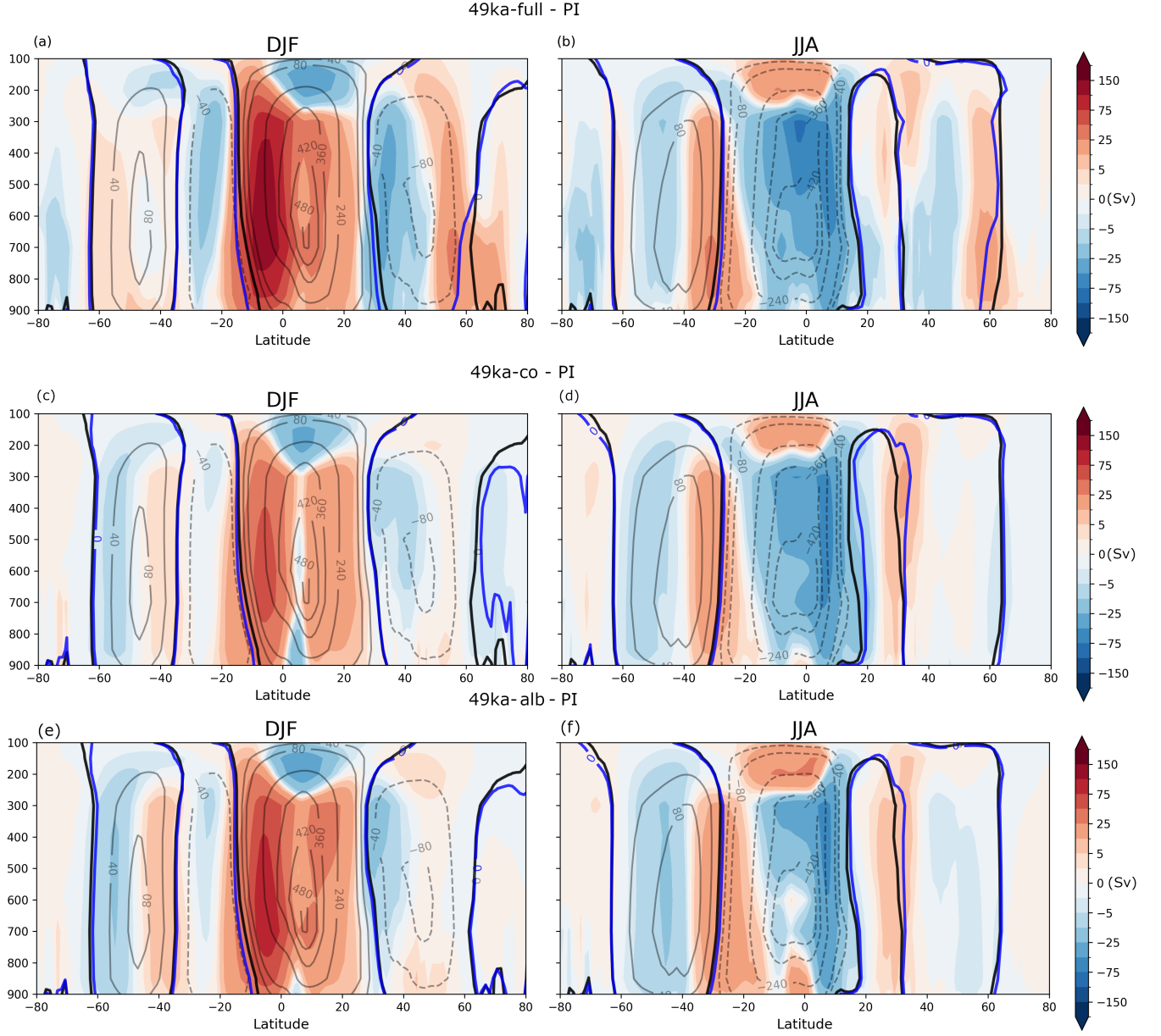
Figure 8. Atmospheric mass streamfunction (Sv) anomalies (shading) between (a,b) 49ka-full and PI, (c,d) 49ka-co and PI, and (e,f) 49ka-alb and PI, for (a) DJF and (b) JJA. Contours (solid=positive; dashed=negative) are PI (black) absolute streamfunction values. The thick black and blue lines represent the zero contour for PI and 49ka experiments, respectively.
