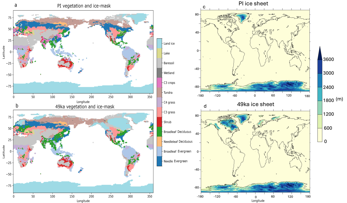
Figure 1. (a,b) Vegetation and ice mask changes at 49 ka compared to PI. The color indicates the dominant Plant Functional Type (PFT) per of each grid cell. (c,d) Ice sheet thickness (m) and extent from (Gowan et al., 2021) for PI and 49 ka (represented by 52.5 ka as described in the text)
