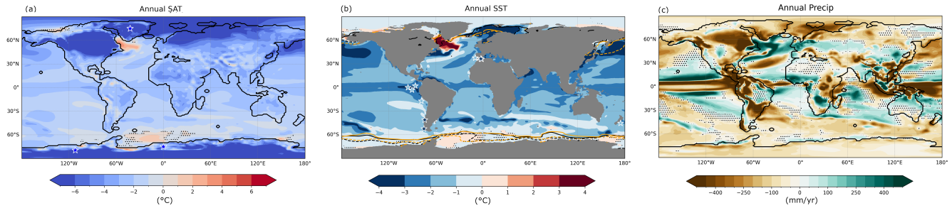
Figure 2. Annual mean anomalies of surface air temperature (SAT), sea surface temperature (SST), and precipitation anomalies for 49 ka climate (exp 49ka-full) compared to PI. Contours are show seasonal mean 15% ocean-sea ice concentration for (orange) 49 ka and (black) PI during DJF (dashed) and JJA (solid). Stippling in subpanel (c) indicates significant-non-significant changes based on a Student's t-test at 95% significancee-confidence level. Stars in subpanels (a) and (b) indicate qualitative estimates of the changes between Greenland Interstadial (GI 13) and PI climate, as inferred from the proxy records (MDO1-2444, ODP-977A, MD95-2043, MD01-2443, MD95-2042 (Martrat et al., 2007) ; ODP-1233 (Kaiser et al., 2005); TR163-19 (Lea et al., 2000); RC13-110 (Feldberg and Mix, 2003); ODP846B (Martínez et al., 2003) ; TG-7 (Calvo et al., 2001); MD97-2120 (Pahnke et al., 2003); MD07-3128 (Caniupán et al., 2011); EPICA Dronning Maud Land (EPICA community members, 2006); WAIS (WAIS Divide Project Members, 2015); NGRIP (Huber et al., 2006; Kindler et al., 2014); SO188-17286-1 (Lauterbach et al., 2020). Dark (light) blue colors represent much colder (slightly colder) climate.
