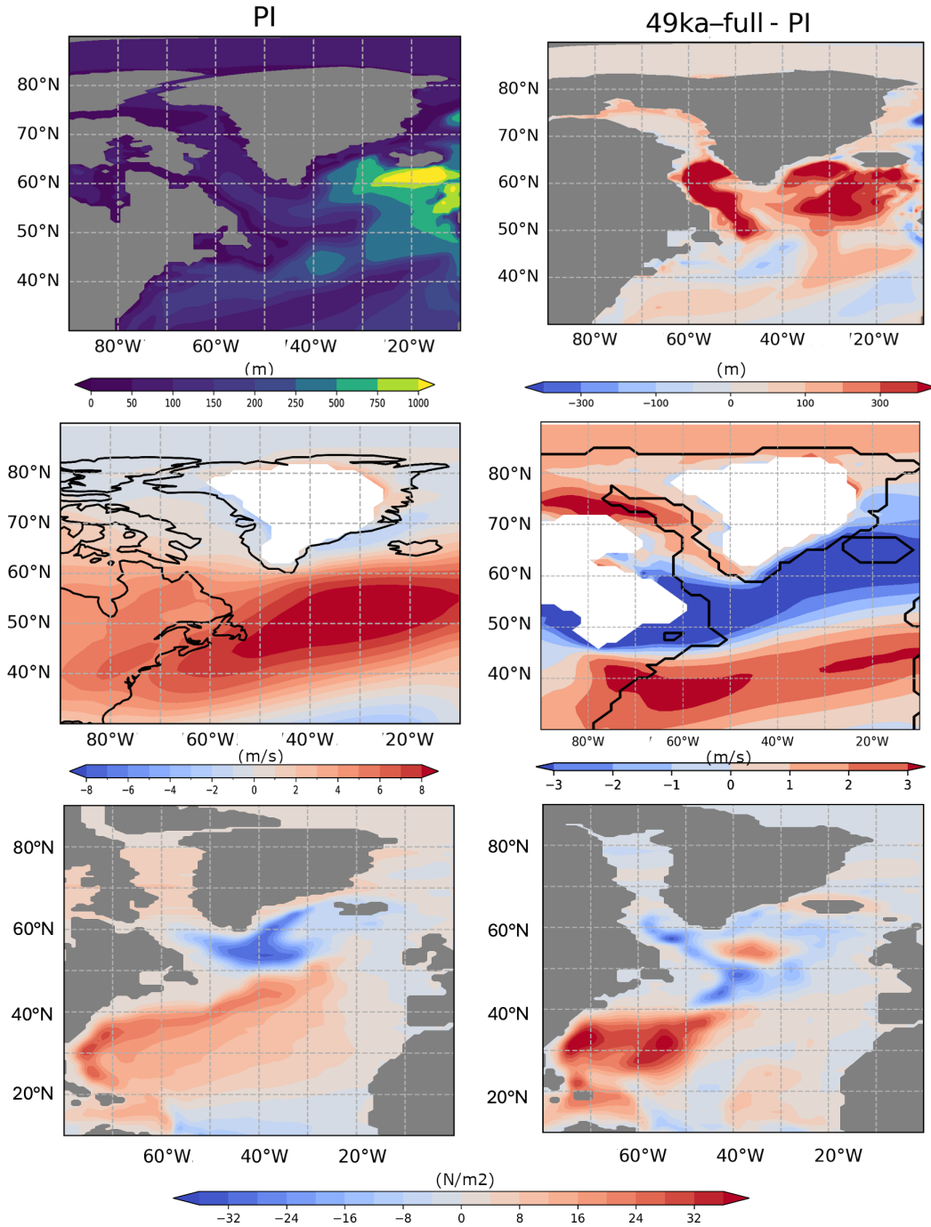
Figure A3. (top) Winter mixed layer depth (m), (centremiddle) Zonal winds (m/s) at 850 hPa, and (bottom) North Atlantic gyre strength (N/m2) for (left) PI and (right) 49ka-49ka-full compared to PI. The white areas in the middle panel mark grid cells with continental ice, and for the 49ka-full simulation, continental outlines are shown based on the adjusted land-sea mask.
