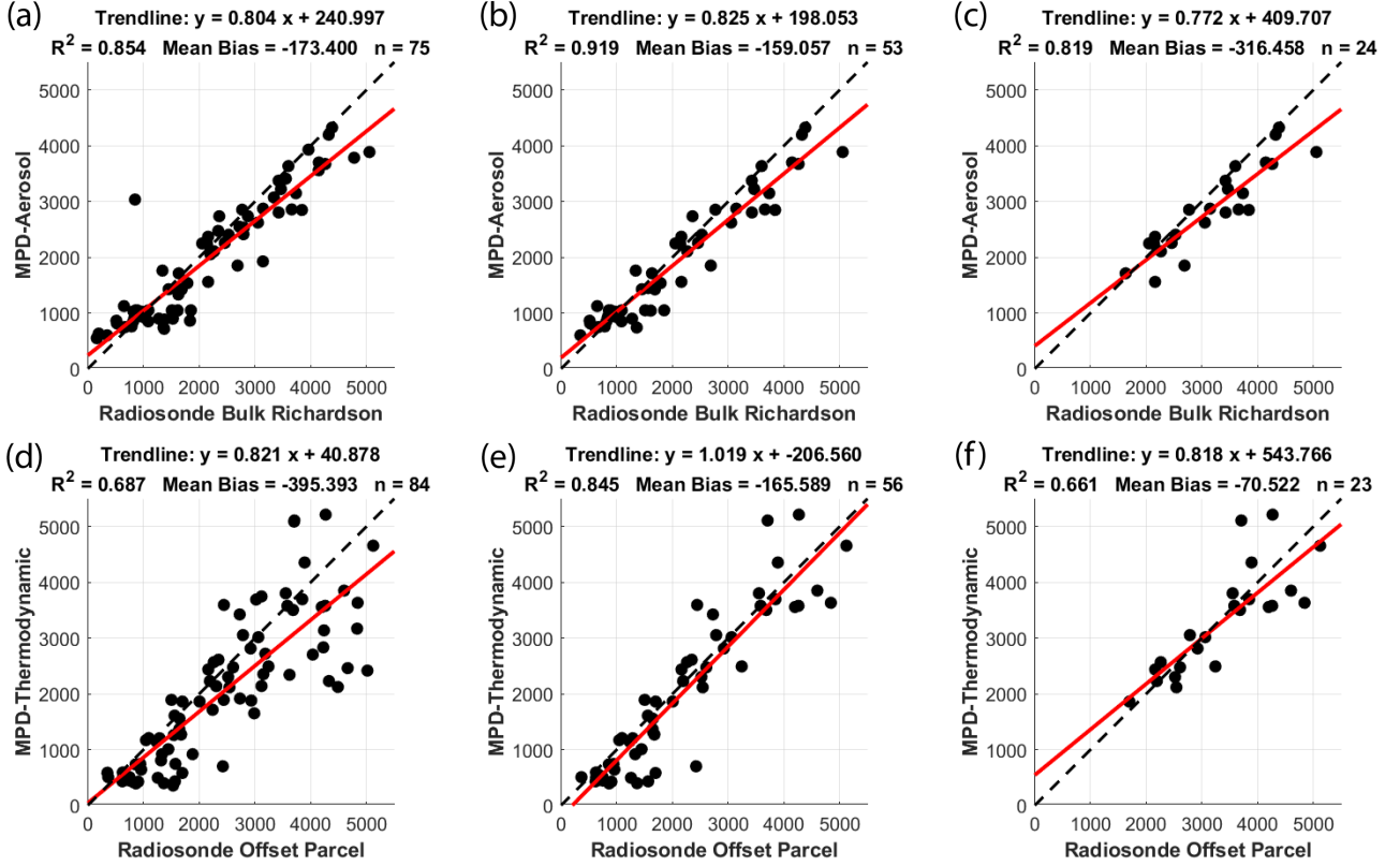
Figure 4. Comparison of MPD-derived MLH retrievals with radiosonde-based retrievals (all values in meters AGL). Panels (a)–(c) show MPD-aerosol retrievals compared with radiosonde bulk Richardson retrievals under different conditions: (a) all conditions, (b) clear-sky conditions, and (c) clear-sky conditions at 22:00 UTC (15:00 local). Panels (d)–(f) show MPD-thermodynamic retrievals compared with radiosonde offset parcel retrievals under (d) all conditions, (e) clear-sky conditions, and (f) clear-sky conditions at 22:00 UTC. The dashed black line indicates 1:1 agreement, and the solid red line shows the linear regression fit.
