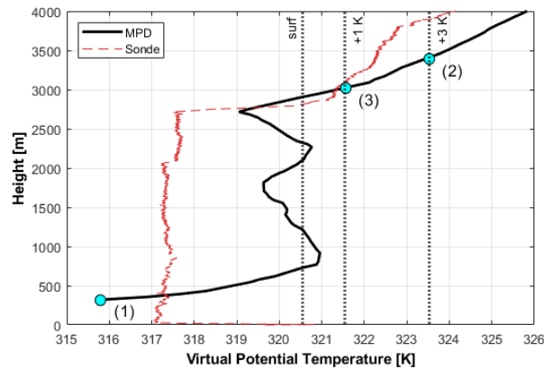
Figure B1. Example virtual potential temperature profiles from the MPD (black) and radiosonde (red dashed line, shown for reference). Vertical dotted lines indicate the surface value ( \theta_{v,surf} ), the +1 K offset, and the +3 K top limiter. The algorithm starts at the lowest available level (1), searches upward to the +3 K intersection (2), then searches downward to the first level at or below the +1 K offset (3). The MLH is diagnosed as the last level before (3). Cyan circles mark the three reference points: (1) lowest available level, (2) first +3 K intersection, and (3) first level at or below +1 K in the downward search.
