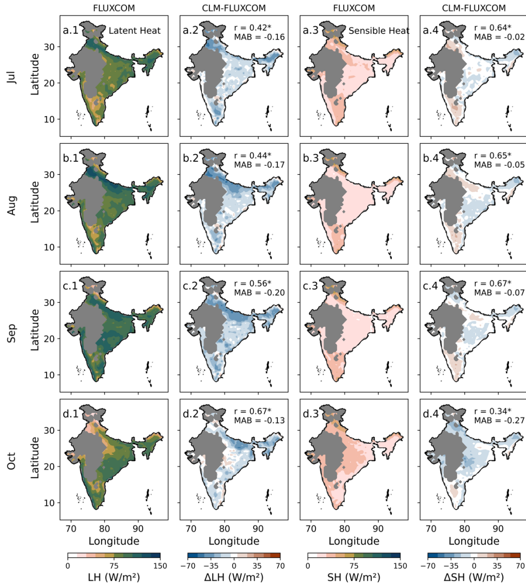
Figure S1: Comparison of monthly water and energy fluxes simulated by CLM5 CTRL run against the FLUXCOM data during the rice growing season, July to October. The area shown here is a region with more than 10% of the land area covered by rice. The second and fourth columns show the difference between CLM5 and FLUXCOM latent and sensible heat, respectively. The monthly mean fluxes over the period 1970-2014 are shown here. Pearson r in the plots is tested for significance, and values that are significant have an asterisk ‘*’.
