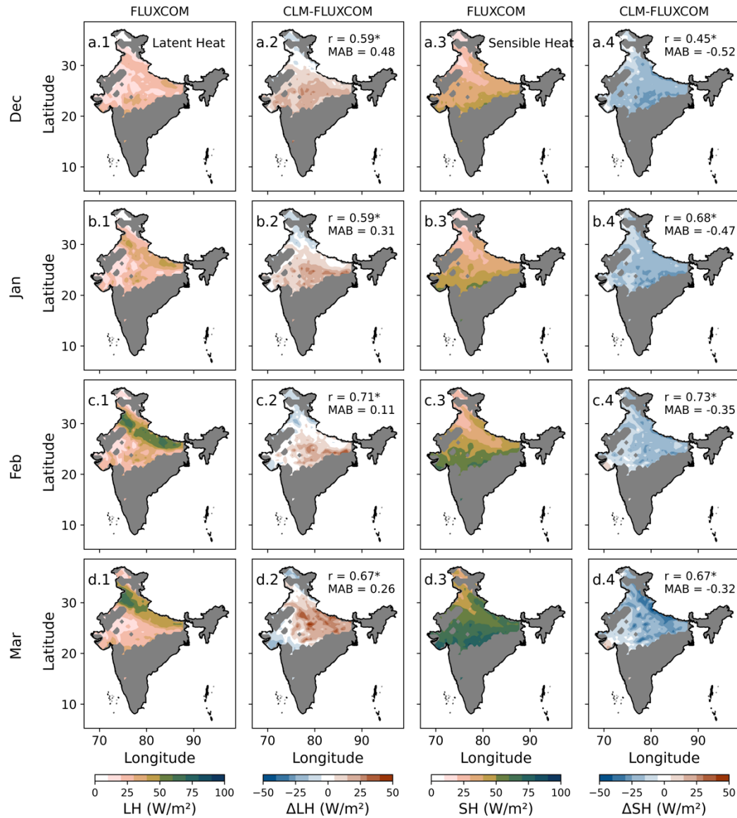
Figure S2: Comparison of monthly water and energy fluxes simulated by CLM5 CTRL run against the FLUXCOM data during the wheat growing season, December to March. The area shown here is a region with more than 10% of the land area covered by wheat. The second and fourth columns show the difference between CLM5 and FLUXCOM latent and sensible heat, respectively. The monthly mean fluxes over the period 1970-2014 are shown here. Pearson r in the plots is tested for significance, and values that are significant have an asterisk “*”.
