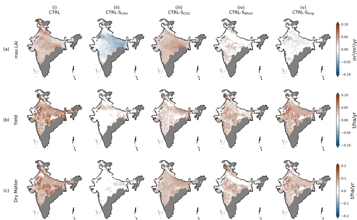
Figure S3: Spatial trend observed in (a) max. LAI, (b) Yield, and (c) Dry Matter of wheat-growing regions in the (i) CTRL simulation. (ii) to (v) shows the impact of each driver. Regions stippled implies the trend is statistically significant at p < 0.05 .
