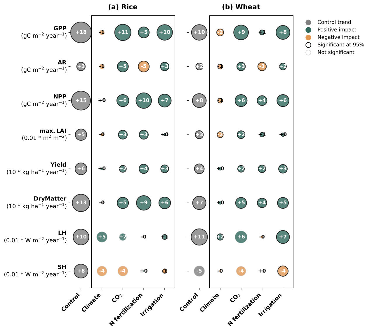
Figure 6: Attribution of long-term trends in carbon fluxes, crop variables, and surface energy and water fluxes for (a) rice and (b) wheat agroecosystems. Grey bubbles show linear trends (1971–2015) in carbon fluxes (GPP, AR, and NPP), crop variables (max. LAI, yield, and dry matter), latent heat flux (LH), and sensible heat flux (SH) from the CLM5 control (CTRL) simulation. Colored bubbles within the rectangular boxes represent the contributions of individual drivers: climate, CO 2 concentration, nitrogen fertilisation, and irrigation (trend of CLM5_CTRL – CLM5_Sdriver). Bubble size is proportional to the magnitude of the trend, with green and red indicating positive and negative contributions, respectively. Bubbles outlined with an edge denote trends or driver impacts that are statistically significant at the 95 % confidence level ( p < 0.05 ).
