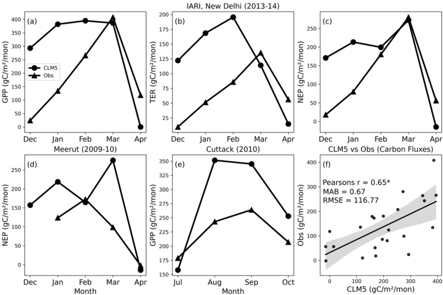
Figure 2: Comparing CLM5 carbon fluxes against observations of (a, b, and c) wheat cropland at IARI, New Delhi, from a study by Reddy et al. (2023), (d) wheat cropland at Meerut, from a study by Patel et al. (2011), (e) rice cropland at Cuttack from Bhattacharya et al. (2013), and (f) scatter plot of all monthly mean carbon flux observations against the monthly mean carbon fluxes from CLM5. The “*” on Pearson r 280 in panel (f) signifies the statistical significance at p<0.001 . The solid black line in (f) is the linear regression, and the shaded region is the 95% confidence interval.
