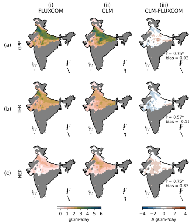
330 Figure 5: Spatial plots of (a) GPP, (b) TER, and (c) NEP from (i) FLUXCOM, (ii) CLM5 over the Indian region, and (iii) the difference between the CLM5 and FLUXCOM data. All plots are for the wheat-growing regions (grid cells with more than 10% of land area covered by wheat crop) and the mean of the growing season (December to March). The ‘*’ over the r value shows a significant correlation at p < 0.01 .
