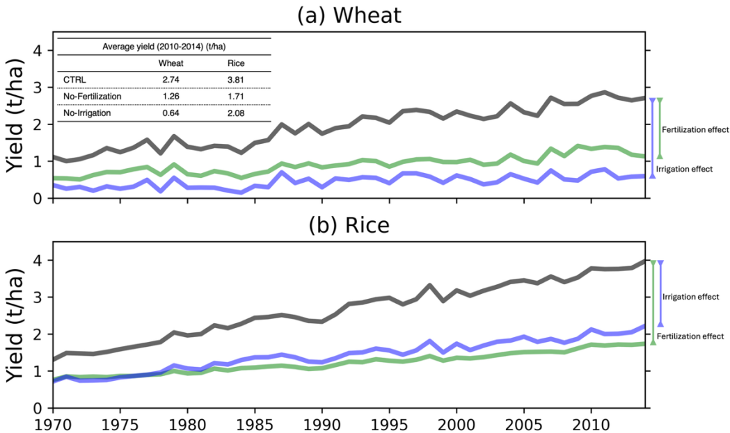
Figure 7: Impact of management drivers on crop yield of (a) wheat and (b) rice. Inlet table shows the average yield in the period 2010-14 for wheat and rice in the CLM5_CTRL simulation, CLM5_SNFert, and CLM5_SIrrig.
