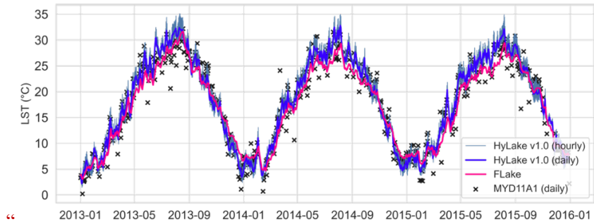
Figure S8: Time series of daily grid-average LST on Lake Chaohu derived from MYD11A1, FLake simulation, and HyLake v1.0 from 2013 to 2015. HyLake v1.0 provides daily and hourly simulations.” (Figure S8 in Supplementary materials)
