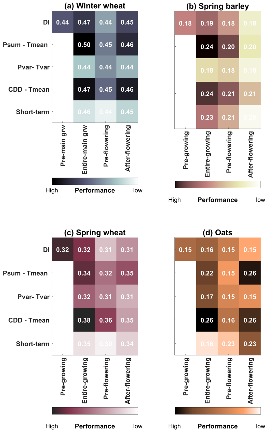
320 Figure 3: Performance of statistical models for yields differing in explanatory variables and period, for four crops (a) winter wheat (b) spring barley (c) spring wheat and (d) oats. Performance is assessed based on the AIC. The darker the color the lower the AIC and hence the higher the performance. Values in each cell indicate the corresponding
