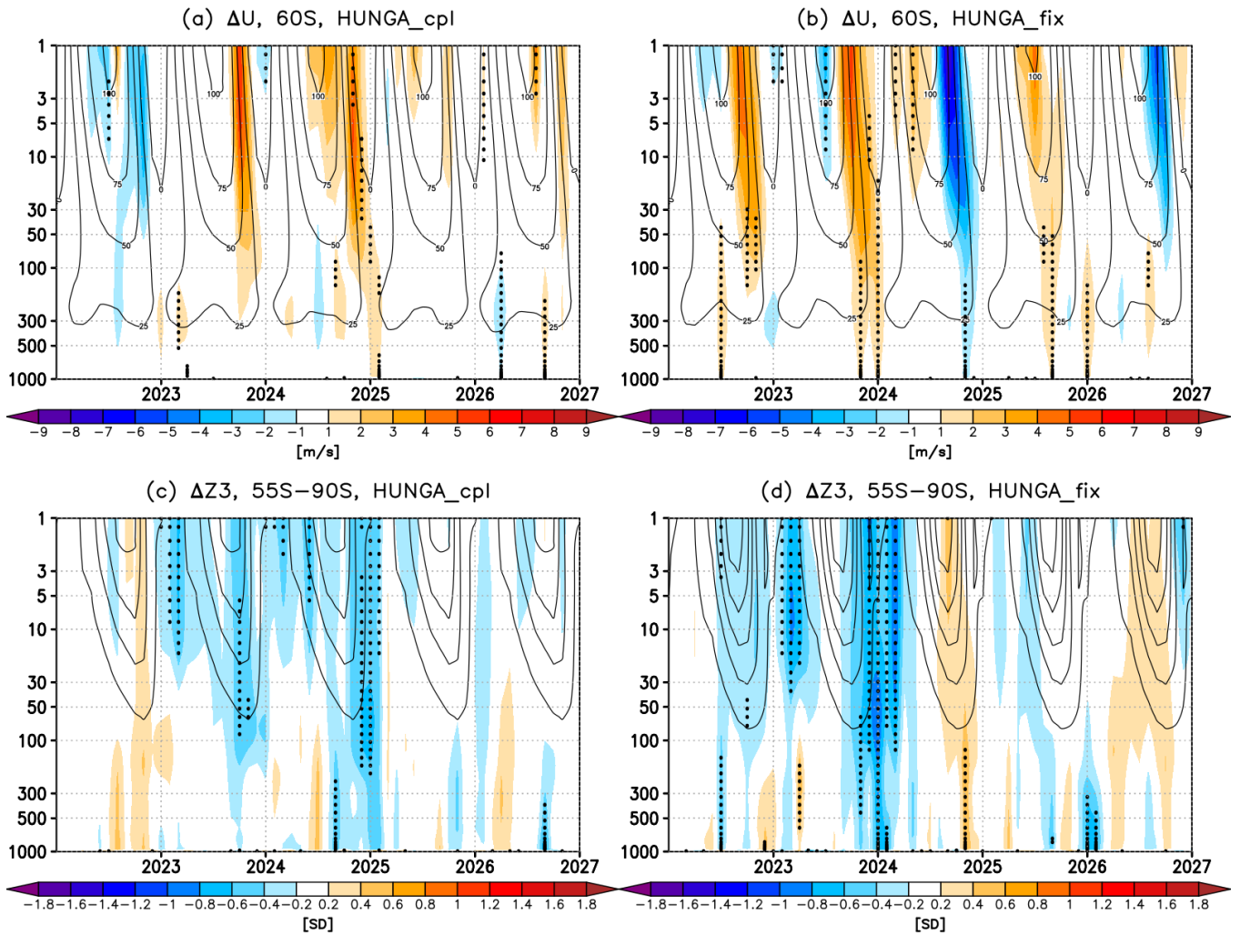
395 Figure 10. Evolution of the SH polar vortex. Shading: Timeseries of changes in (a-b) zonal wind at 60°S [in units of m/s] and (c-d) geopotential height [in units of standard deviations] averaged over the Antarctic polar cap (55°S-90°S) between the forced simulation and the control. The left panels are for the coupled ocean simulations and the right panels are for the atmosphere-only simulations. Stippling denotes regions where the response is statistically significant (defined as in Fig. 1).
