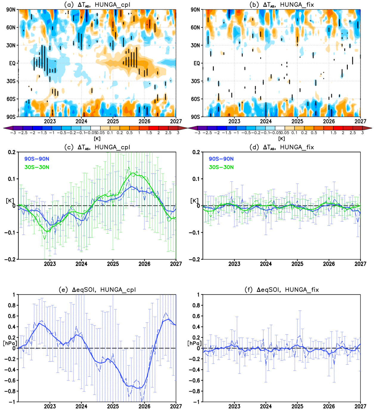
220 Figure 4. Time series of changes in (a-b) zonal mean near-surface air temperature, (c-d) global and tropical mean near-surface air temperature, and (e-f) the eqSOI index between the forced simulation and the control in the coupled ocean (left) and atmosphere-only (right) simulations. Dashed lines in (c-f) indicate ensemble mean changes and solid lines their 5-month running means. Error bars in (c-f) denote confidence intervals of the ensemble mean changes ( \pm 2 standard errors).
