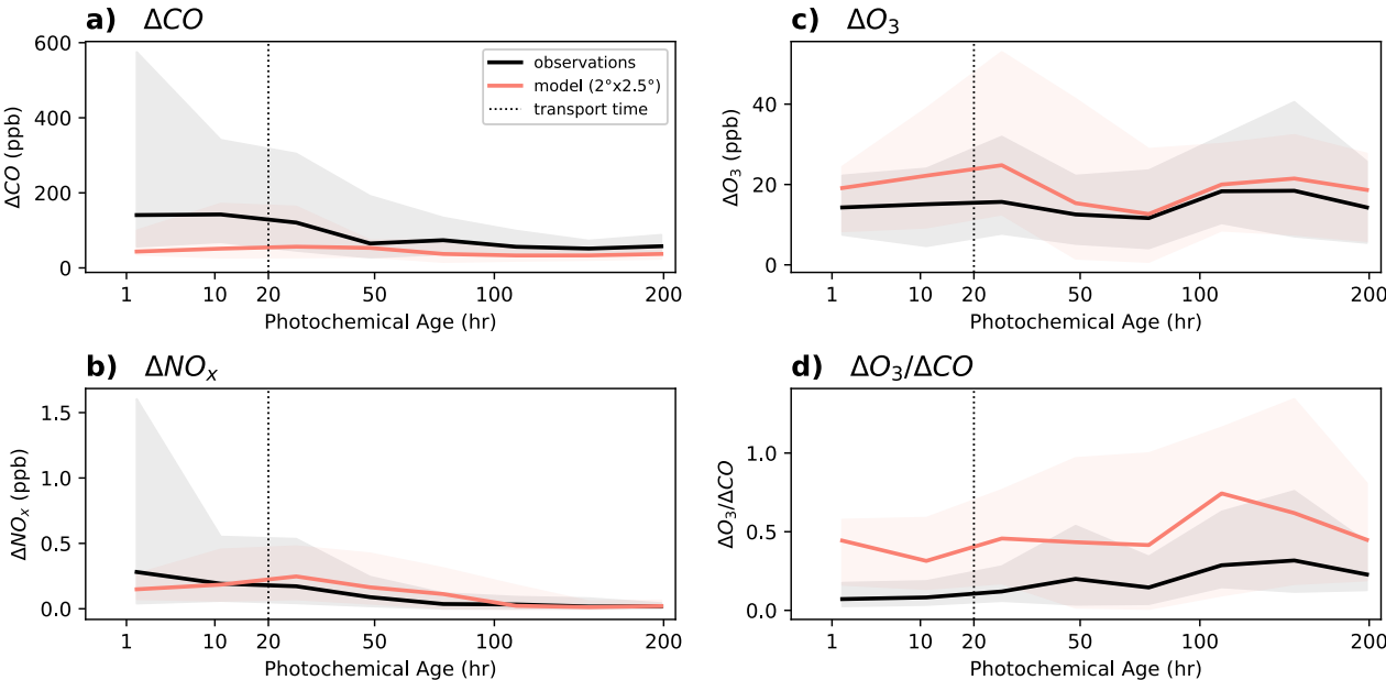
425 Figure 8. Comparison between GEOS-Chem simulated (red) and fire-influenced observations (black), plotted over observationally 430 derived photochemical ages, binned in log-space. The lines represent the median, and the shaded area extends from the 16th to the 435 84th percentile (corresponding to one standard deviation, in outlier resistant percentile space) within each bin. The dashed line represents the approximate transport time for a 2x2.5 grid box at mid-latitudes.
