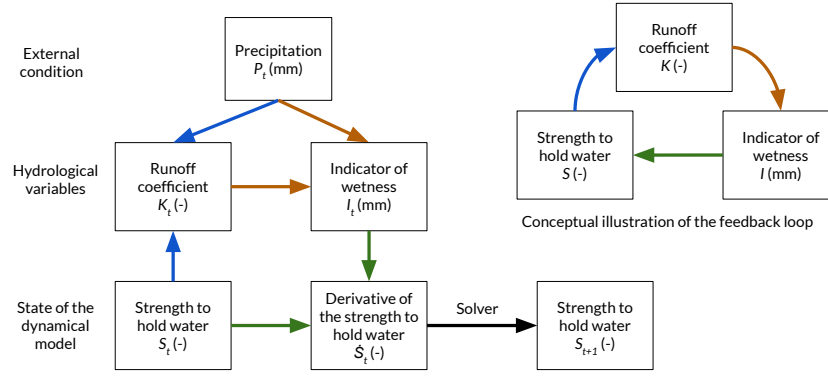
Figure 3. At every time t , the derivative of the water holding strength \dot{S}_t is computed in three steps: i) the runoff coefficient K_t is derived from the water holding strength S_t and the precipitation P_t (Eq. 1), ii) the indicator of wetness I_t is determined by the runoff coefficient K_t and the precipitation P_t (Eq. 2), iii) the derivative \dot{S}_t is calculated with the water holding strength S_t and the indicator of wetness I_t (Eq. 3).
