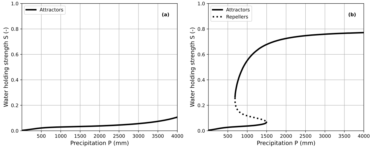
Figure 4. Bifurcation diagram of a (a) monostable (b) bistable parameterization \theta for precipitation P between 1 mm and 4000 mm.
