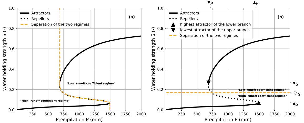
Figure 5. Bifurcation diagram of a bistable parameterization \theta for precipitation P between 1 mm and 2000 mm (for readability). We illustrate (a) regimes based on attraction basin (b) regimes based on a threshold \diamond_S , where \diamond_S equals the mean of \blacktriangle_S and \nabla_S .
