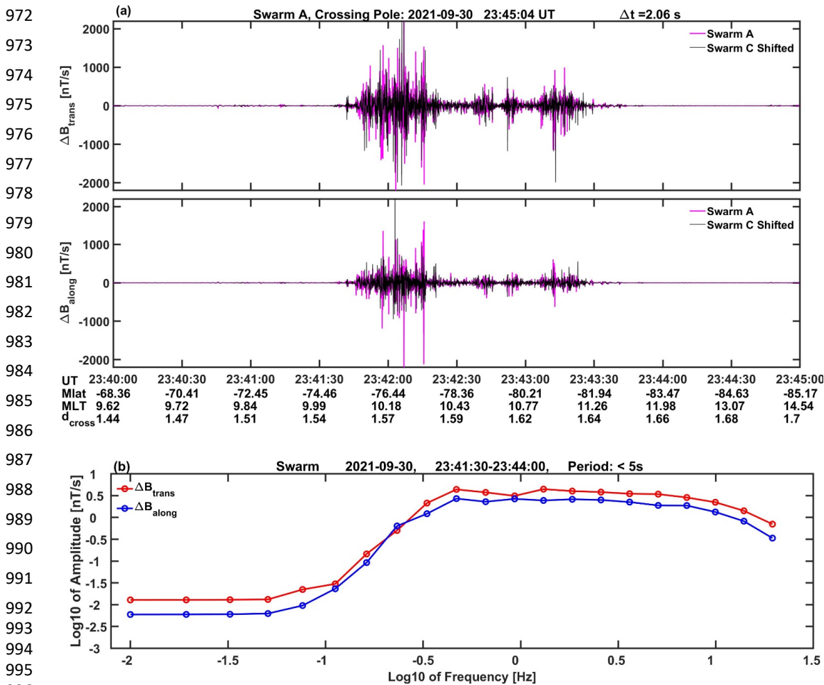
Figure 9. Example of signal spectra for a typical burst of km-scale FAC activity, separately for the field components \Delta B_{trans} and \Delta B_{along} . The steep amplitude roll-off around 0.2 Hz is caused by the applied high-pass filter.
