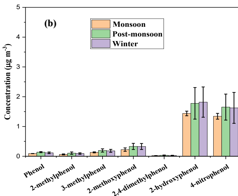
Fig.3: Variation of concentration of phenolic compounds in (a) Dhaka, South and (b) Dhaka North site during monsoon, post-monsoon and winter.
