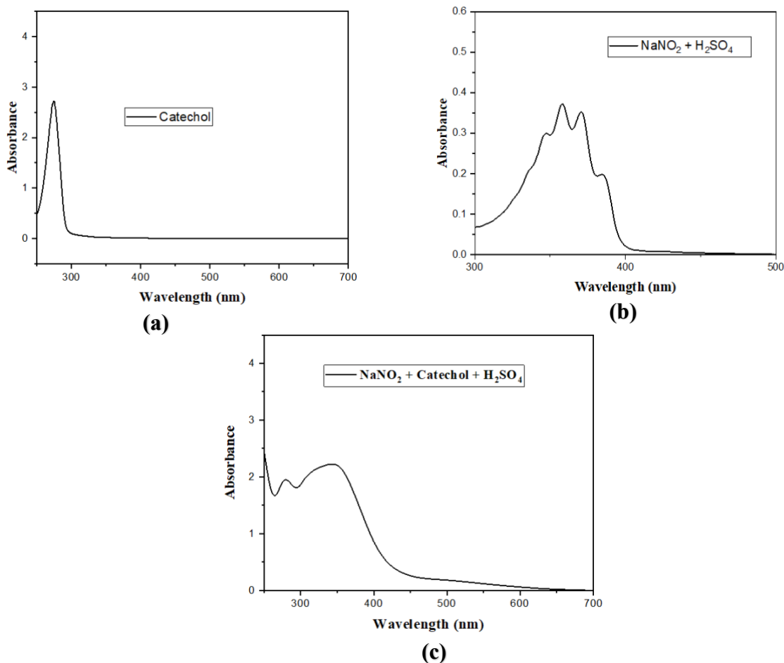
Fig.4: Absorbance of (a) single catechol, \lambda_{\text{max}}=275 nm, (b) \text{NaNO}_2 + \text{H}_2\text{SO}_4 , and (c) reaction system (catechol-nitrite)
