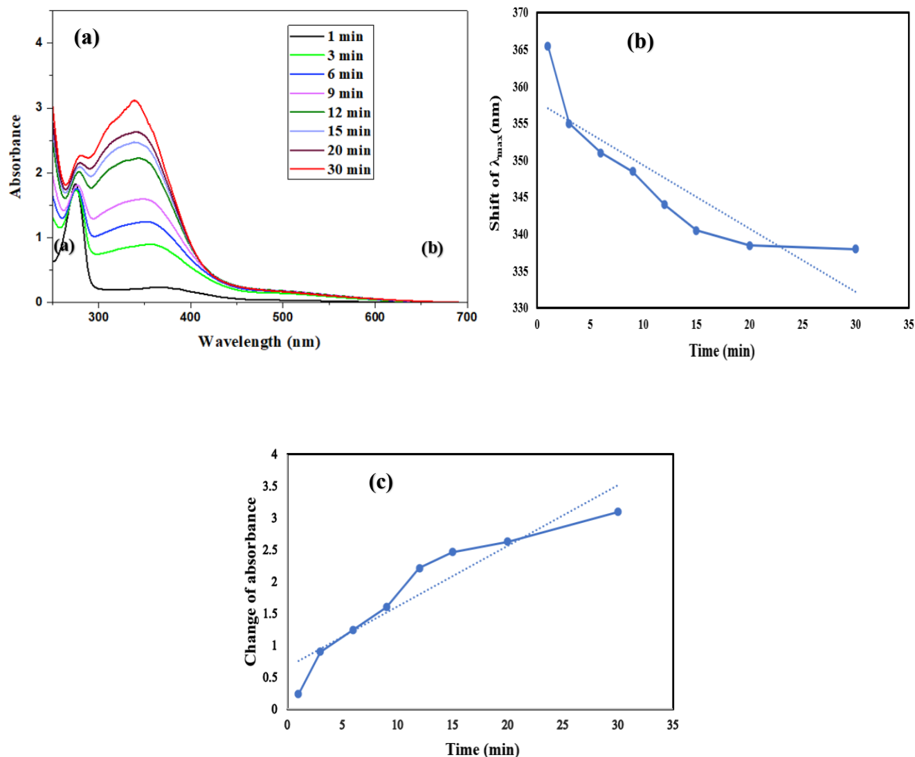
Fig.5: (a) Change of the absorbance with times of the reaction system containing 1 mM 2-hydroxyphenol and 1 mM NaNO 2 at pH=3.5. A distinct color denotes the duration of the sample run in the ultraviolet-visible spectrophotometer. The initial reactant contribution was subtracted from each spectrum. (b) Shift of \lambda_{\max} with time, and (c) Change of absorbance with time.
