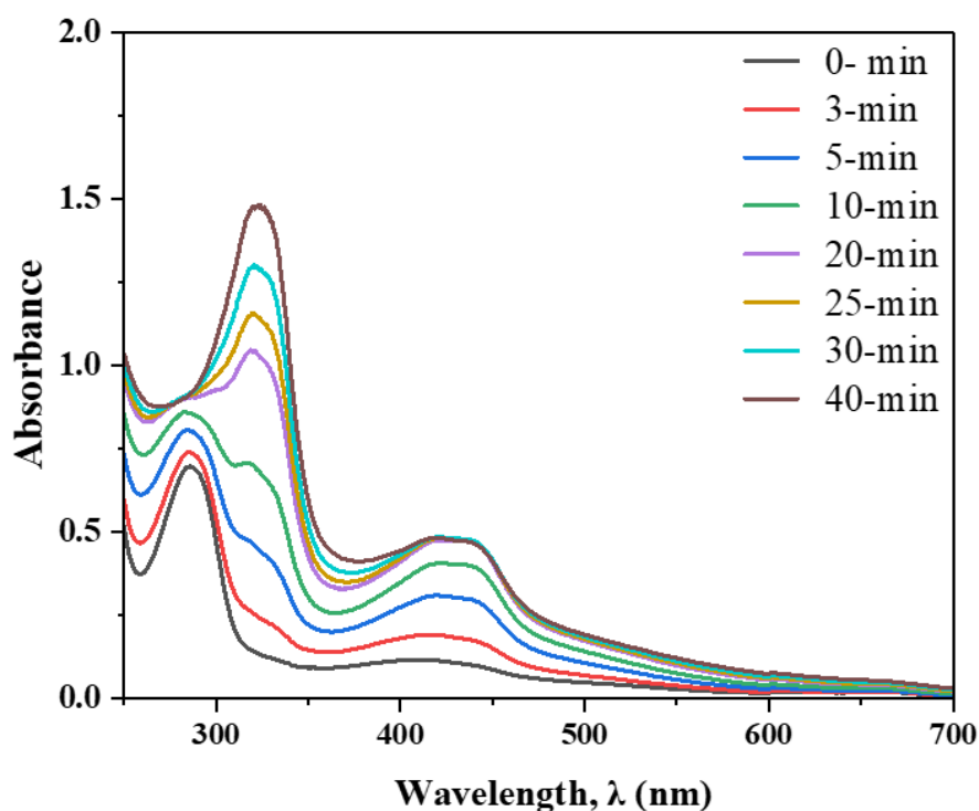
433 434 Fig. 6: UV-visible absorption spectra of the nitrite-catechol reaction system in alkaline medium, pH~7-8 435 to form a light-absorbing nitro aromatic compound.
