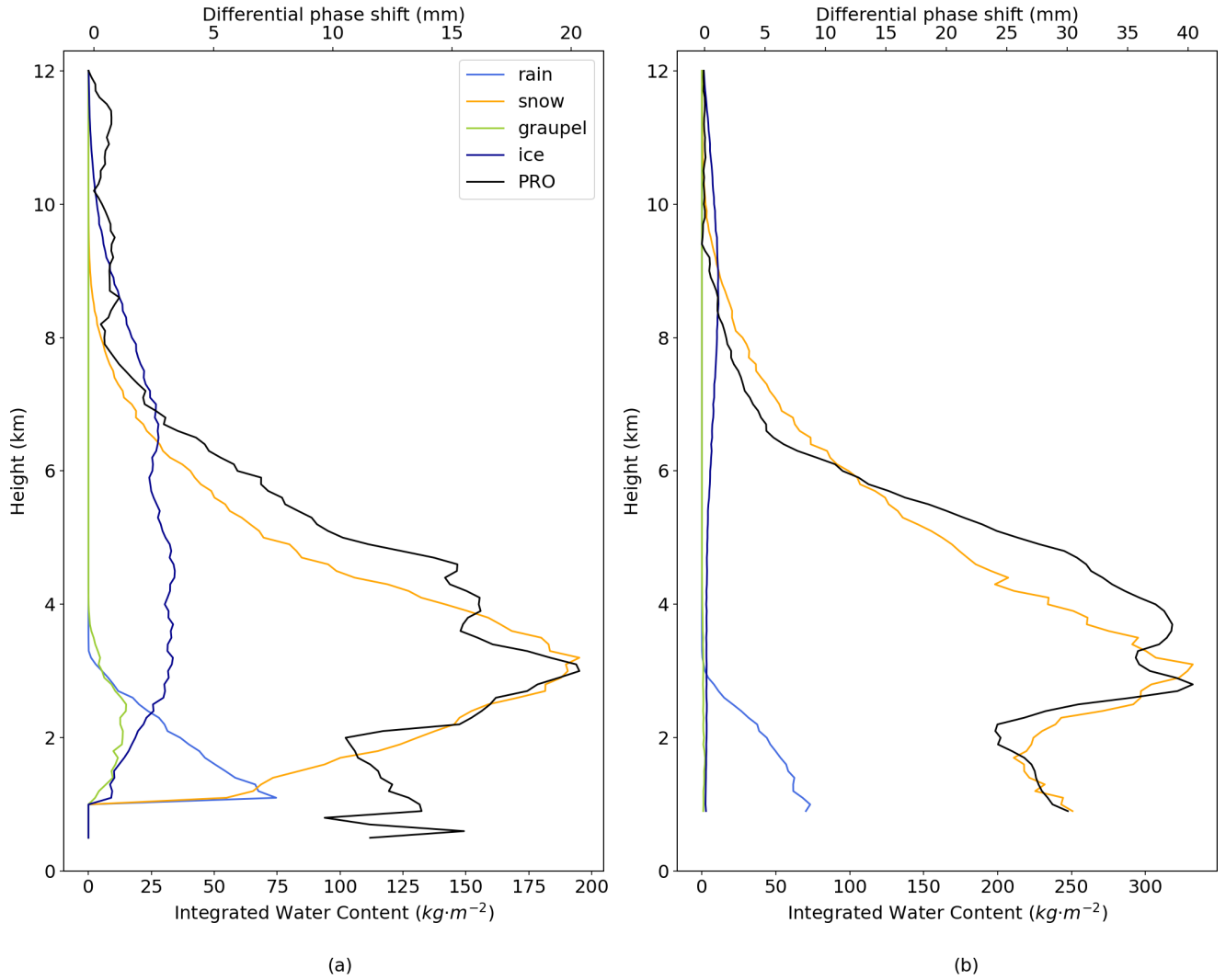
Figure 8. Vertical profiles of the differential phase shift (top x-axis) obtained from PAZ and the integrated water content (bottom x-axis) from WRF for the different hydrometeors. The microphysics schemes used were Goddard (a) for the observation with roid PAZ1.2019.142.10.32.G02 and Morrison (b) for the observation with roid PAZ1.2023.038.10.59.G19 scheme.
