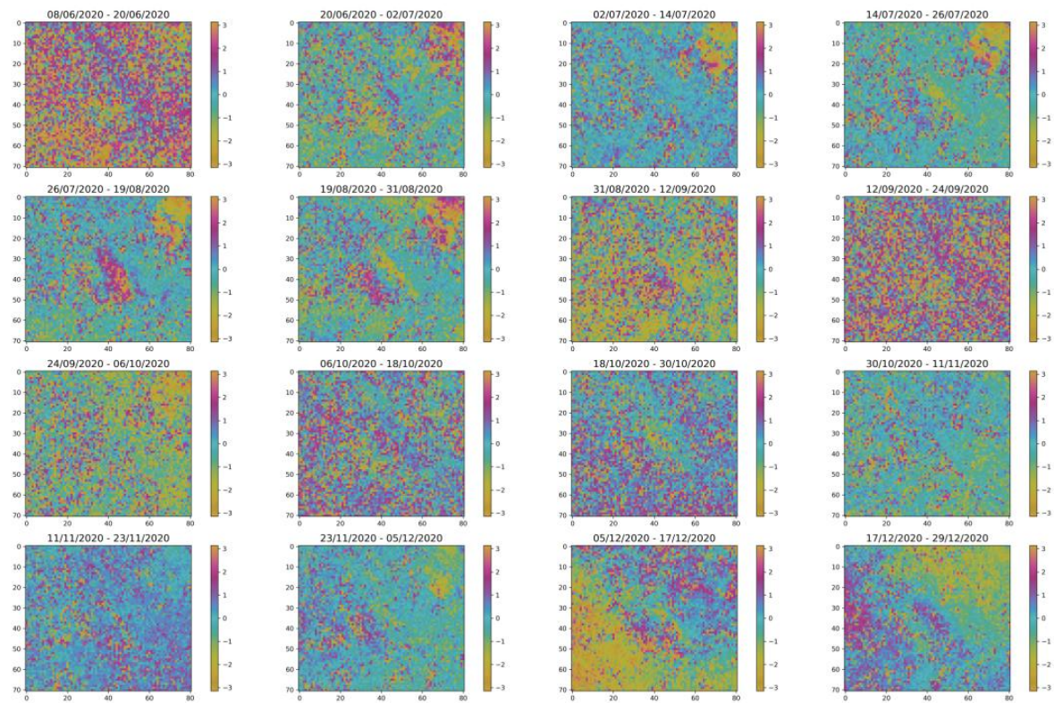
Supplementary Figure 8. Corrected wrapped interferograms from 08/06/2020 to 29/12/2020.
