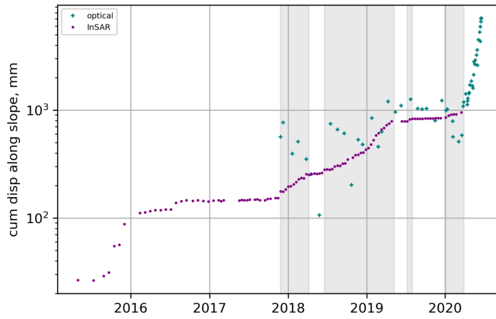
Supplementary Figure 9. Semilog plot of cumulative displacements on the Achoma landslide, showing the complementarity of InSAR and optical image correlation.
