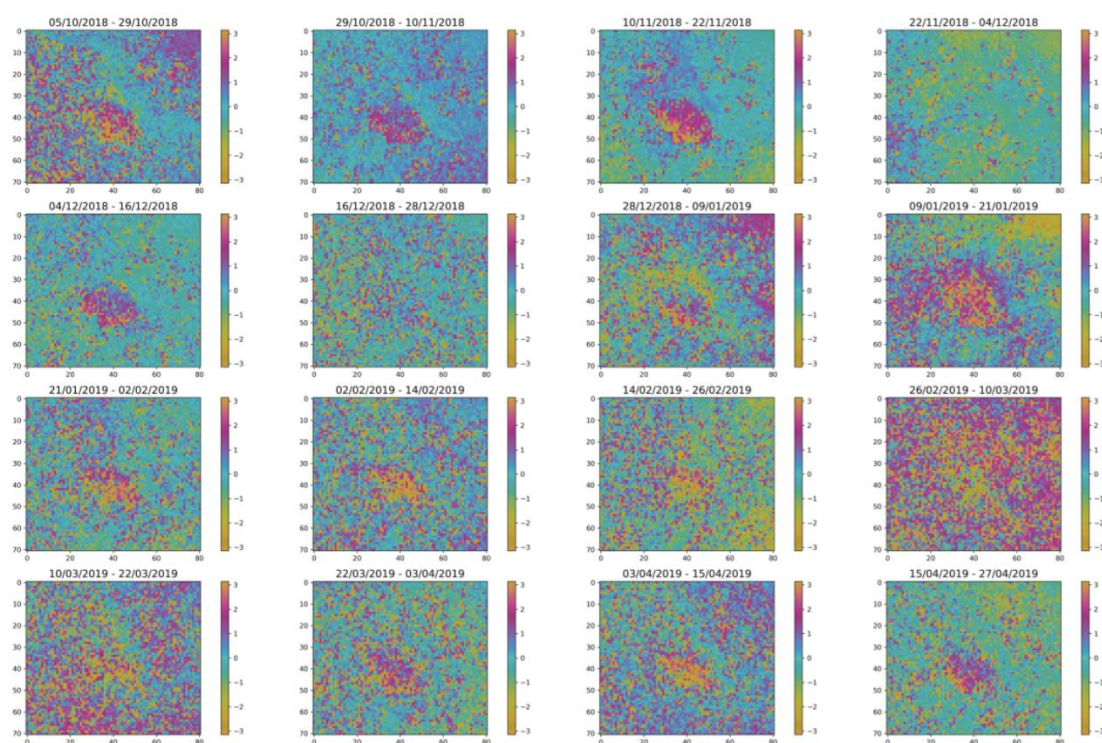
Supplementary Figure 5. Corrected wrapped interferograms from 05/10/2018 to 27/04/2019.
