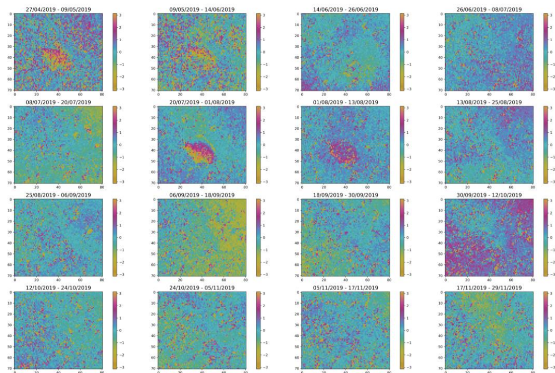
Supplementary Figure 6. Corrected wrapped interferograms from 27/04/2019 to 17/11/2019.
