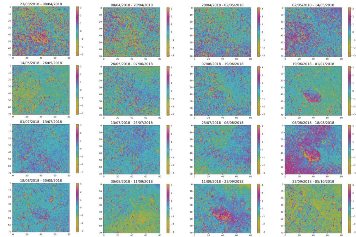
Supplementary Figure 4. Corrected wrapped interferograms from 27/03/2018 to 05/10/2018.
