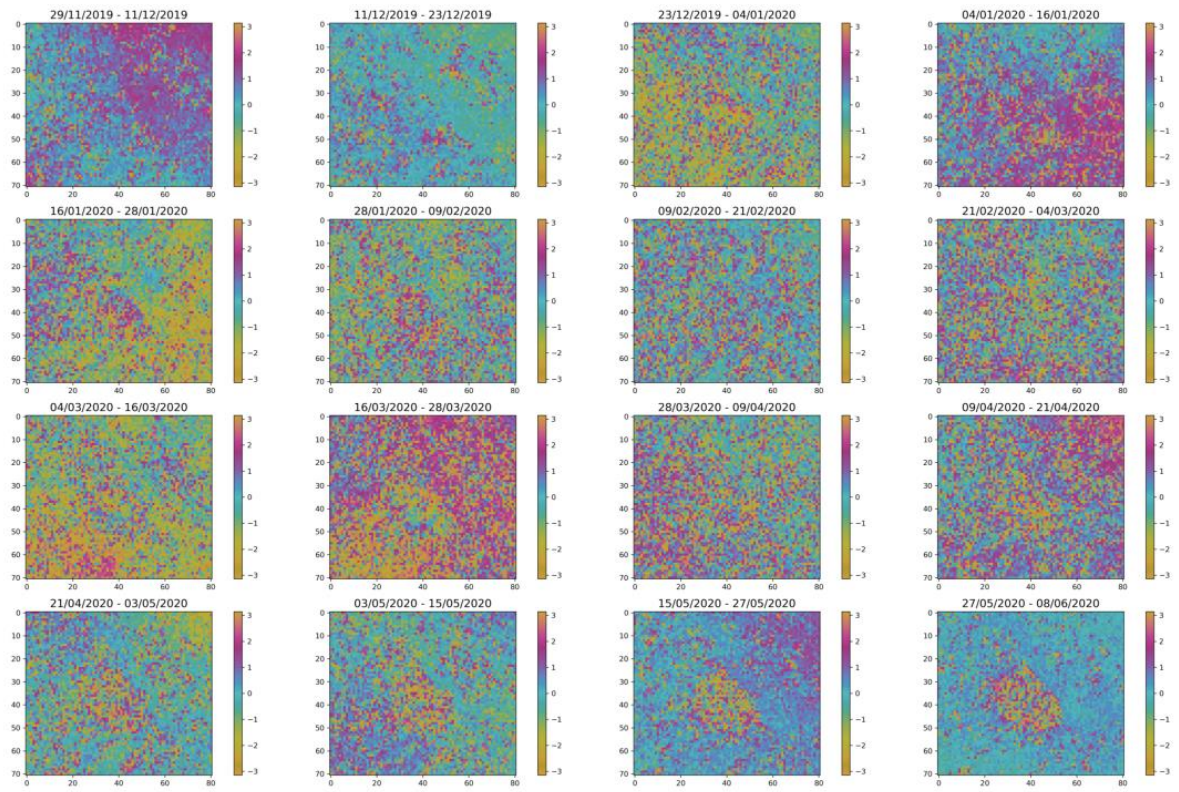
Supplementary Figure 7. Corrected wrapped interferograms from 29/11/2019 to 08/06/2020.
