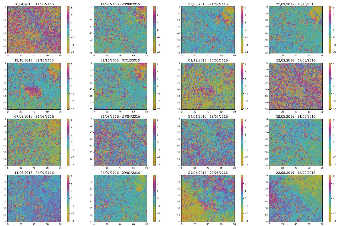
Supplementary Figure 1. Corrected wrapped interferograms from 30/04/2015 to 15/09/2016.
