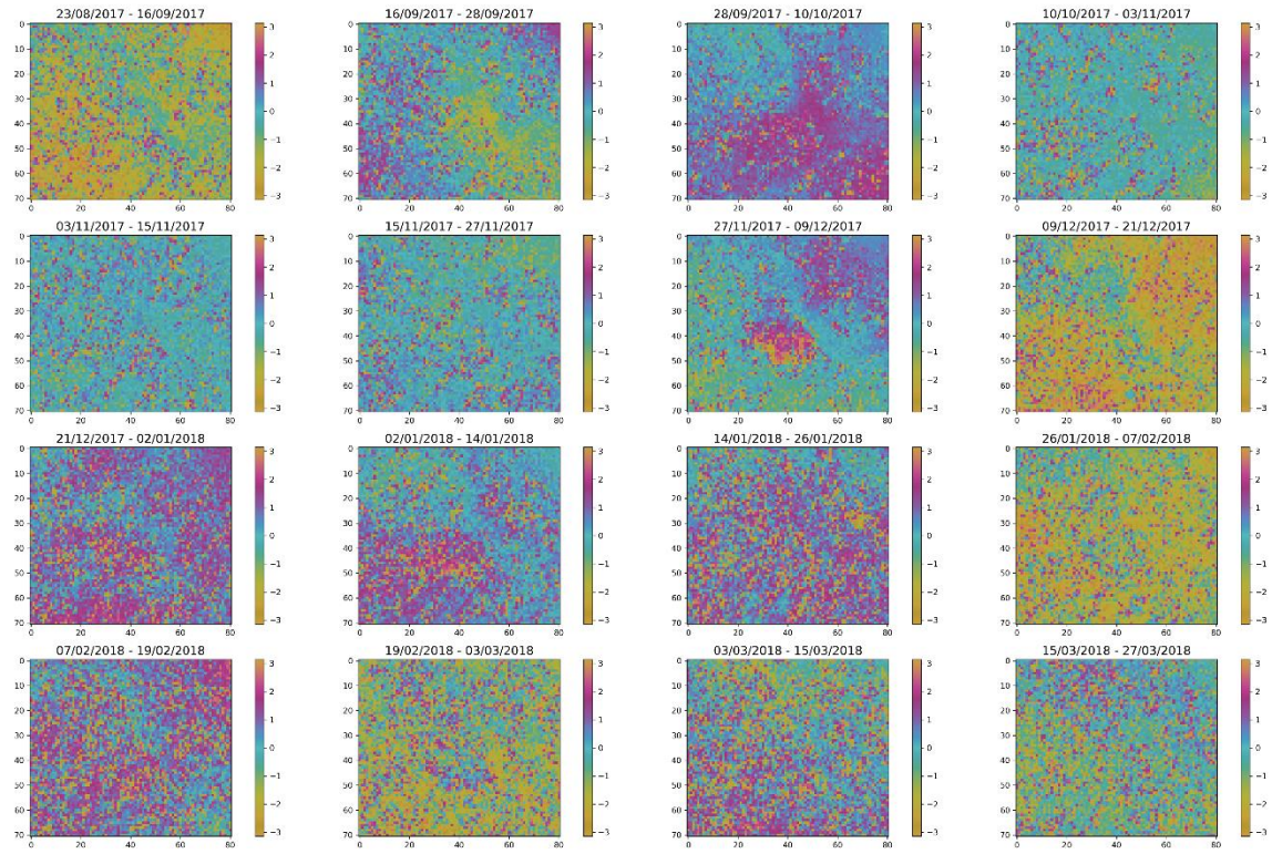
Supplementary Figure 3. Corrected wrapped interferograms from 23/08/2017 to 27/03/2018.
