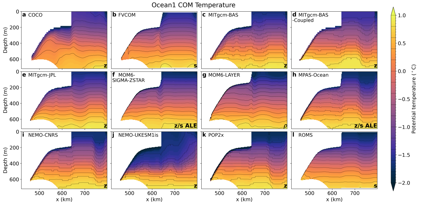
Figure 2. Spin-up (average of year 20) temperature transect along y = 40 km in the Ocean1 COM experiment. Model vertical coordinates are labelled in the lower right corner, with z for z -coordinate models, s for terrain-following, \rho for isopycnal, and z/s ALE for Arbitrary Lagrangian-Eulerian coordinates with a quasi z -ice shelf-following target coordinate (Table 2). Contours are spaced by 0.2^\circ\text{C} .
