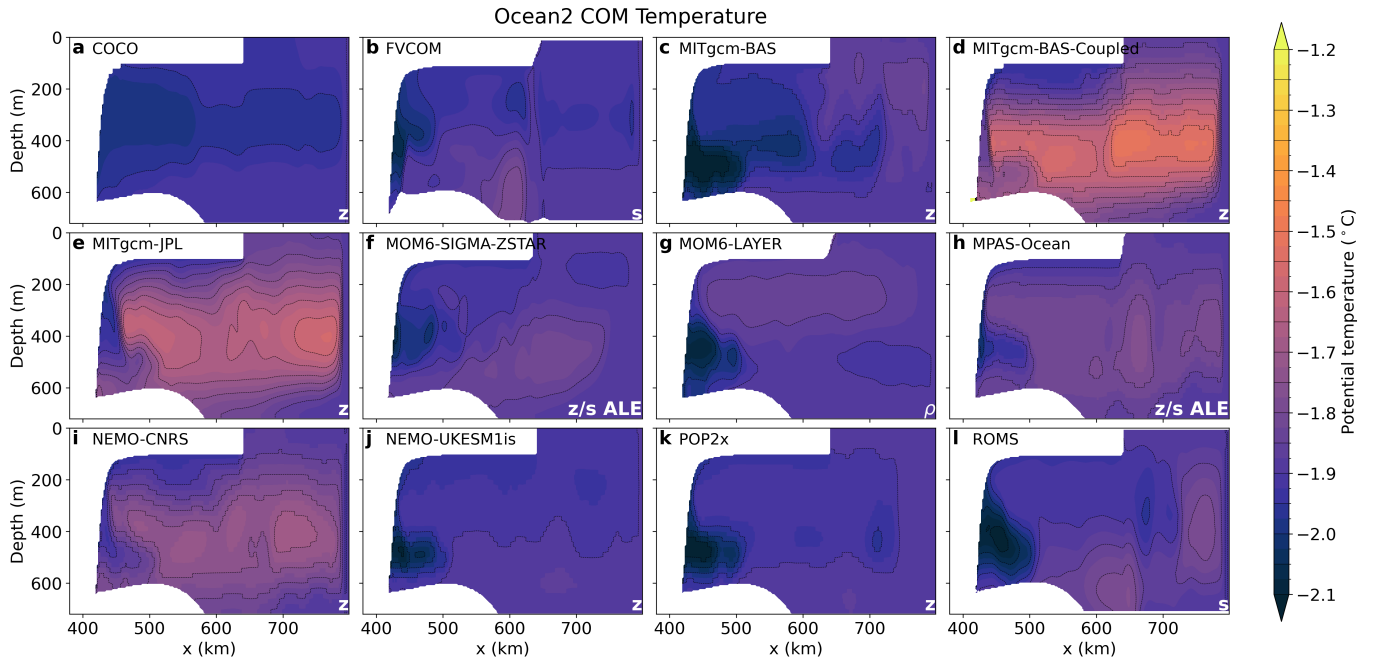
Figure 3. Spin-up (average of year 20) temperature transect along y = 40 km in the Ocean2 COM experiment. Model vertical coordinates are labelled in the lower right corner, as in Fig. 2. Contours are spaced by 0.05^\circ\text{C} . Note the different colourbar to Fig. 2.
