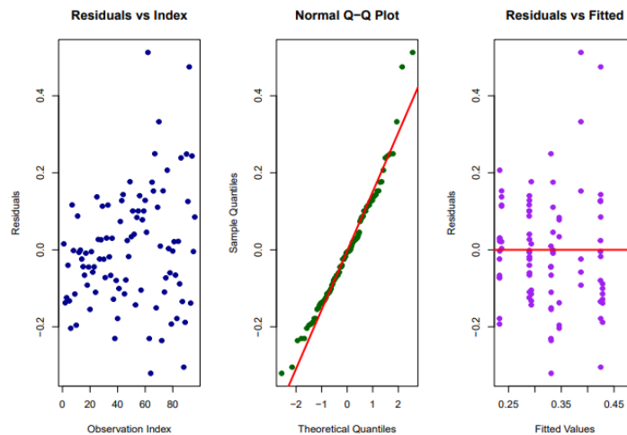
Fig 1: Residual plots for cumulative N 2 O emissions
