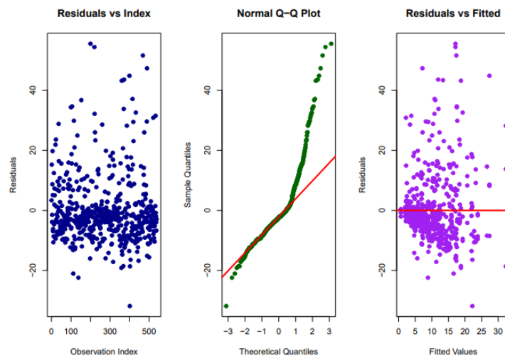
Fig 2: Hourly N 2 O fluxes
