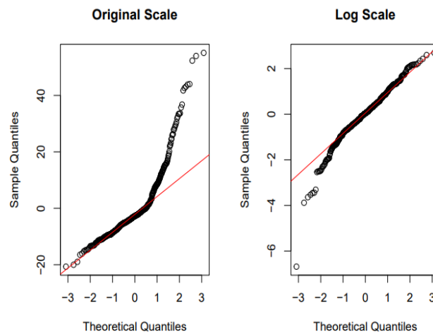
Fig 3: Q-Q plots comparing non-transformed and log transformed hourly N 2 O fluxes
