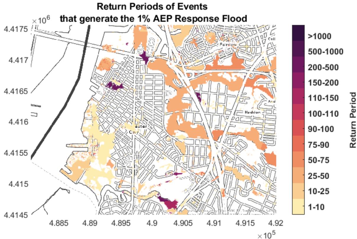
390 Figure 8. Return periods (based on the bivariate extreme model) of the events that generate the 100-year water depth from the response approach. [NAD83/UTM18N. ©Esri]
