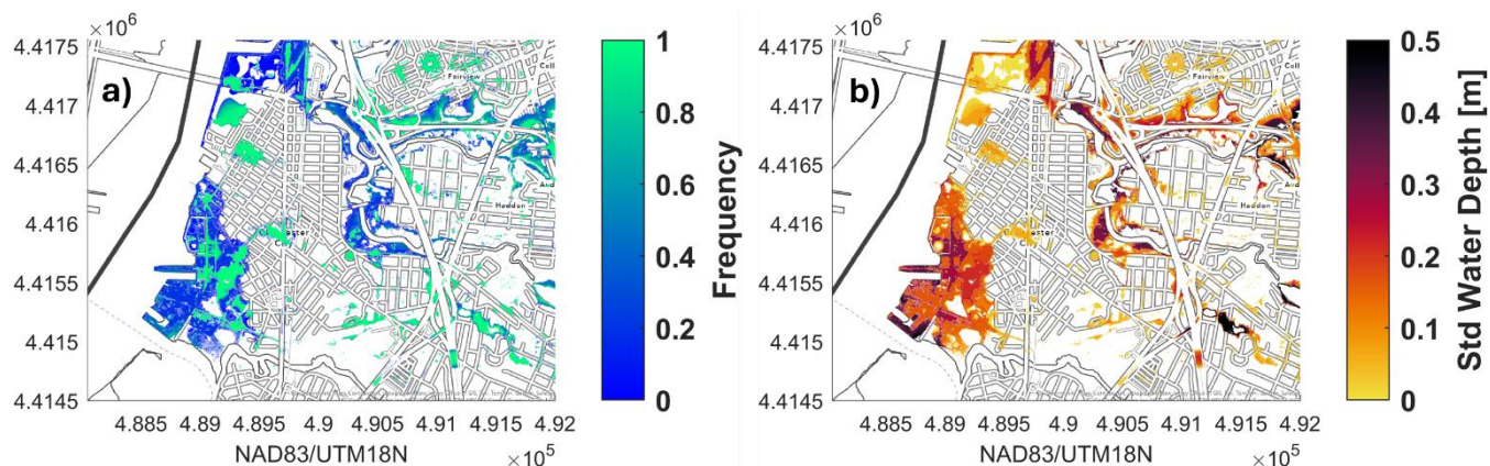
305 Figure 4 a) Frequency of flooding at each model cell (1m 2 ) from the 25 events selected along the 100-year (1% AEP) isoline. b) The standard deviation of water depth (m) at each model cell (1m 2 ) between the 25 events selected along the 100-year (1% AEP) isoline. [NAD83/UTM18N. ©Esri]
