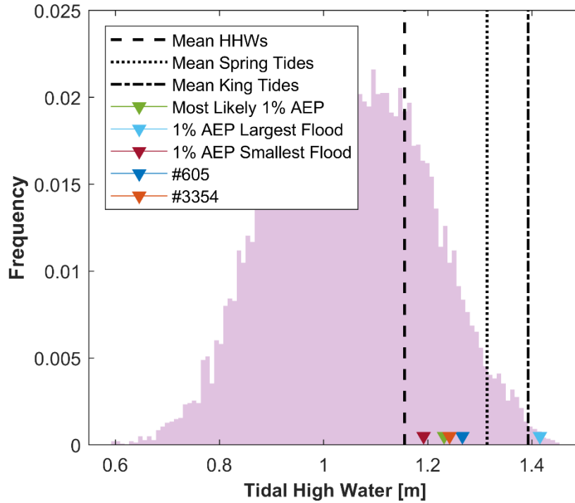
230 Figure 3 Histogram of tidal high water levels over the last 19 year period from 2003 to 2021. Black lines show the tidal levels of MHHW, Mean Spring Tide, and Mean King Tide (defined as the largest annual tide). Coloured lines show as an example the largest high tide levels of the tidal curves selected for the synthetic events shown in Fig. 2b-d, and two additional synthetic events (#605 and #3354) discussed in the results section. Tidal levels are referenced to NAV 88 datum.
