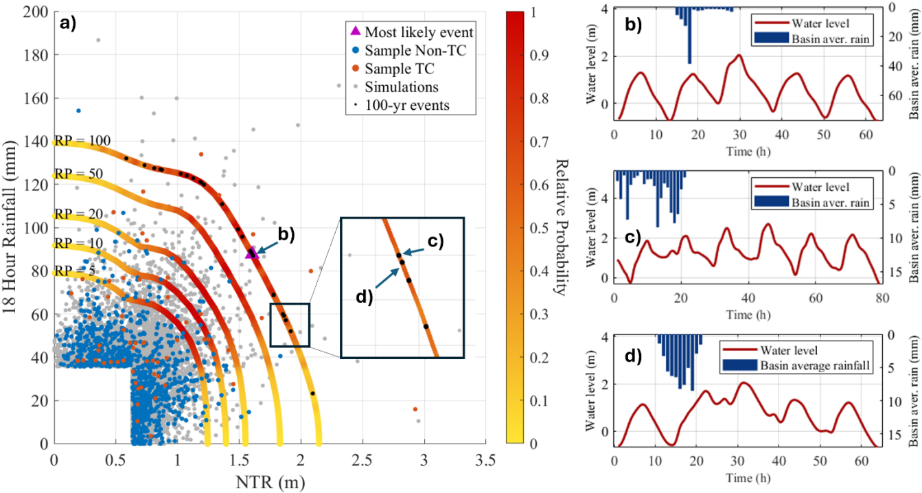
Figure 2. a) Joint probabilities of non-tidal residual (NTR) and 18hr rainfall accumulation. Blue dots show the historical non-tropical cyclone events, red dots show the historical tropical cyclone events, and grey dots the 5,000 synthetic events generated for this study. All synthetic events (grey points) have assigned water level hydrographs and rainfall fields to be used as boundary conditions for SFINCS. b) c) and d) show as an example the time series of three 1% AEP (100-year) events (black dots along the 100-year isoline); b) shows the time series of the “most likely” event, marked as a purple triangle in a); c) shows the 1% AEP (100-year) event that produces the largest flood from all 1% AEP (100-year) events (black dots in a); and d) shows the 1% AEP (100-year) event that produces the smallest flood from all 1% AEP (100-year) events. Water levels are referenced to NAVD88.
