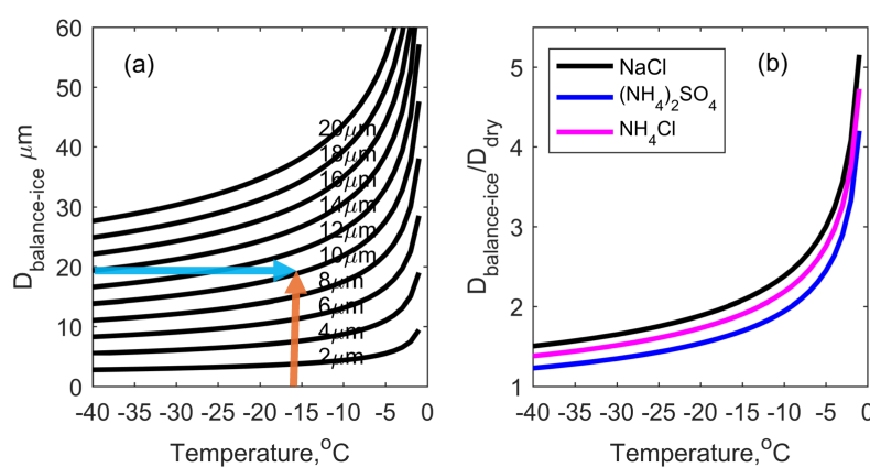
Figure 2. (a) The relationship between the diameter of dry salt particles (NaCl) and the corresponding balanced diameter of droplets. Each black line represents the diameter of the dry salt particles; (b) Ratio of droplet diameter in equilibrium state to dry aerosol diameter for different aerosol compositions.
