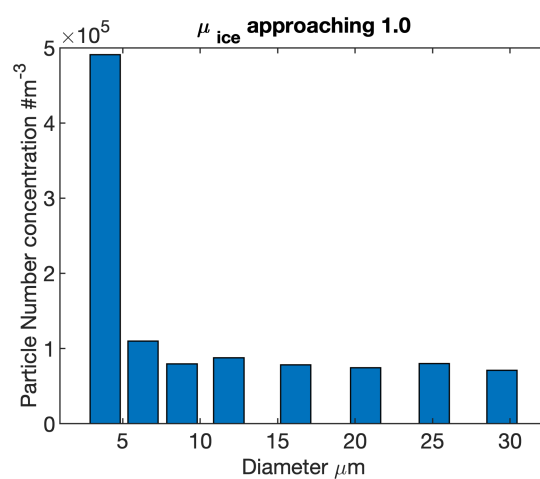
Figure 7. The particle number concentration of each bin from AFLUX campaign in-situ measurement when the ice phase fraction coefficient, \mu_{ice} , approaches 1.0.
