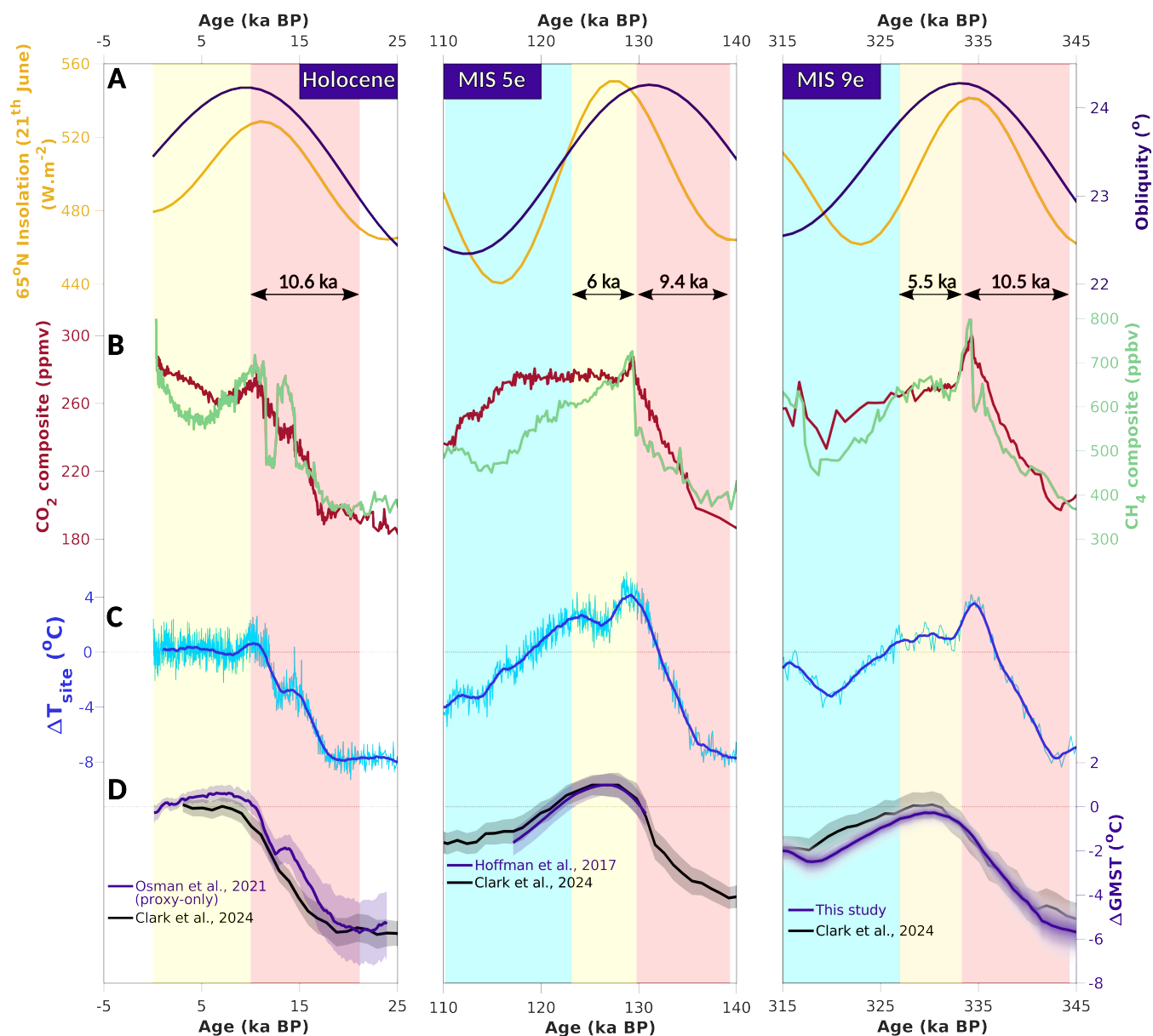
575 Figure 6: Comparison of our new MIS 9 synthesis to the Holocene and MIS 5e ones. A) 65°N summer solstice insolation (light orange, Laskar et al., 2004) and obliquity (dark purple, Berger & Loutre, 1991) variations; B) composite CO 2 (brown; Bereiter et al., 2015; Nehrbass-Ahles et al., 2022) and CH 4 (green, Louergue et al., 2008) atmospheric concentrations; C) anomaly of Antarctic surface air temperature (light blue; Landais et al., 2021) and 2-ka moving average (blue); most recent GMST for the Holocene and T-I (Osman et al., 2021; Clark et al., 2024), the MIS 5e (Hoffman et al., 2017; Clark et al., 2024) and MIS 9e (this study; Clark et al., 2024). Note that CO 2 , CH 4 and ΔT site are plotted on the AICC2023 chronology (Bouchet et al., 2023). We rescale the global SST from Hoffman et al. (2017) on AICC2023 and convert it into GMST by applying the same procedure as in this study. The Osman et al. (2021) stack refers as the “data-only” rather than the estimations data-assimilated into climate model simulations. Red vertical bands are related to deglacial warming periods, yellow vertical bands to the climatic optima (visually defined) and blue vertical bands to glacial inceptions. 580
