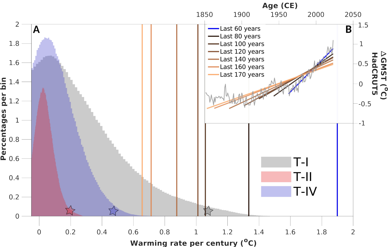
Figure 7: Percentages of rate of warming over termination I, II and IV. A) Percentages per bin of warming rate per century for the T-I, T-II and T-IV; B) the HadCRUT5 (Morice et al., 2021) temperature curve, representative of the most recent (1850 to 2023 years CE) GMST. These rates were obtained using the first derivative with 10^5 iterations, which randomly drawn the GMST values within the 2\sigma uncertainty for each time-bin. Periods involved for the terminations are 20 to 10 ka (T-I, grey), 140 to 125 ka (T-II, orange) and 346 to 333.5 ka (T-IV, blue). Coloured stars represent the 99 th percentile observed for each deglaciation. We calculate the warming trend, from the last 170 to the last 60 years (20 years step). Then, after a conversion in °C per century, we report these trends in the principal panel (vertical bands) for a comparison to those obtained for the three terminations.
