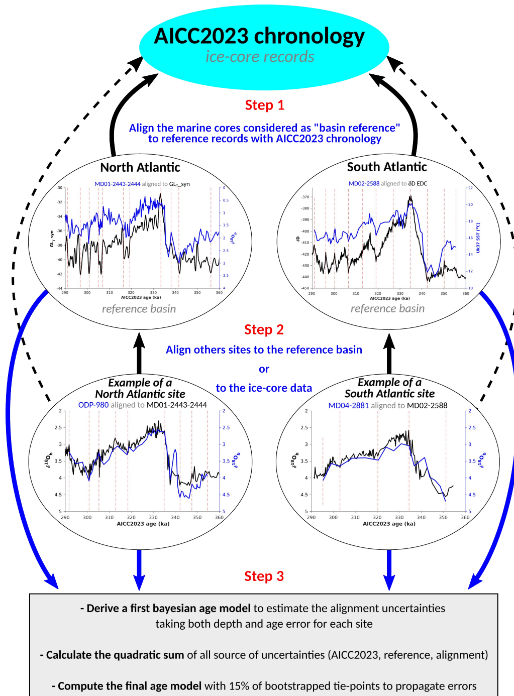
240 Figure 2: Description and examples of the chronology construction. In step 1 and 2, the blue curve is the record used to align to the reference (black curve). Dashed vertical lines in “Step 1” and “Step 2” represent the tie points used to align the record to the reference. For the North Atlantic example, the \delta^{18}O_p from core MD01-2443-2444 (Martrat et al., 2007) is aligned to the GL_T_{syn} (Barker et al., 2011), and the \delta^{18}O_p record from ODP-980 (McManus et al., 1999) is align to the MD01-2443-2444 one with the revised age scale.
