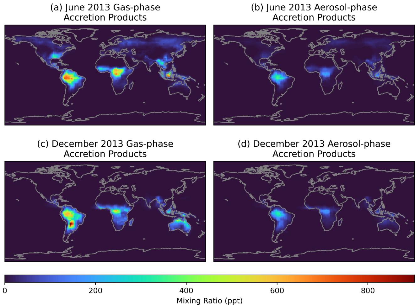
350 Figure 4. Monthly average ground-level gas (a,c), and aerosol-phase (b,d) mixing ratios simulated by GEOS-Chem with added RO 2 accretion reactions in June (a,b) and December (c,d) 2013.
