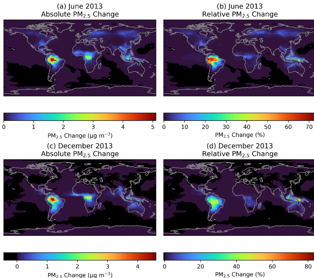
375 Figure 5. The change in monthly average ground-level PM 2.5 concentrations when adding RO 2 accretion reactions to GEOS-Chem. (a) and (c) show the absolute change in ground-level PM 2.5 mass concentration in June and December, respectively. (b) and (d) show the change as a percentage of ground-level PM 2.5 in the base model in June and December, respectively.
