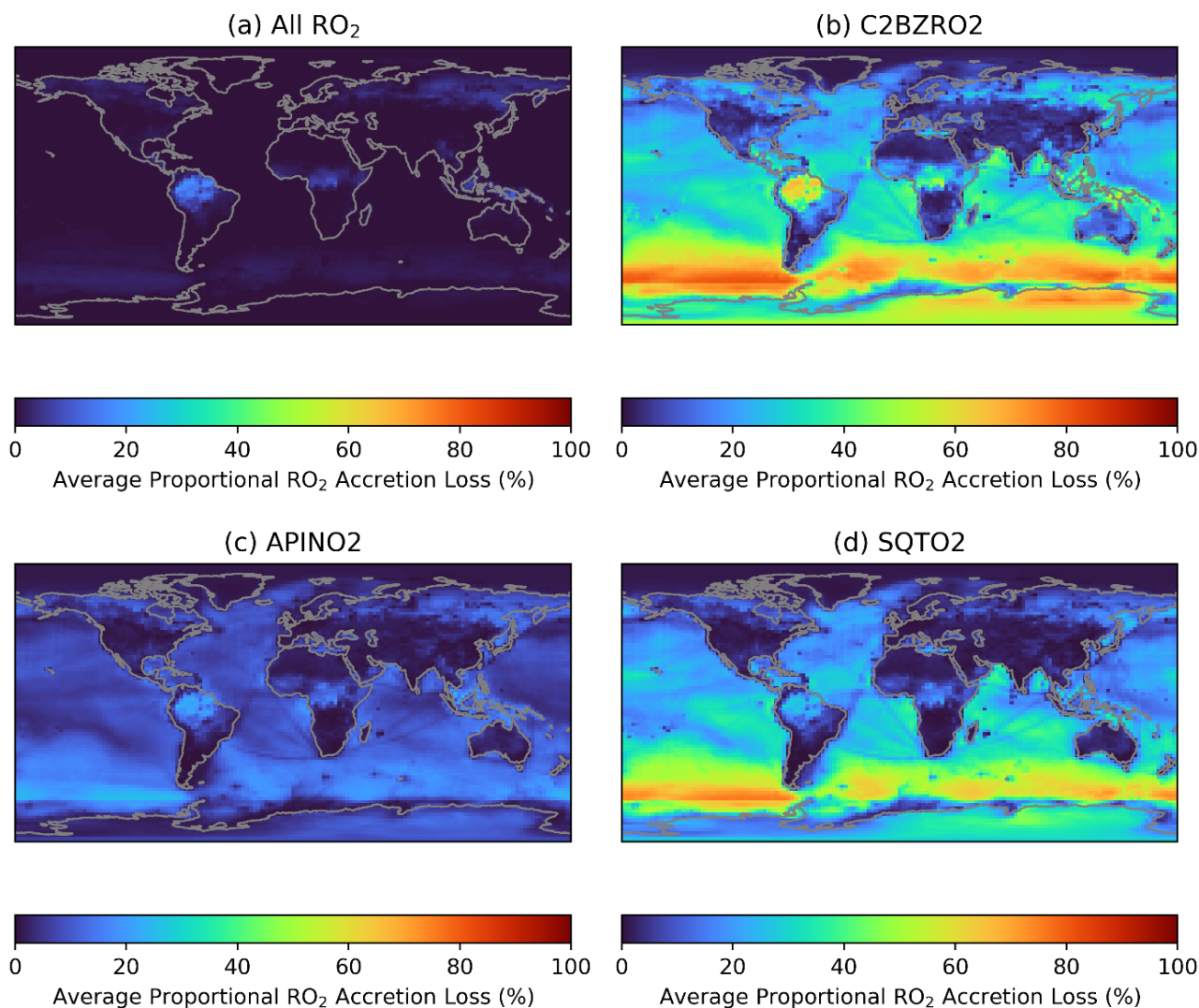
480 Figure 9. Proportional loss of RO 2 to accretion reactions, independent of RO 2 concentration, during June of the GEOS-Chem simulation. (a) average for all RO 2 , (b) primary RO 2 from styrene oxidation (C2BZRO2), (c) primary \alpha -pinene RO 2 (APINO2), (d) primary sesquiterpene RO 2 (SQTO2).
