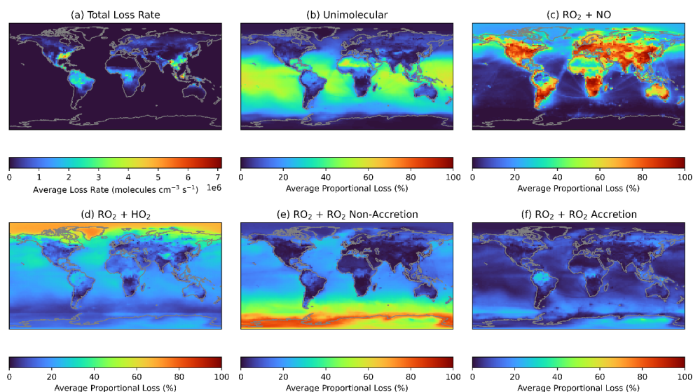
Figure 8. (a) Average total loss rate of the primary isoprene RO 2 , IHOO1, during June of the GEOS-Chem simulation. (b-f) Average fractional loss of IHOO1 to each loss pathway, independent of RO 2 concentration.
