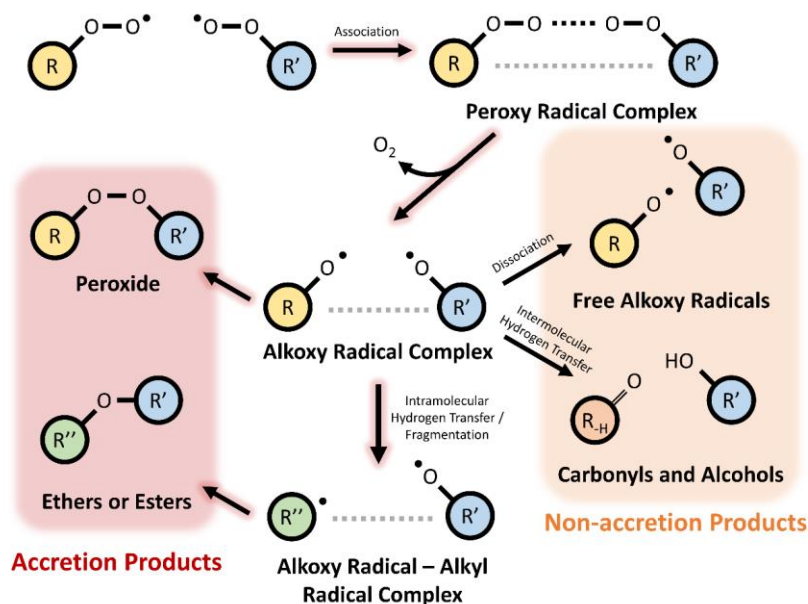
85 Figure 1. Schematic showing the formation of peroxide, ether, and ester RO 2 accretion products via intermediate complexes of peroxy and alkoxy radicals.
