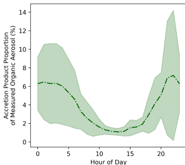
385 Figure 6. Proportion of measured organic aerosol estimated to be comprised of accretion products in the MCM-Accr SOAS box model simulations, calculated by taking the ratio of the modelled accretion product concentration and the AMS measured OA. Lines represent the hourly mean mixing ratio and shaded areas show one standard deviation above and below the mean.
