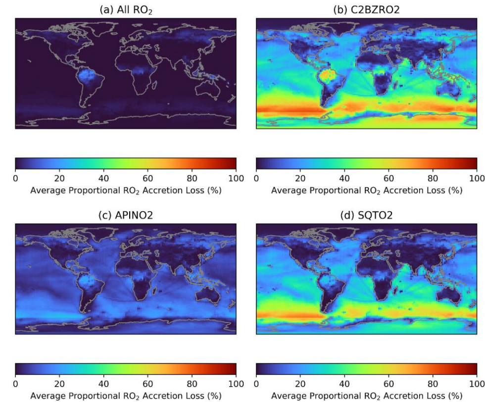
Figure 9. Proportional loss of RO 2 to accretion reactions, independent of RO 2 concentration, during June of the GEOS-Chem simulation. (a) average for all RO 2 , (b) primary RO 2 from styrene oxidation (C2BZRO2), (c) primary \alpha -pinene RO 2 (APINO2), (d) primary sesquiterpene RO 2 (SQTO2).
