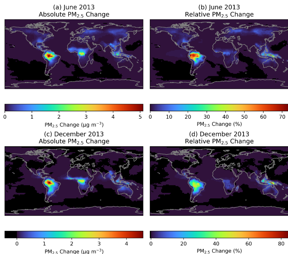
Figure 5. The change in monthly average ground-level PM 2.5 concentrations when adding RO 2 accretion reactions to GEOS-Chem. (a) and (c) show the absolute change in ground-level PM 2.5 mass concentration in June and December, respectively. (b) and (d) show the change as a percentage of ground-level PM 2.5 in the base model in June and December, respectively.
