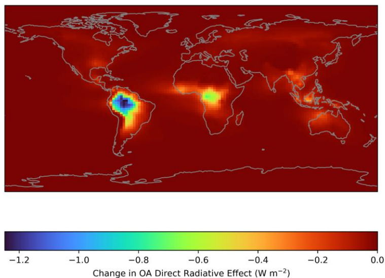
Figure 13. Calculated difference in annual average Direct Radiative Effect (DRE) when RO 2 accretion reactions are included and excluded from the GEOS-Chem simulations.
